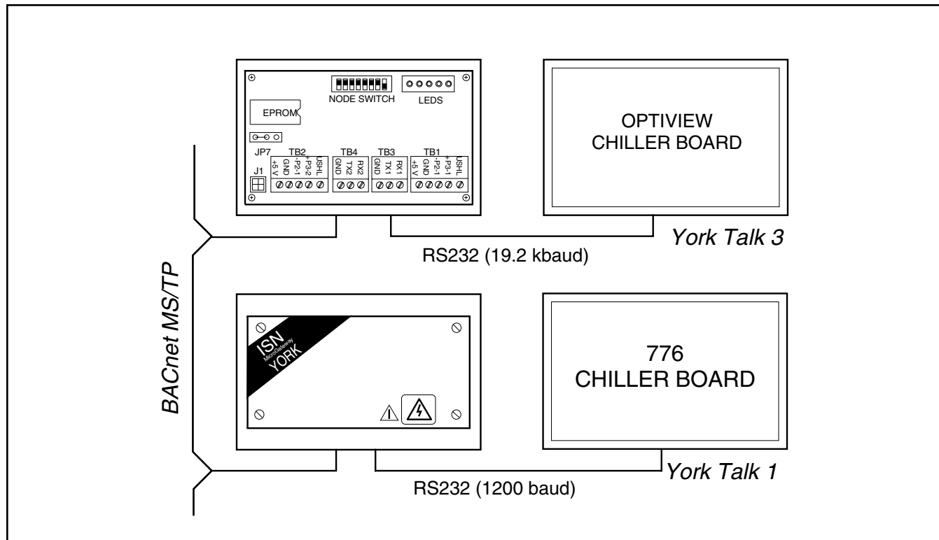
Figure 2. Typical Board Topology
