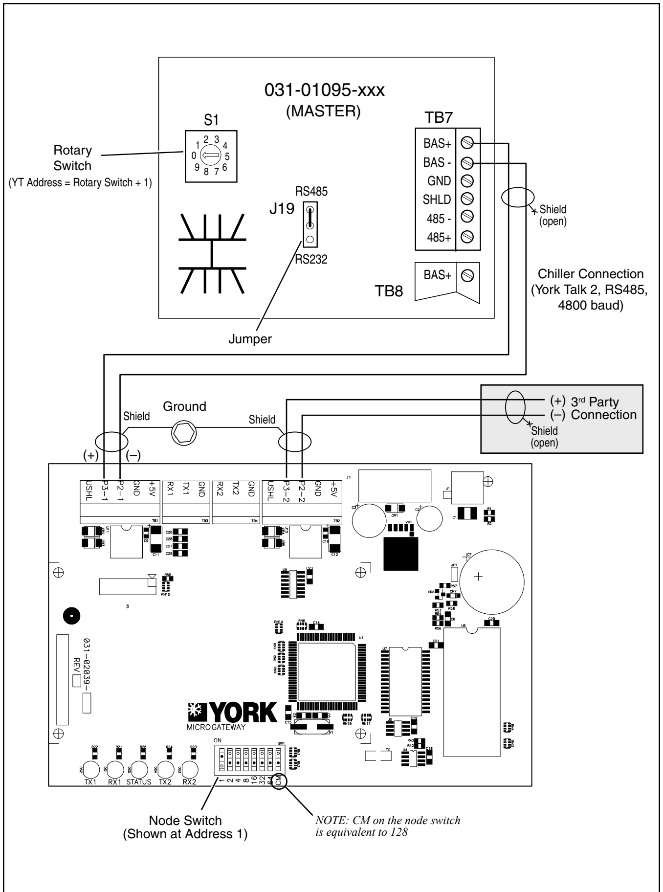
Figure 14. 1095 Master Board Connections
