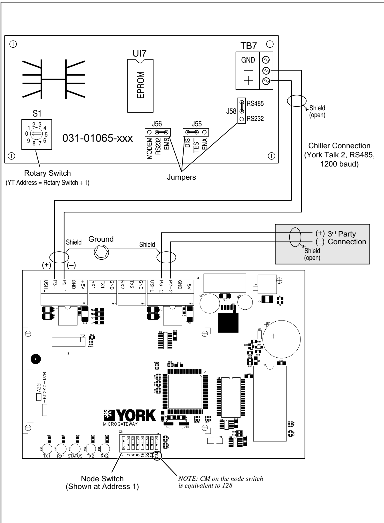
Figure 13. 1065 Board Connections
