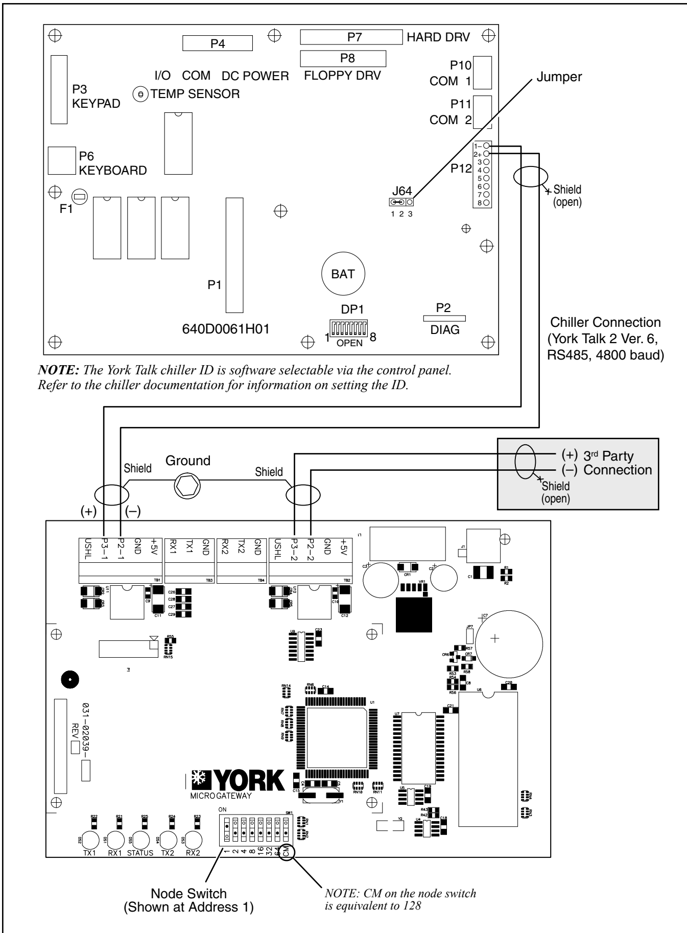
Figure 19. Frick Quantum 1 and 2 Board Connections
