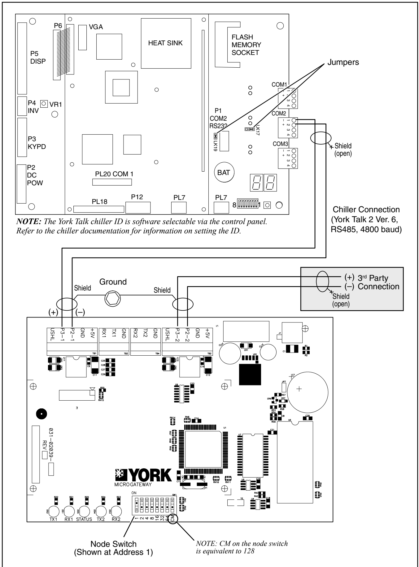
Figure 20. Frick Quantum 3 Board Connections
