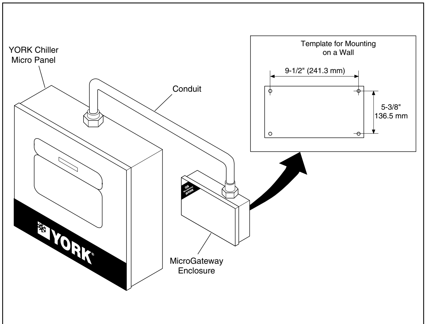
Figure 9. Wall Mounting
