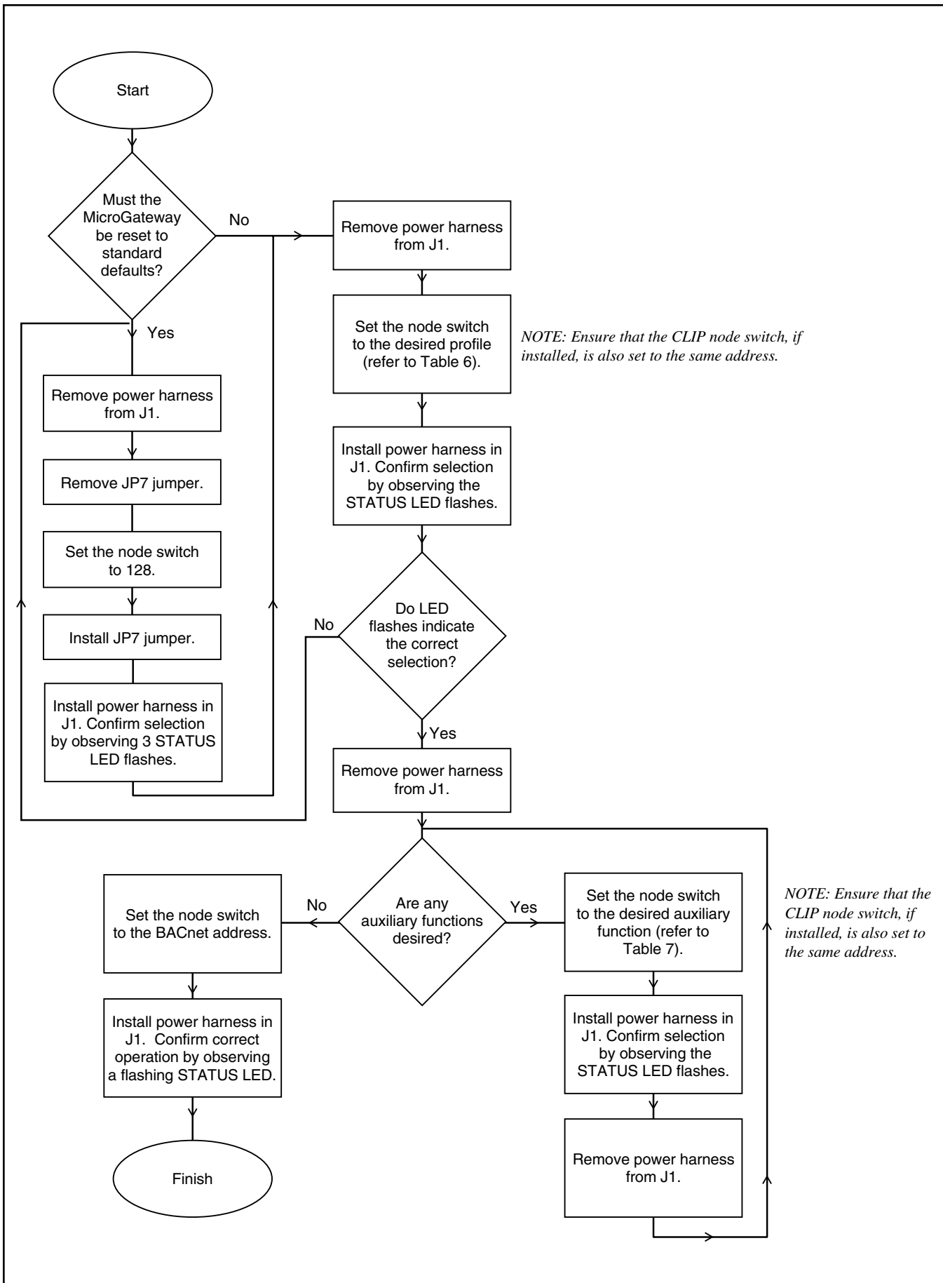
Figure 23. Commissioning Sequence
