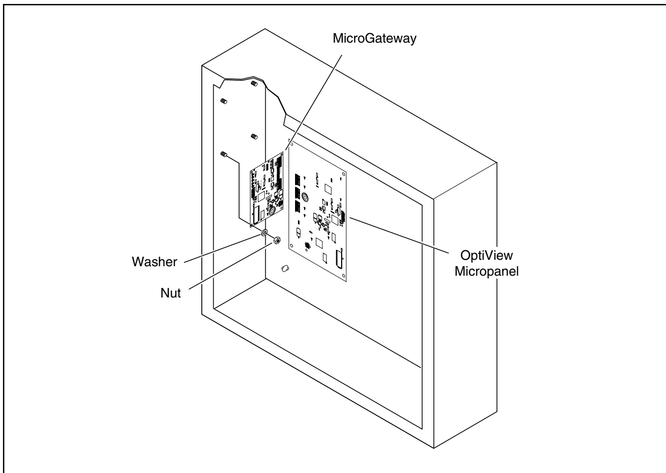
Figure 6. OptiView Mounting
