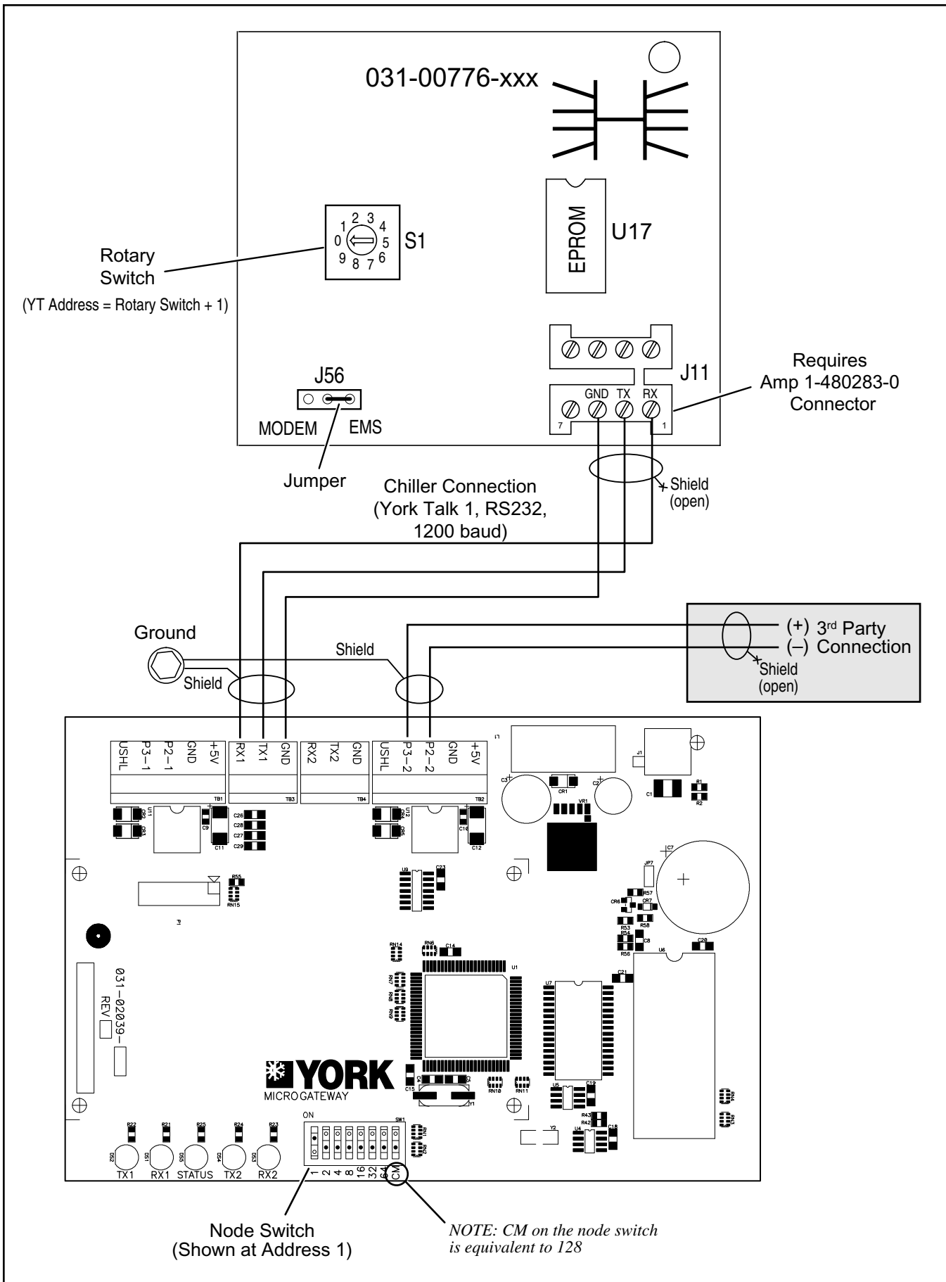
Figure 11. 776 Board Connections
