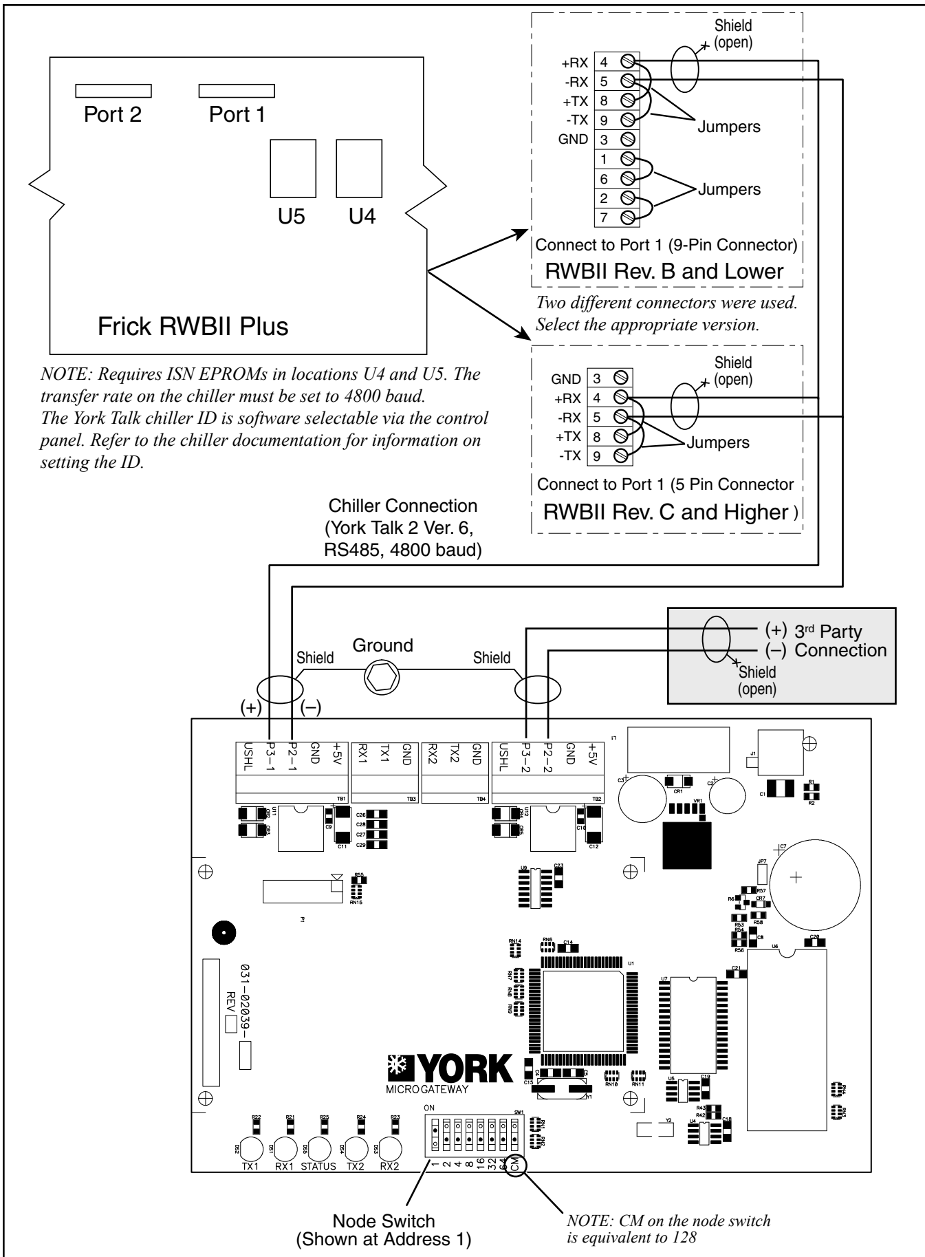
Figure 21. Frick RWB II Board Connections
