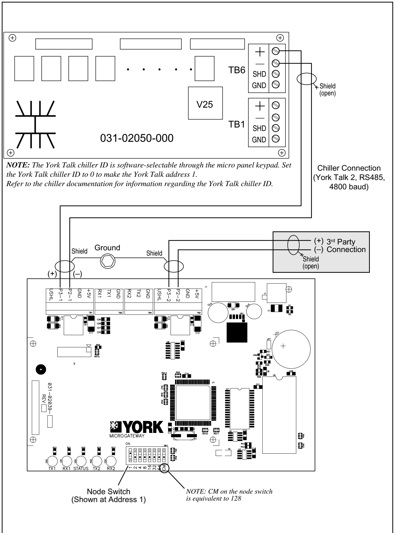
Figure 18. 2050 Board Connections
