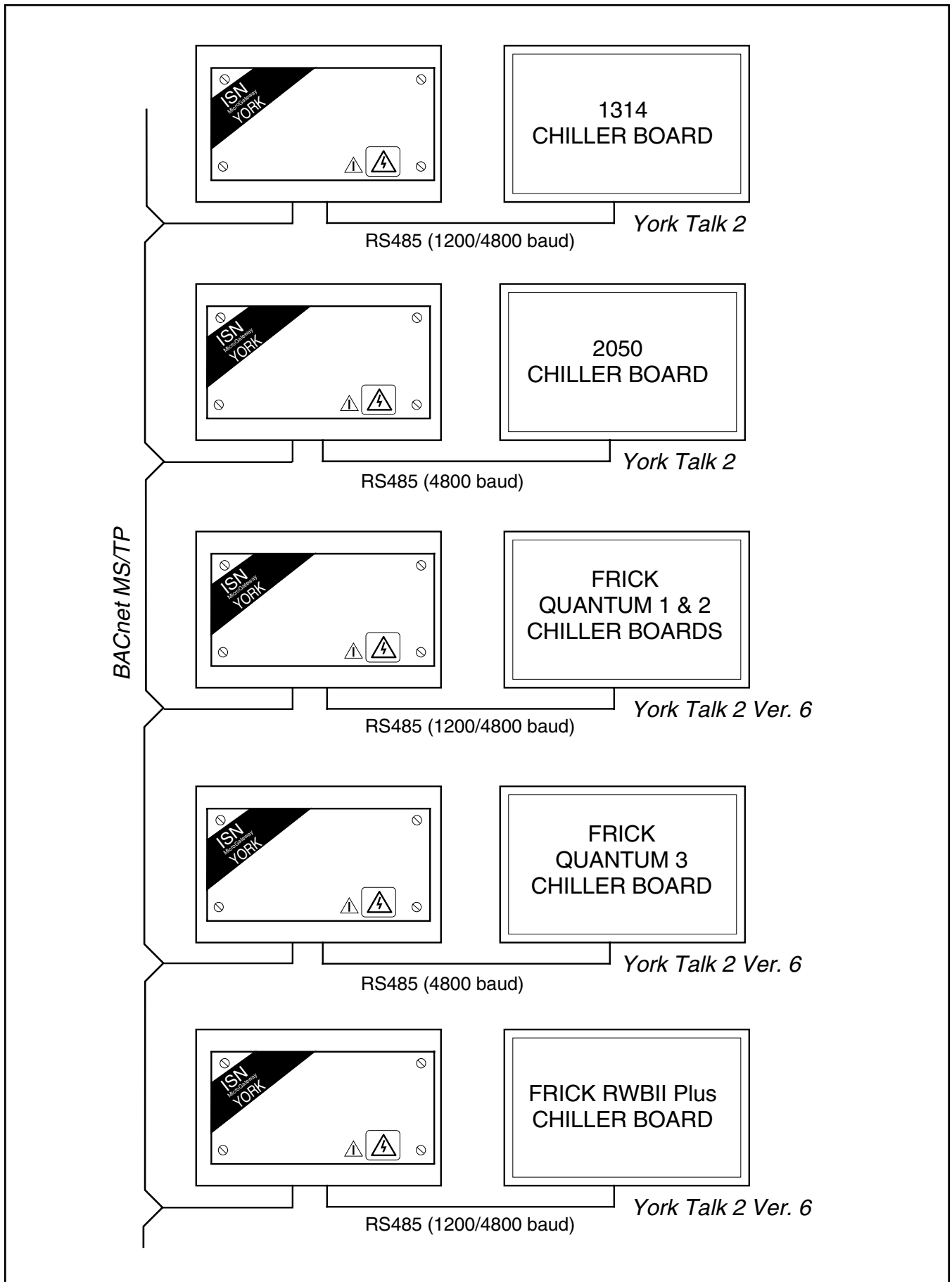
Figure 4. Typical Board Topology
