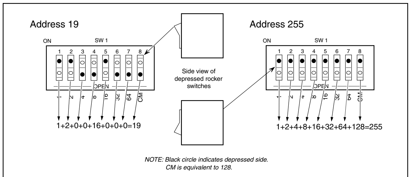
Figure 22. Setting the Node Switch
