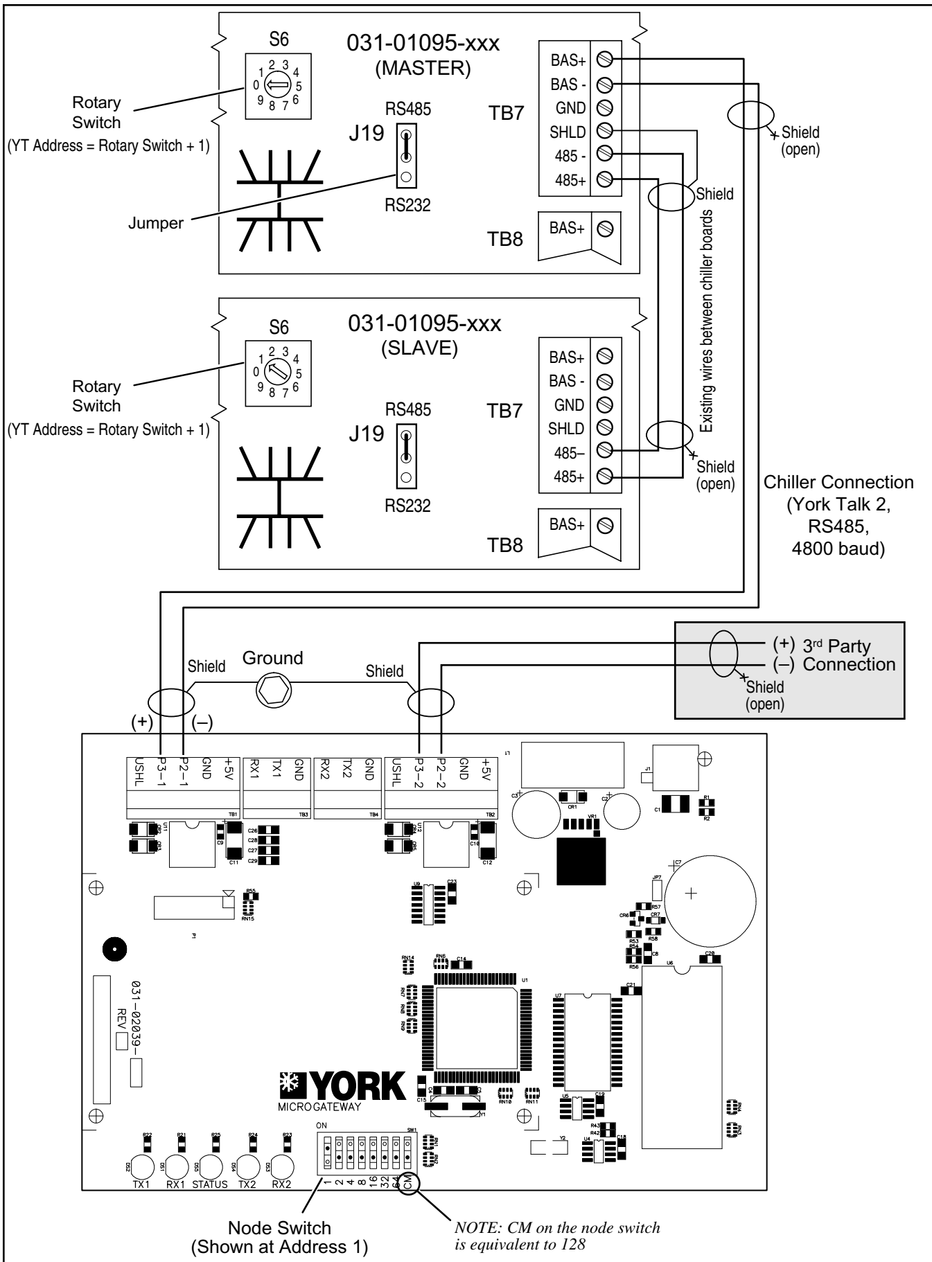
Figure 15. 1095 Master/Slave Board Connections
