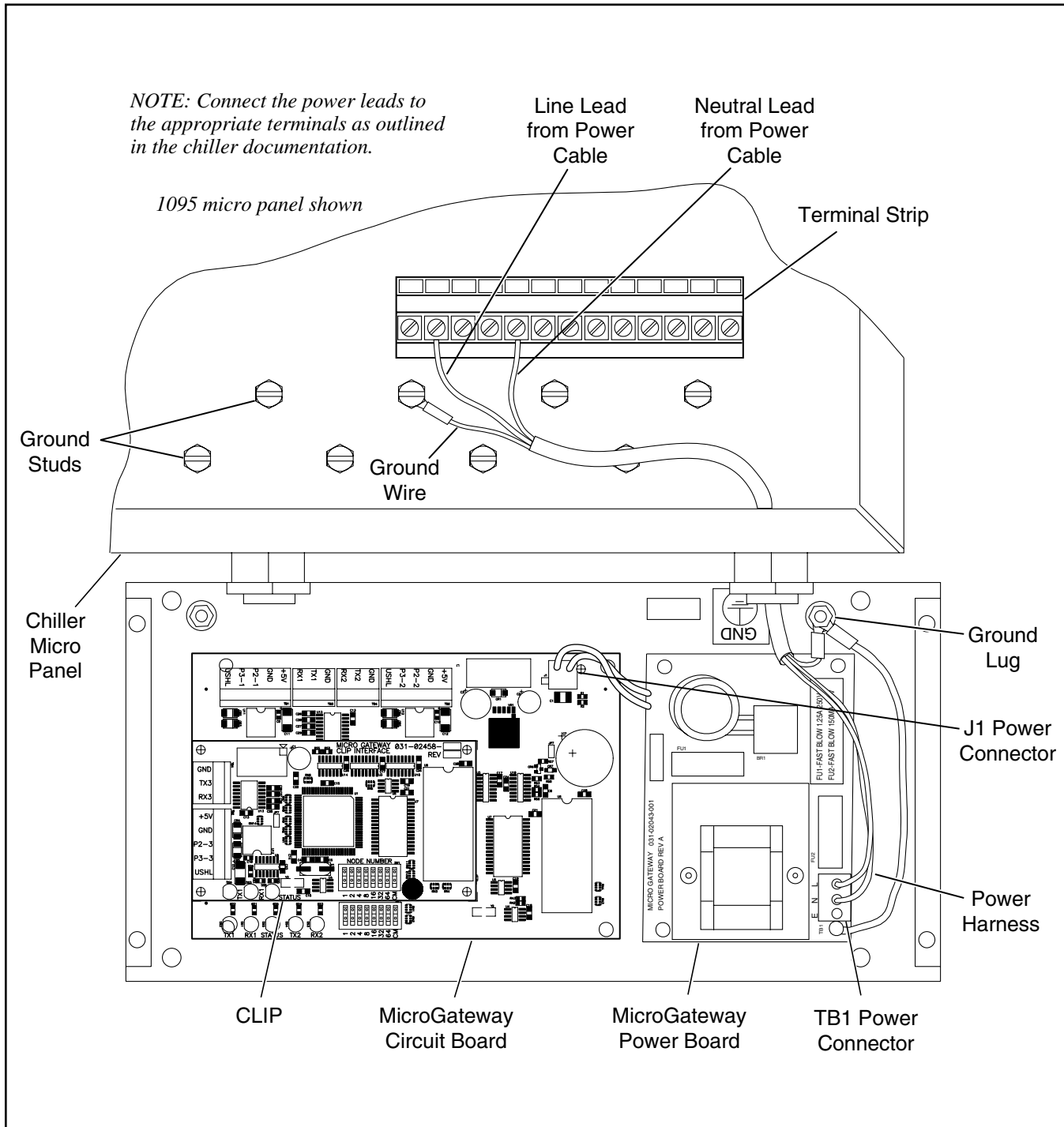
Figure 10. Typical Power Connections for Close-Coupled MicroGateway
