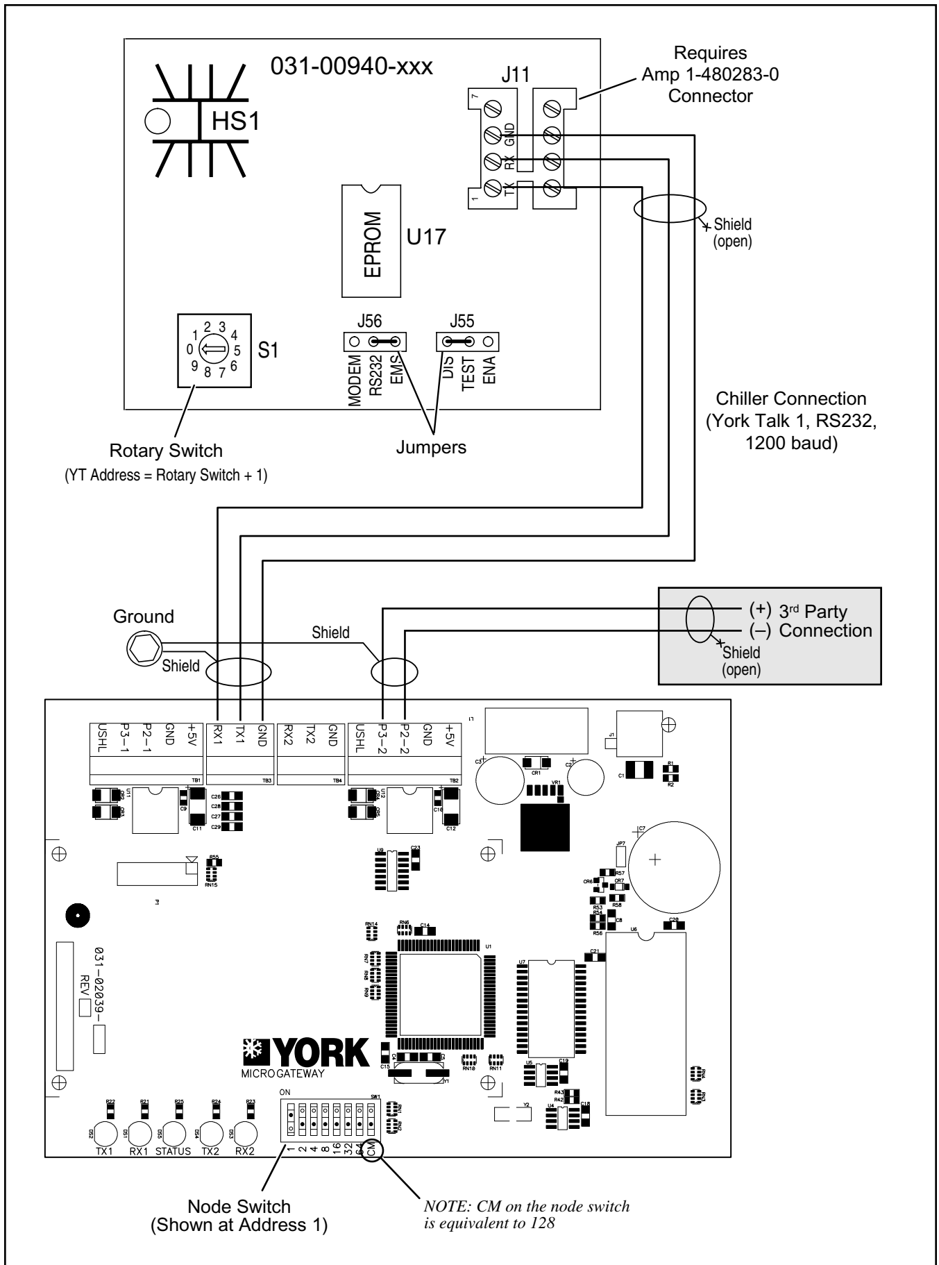
Figure 12. 940 Board Connections
