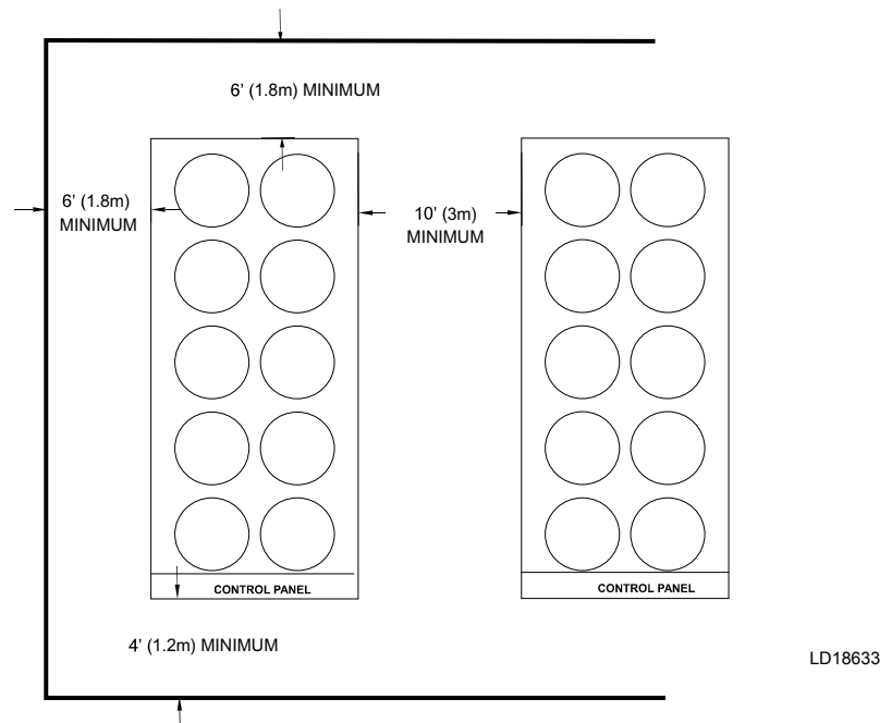
FIGURE 6 - ACCEPTABLE MINIMUM CLEARANCES AROUND/BETWEEN UNIT(S) FOR PROPER AIRFLOW
