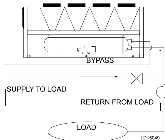
FIGURE 9 - SUGGESTED LAYOUT FOR APPLICATIONS WITH A FLOW RATE LESS THAN THE EVAPORATOR MINIMUM ALLOWABLE FLOW RATE
