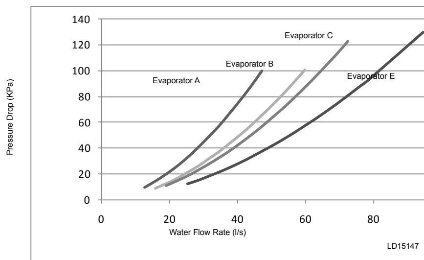
FIGURE 6 - TWO PASS WATER PRESSURE DROP, SI UNITS
