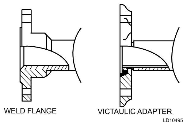
FIGURE 13 - FLANGE ATTACHMENT
