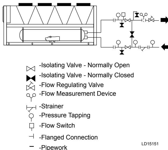
FIGURE 7 - PIPEWORK ARRANGEMENT
