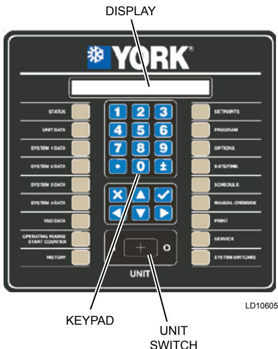
FIGURE 18 - KEYBOARD AND DISPLAY
