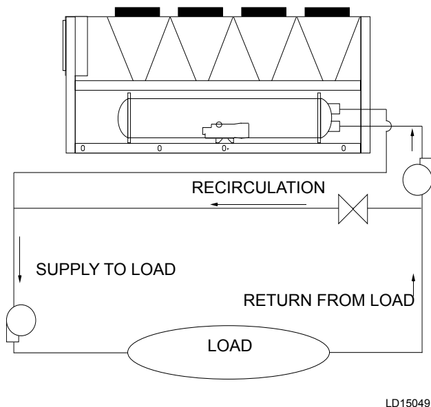
FIGURE 8 - LEAVING WATER TEMPERATURE OUT OF RANGE SUGGESTED LAYOUT
