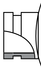
FIGURE 11 - VICTAULIC GROOVE
