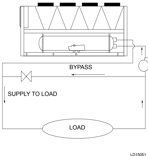
FIGURE 10 - SUGGESTED LAYOUT FOR APPLICATIONS WITH A FLOW RATE GREATER THAN THE EVAPORATOR MAXIMUM ALLOWABLE FLOW RATE
