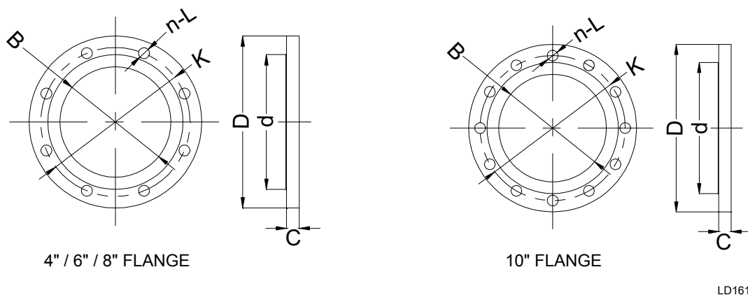
FIGURE 12 - FLANGE FOR GB VESSELS
