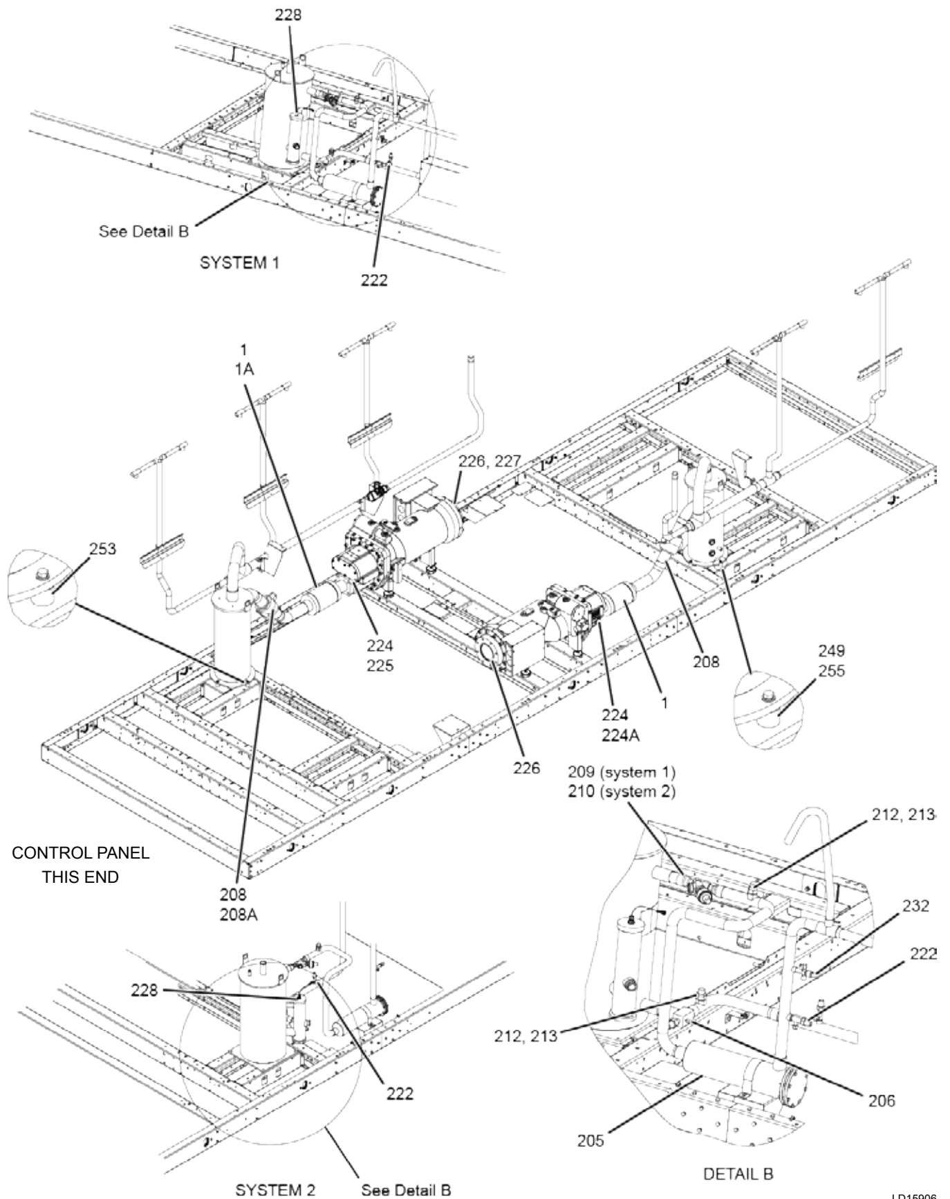
FIGURE 5 - REFRIGERATION CIRCUITS
