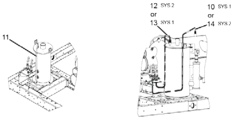
0153 oil separator arrangement for both system 1 and 2.
