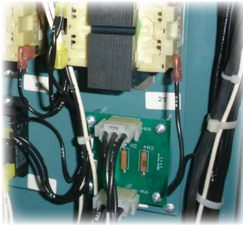
FIGURE 4 - DC BUS ISOLATOR BOARD
