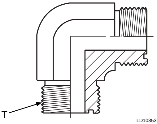
FIGURE 20 - ORFS ELBOW
