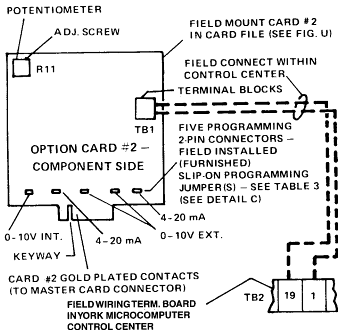
FIG. W—REMOTE LEAVING CHILLED WATER TEMPERATURE SETPOINT OPTION CARD #2
