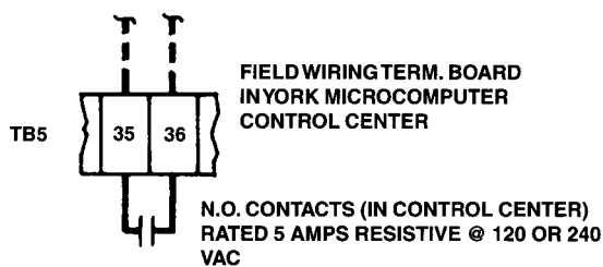
FIG. D—RUN CONTACTS
