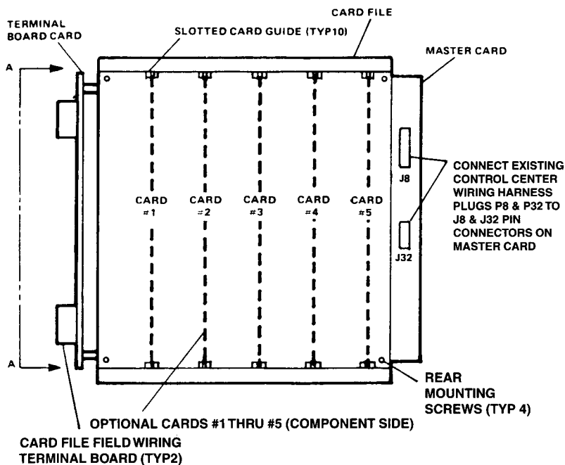
DETAIL—CARD FILE (FRONT VIEW)
