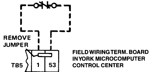
FIG. N—ELECTRO-MECHANICAL STARTER MANUAL RESET OVERLOADS (2300 TO 4160 VOLTS U.L. OR C.S.A. APPROVED UNITS ONLY)
