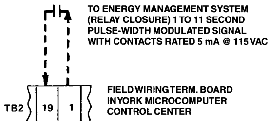
FIG. P—REMOTE LEAVING CHILLED WATER TEMPERATURE SETPOINT WITH PWM SIGNAL
