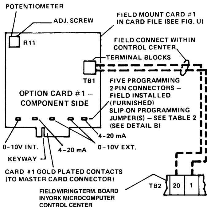
FIG. V—REMOTE CURRENT LIMIT SETPOINT—OPTION CARD #1
