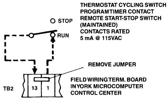
FIG. F—REMOTE/LOCAL CYCLING DEVICES
