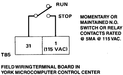
FIG. BB—AUXILIARY SAFETY SHUTDOWN INPUT
