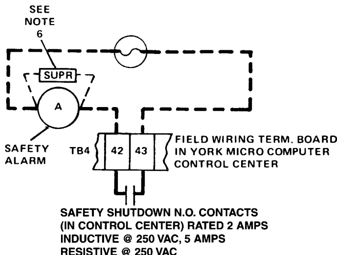
FIG. Y—EXTERNAL SIGNAL FOR REFRIGERATION UNIT FAILURE (NOTE 6)
