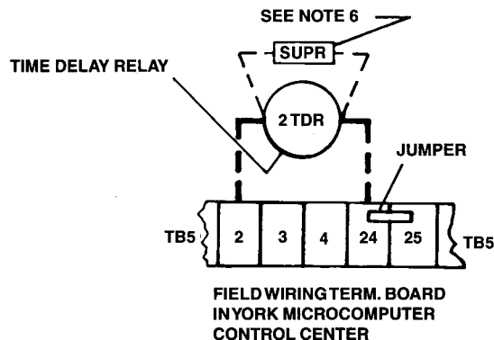
FIG. H—CONDENSER WATER FLOW INTERLOCK (SEE NOTES 6 & 12)
