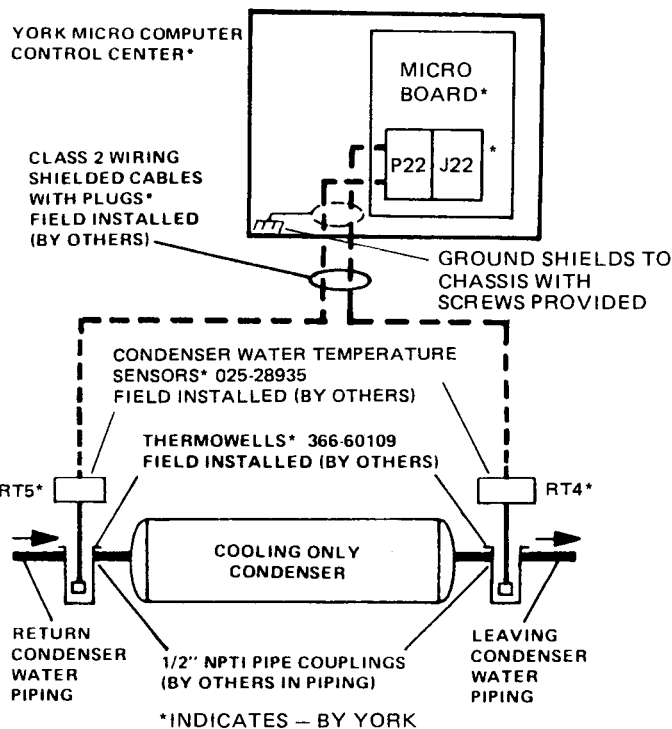
FIG. S—CONDENSER WATER TEMPERATURE SENSORS (KIT)
