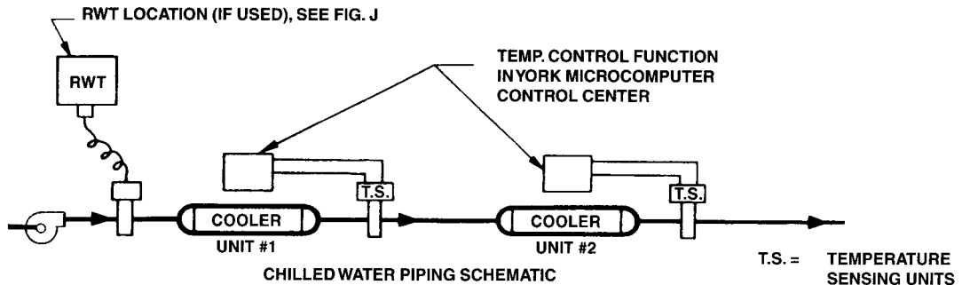
FIG. K—MULTIPLE UNITS (TWO)—SERIES OPERATION (NOTES 8 & 11)
