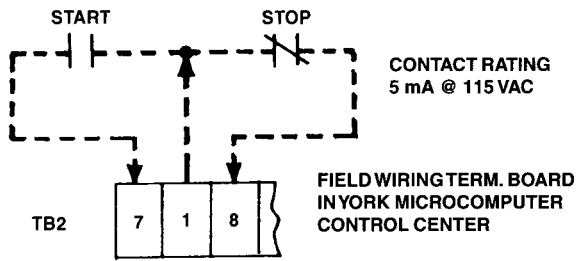
FIG. E—REMOTE START-STOP CONTACTS FROM ENERGY MANAGEMENT SYSTEM
