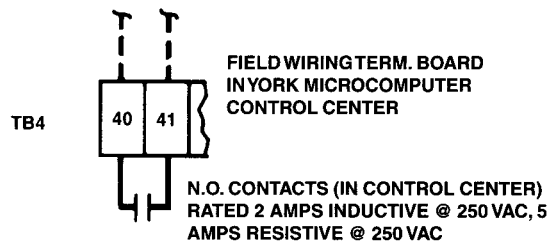
FIG. B - CYCLING SHUTDOWN CONTACTS
