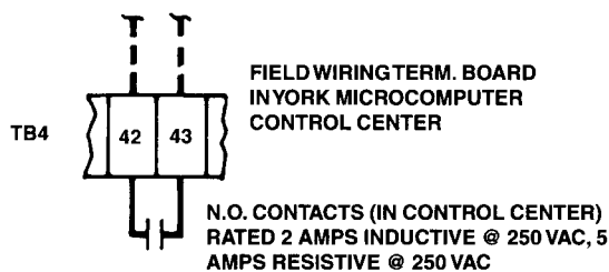
FIG. C—SAFETY SHUTDOWN CONTACTS
