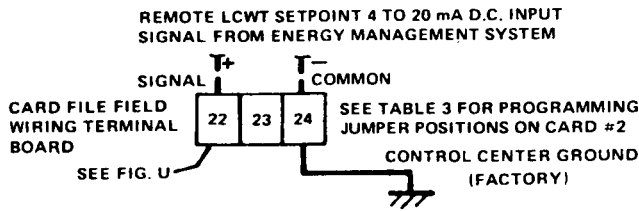
DETAIL 1—4 to 20 mA D.C. INPUT CURRENT SIGNAL CONNECTIONS
