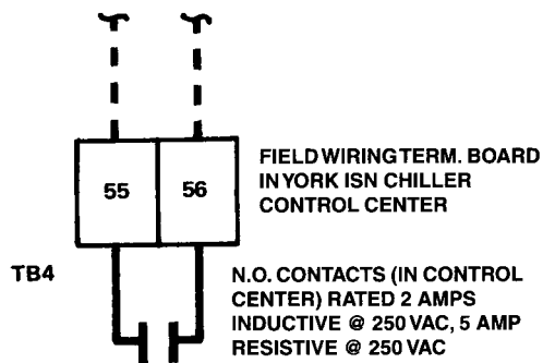
FIG. DD—EXCESS PURGE WARNING CONTACTS
