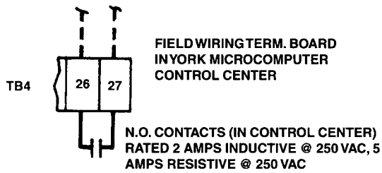
FIG. A - REMOTE MODE READY TO START CONTACTS
