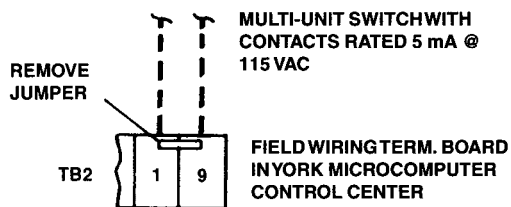
FIG. G—MULTI-UNIT SEQUENCE
