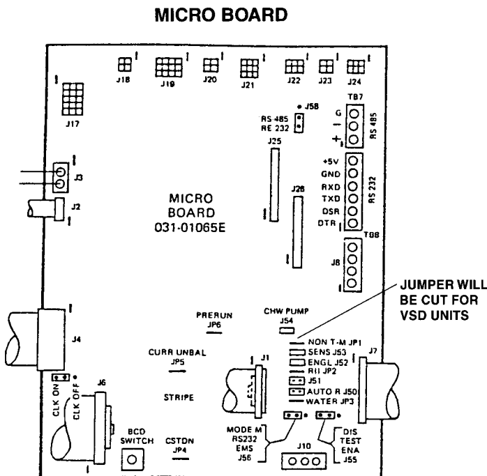
FIG. R—MICRO BOARD JUMPERS FOR AUTO/MANUAL RESTART AFTER POWER FAILURE OR ENGLISH/METRIC DISPLAY UNITS
