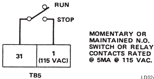
FIG. BB – AUXILIARY SAFETY SHUTDOWN INPUT
