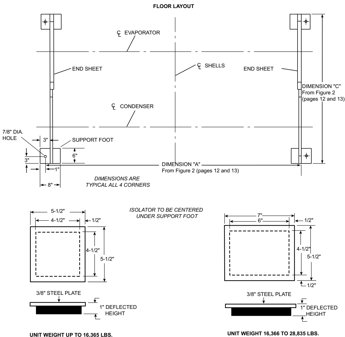
FIGURE 3 - STANDARD NEOPRENE VIBRATION ISOLATOR PAD MOUNTS (ENGLISH)
