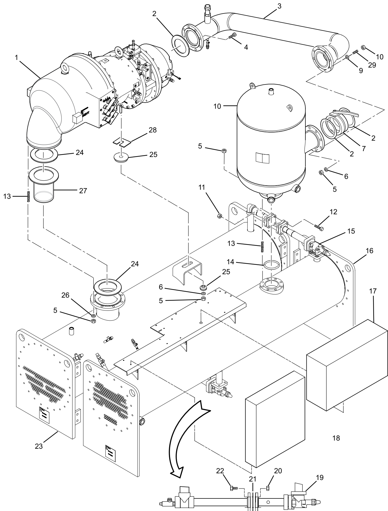
FIGURE 11 - FORM 7 FIELD ASSEMBLY – EXPLODED VIEW
