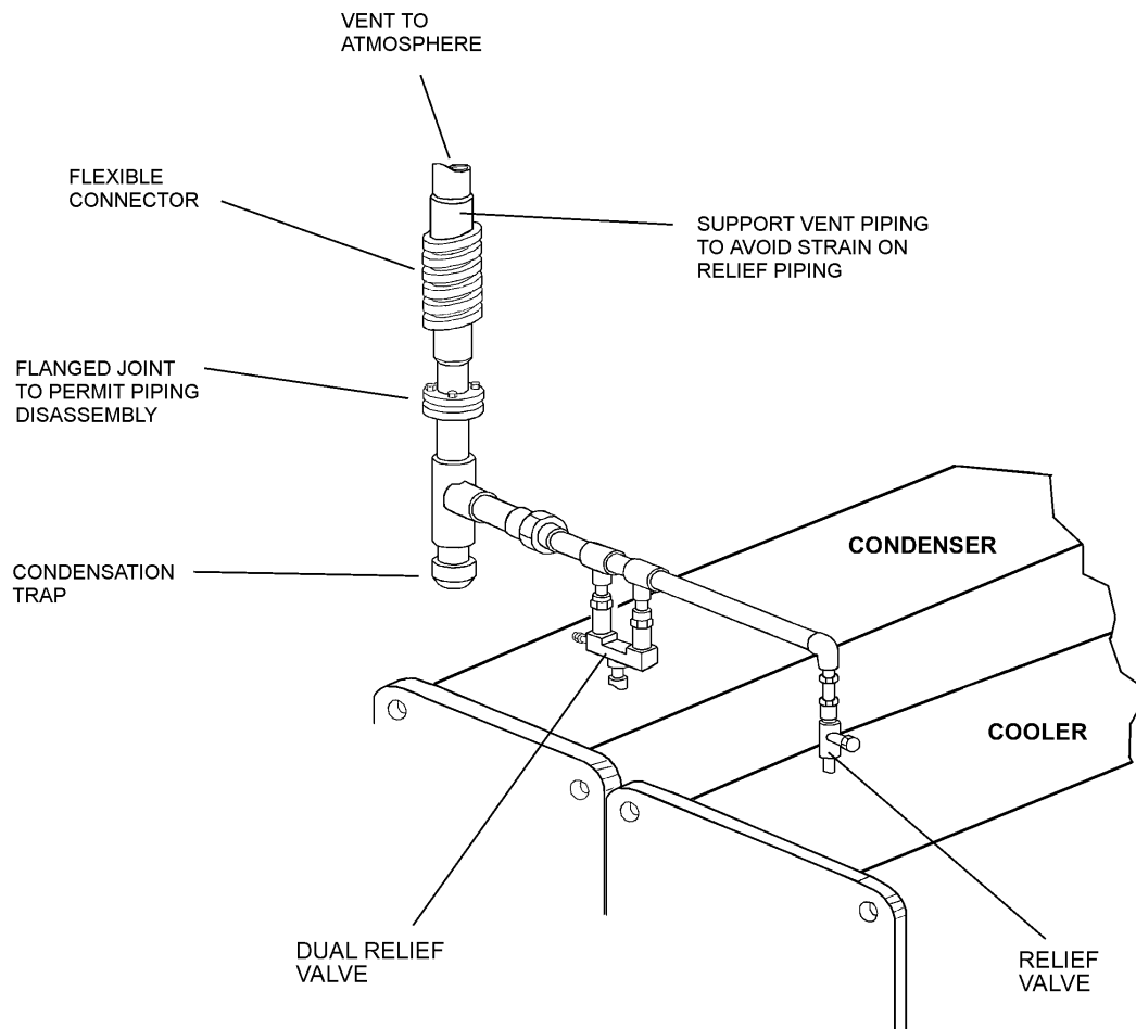
FIGURE 16 - TYPICAL REFRIGERANT VENT PIPING FROM RELIEF VALVES
