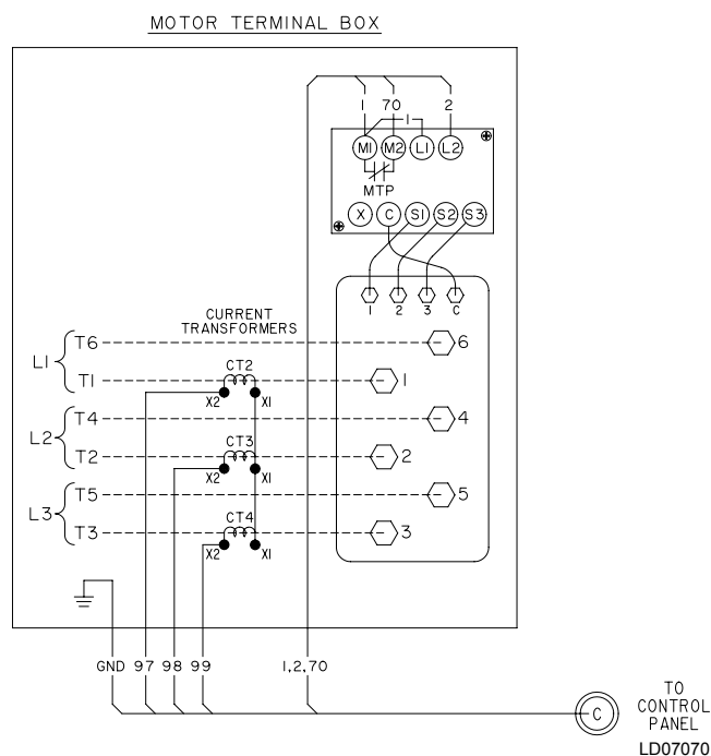
FIGURE 17 - YR MOTOR CONNECTIONS (ELECTRO-MECHANICAL STARTER)
