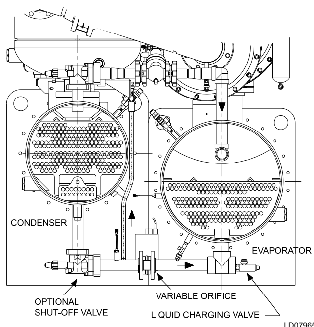
FIGURE 22 - VARIABLE ORIFICE
