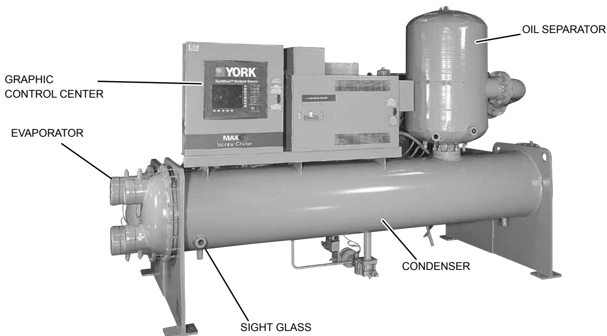
FIGURE 7 - MODEL YR – FRONT VIEW OF ASSEMBLED UNIT
