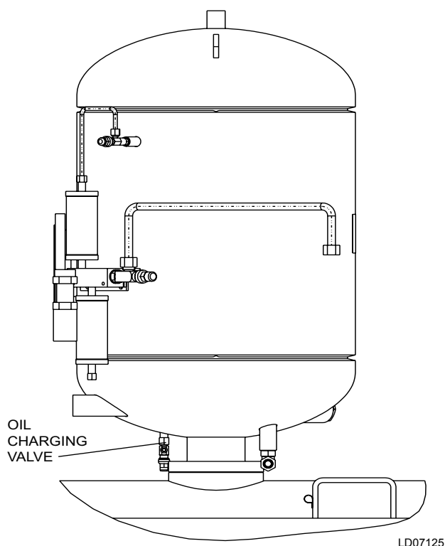
FIGURE 23 - CHARGING OIL
