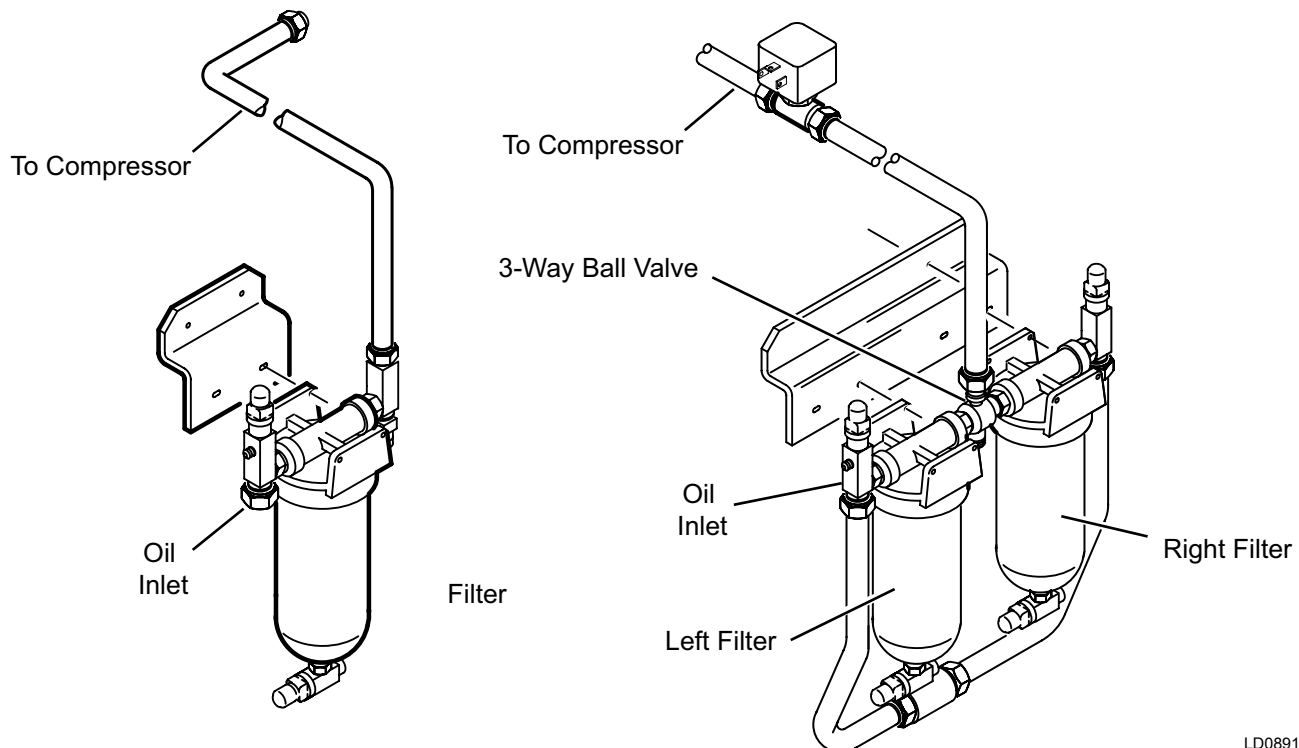
FIGURE 24 - OIL FILTERS
