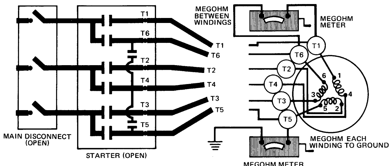
FIGURE 26 - DIAGRAM, MEGOHM MOTOR WINDINGS
