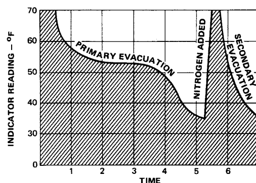
FIGURE 13 - SATURATION CURVE
