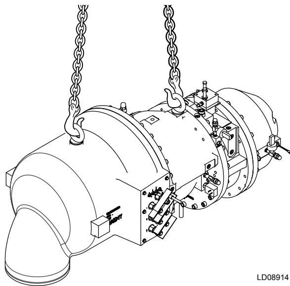
FIGURE 8 - RIGGING COMPRESSOR ASSEMBLY
