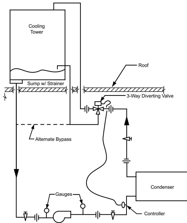
FIGURE 15 - COOLING TOWER PIPING WITH 3 PORT BY-PASS VALVE
