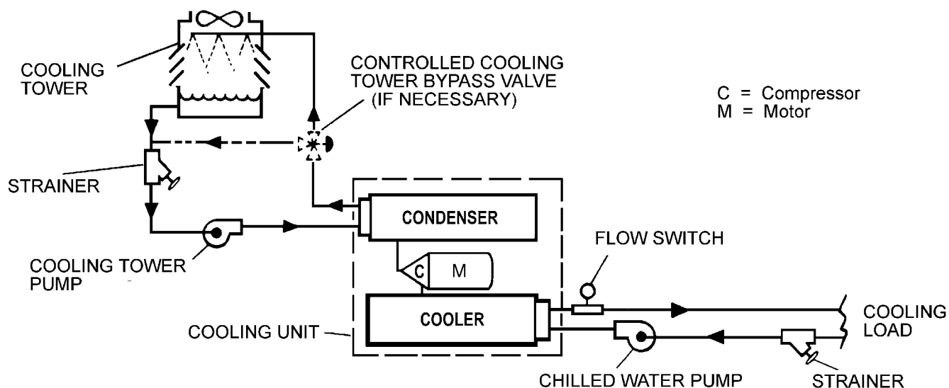
FIGURE 14 - SCHEMATIC OF A TYPICAL PIPING ARRANGEMENT
