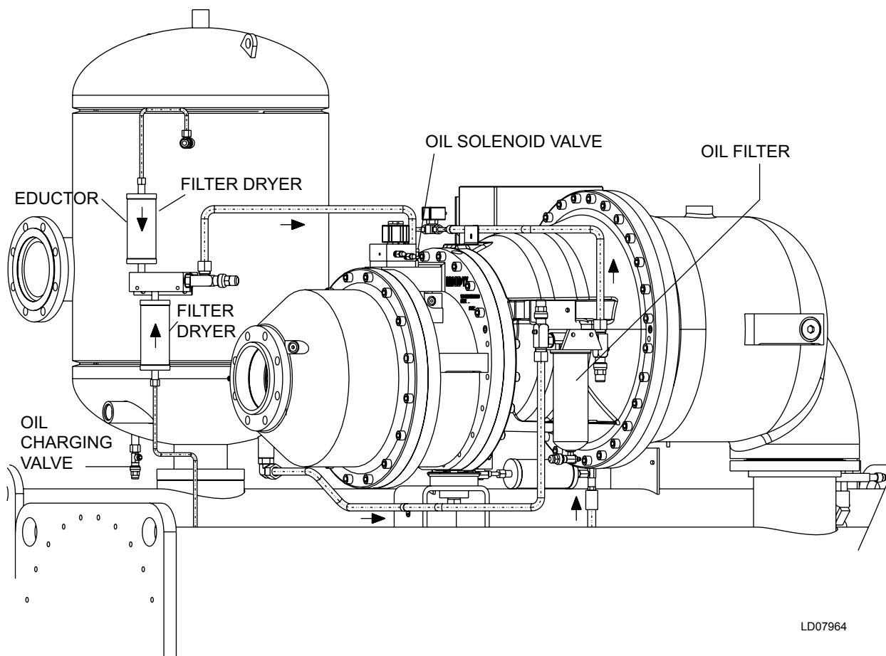
FIGURE 20 - OIL FILTER SYSTEM
