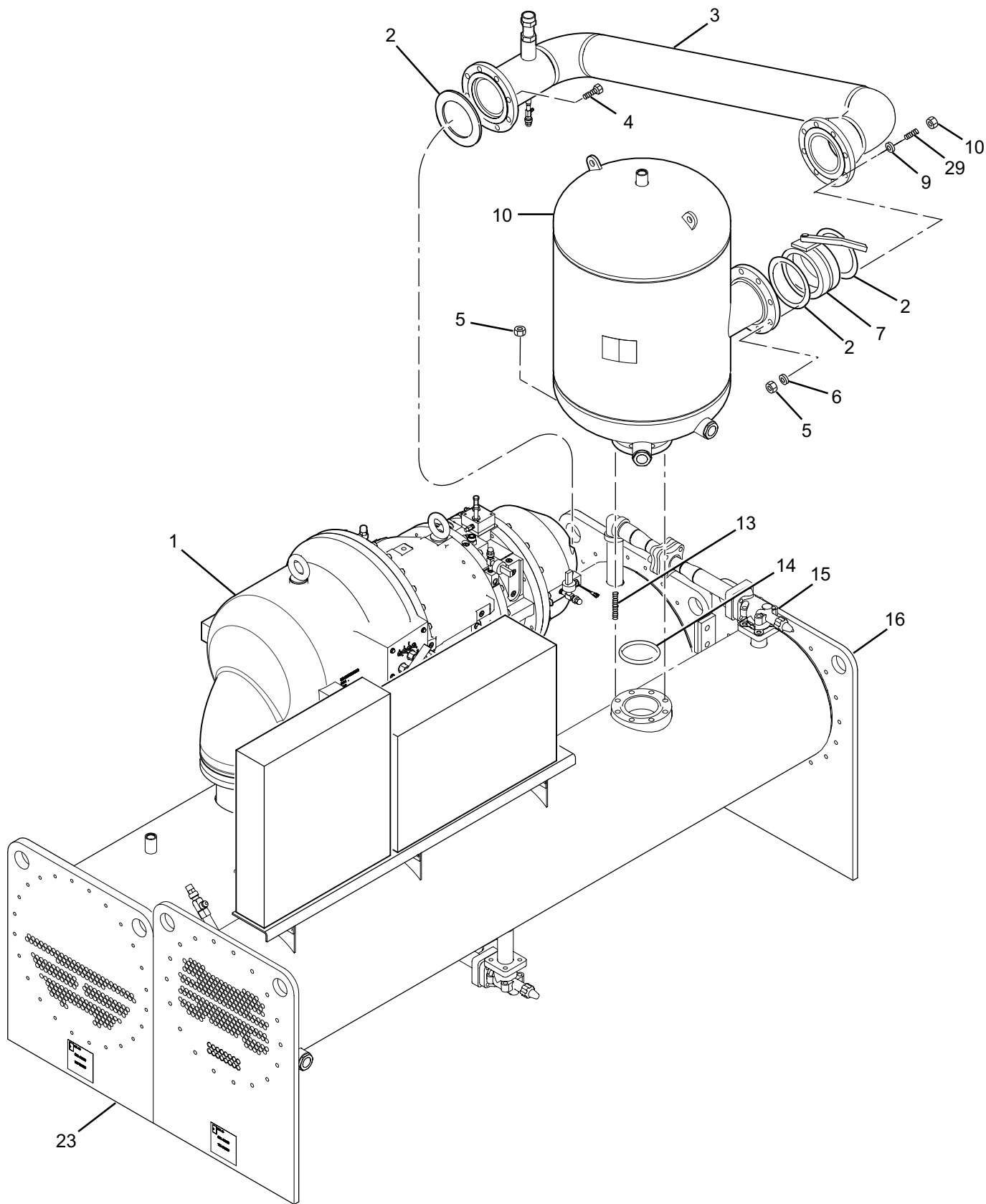
FIGURE 12 - FORM 8 FIELD ASSEMBLY – EXPLODED VIEW
