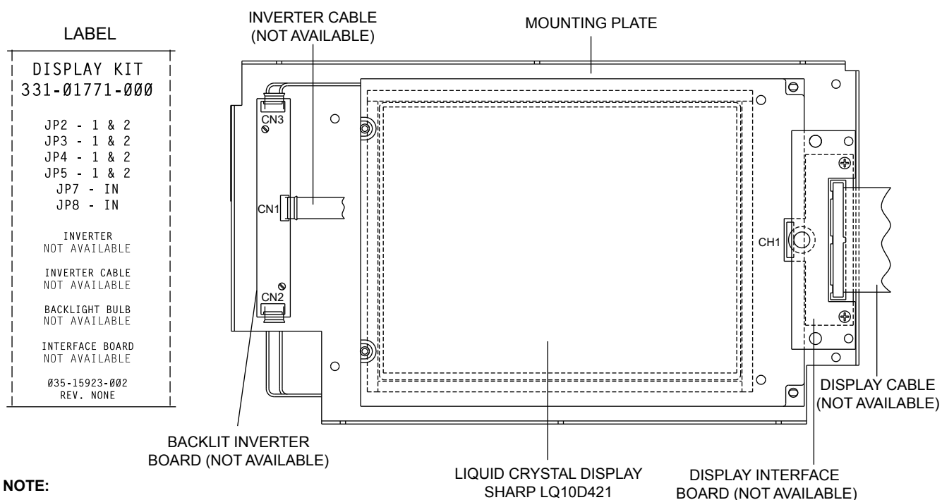
FIGURE 24 - LIQUID CRYSTAL DISPLAY ASSEMBLY – SHARP LQ10D421 DISPLAY
