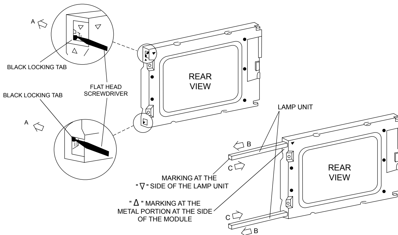
FIGURE 29 - DISPLAY (SHARP LQ10D421) LAMP REPLACEMENT
