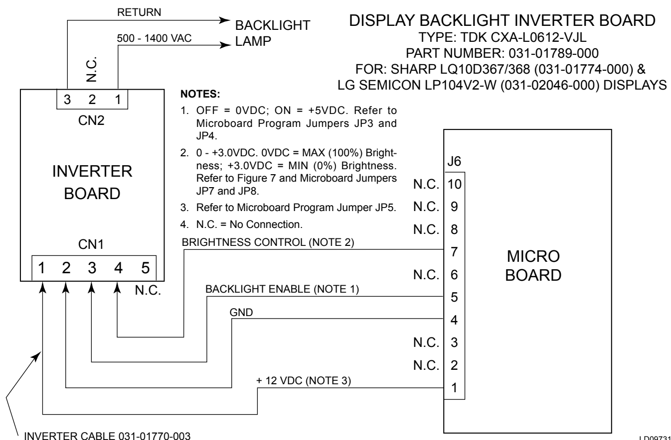
FIGURE 33 - DISPLAY BACKLIGHT INVERTER BOARD (SHARP LQ10D367/368 (031-01774-000) AND LG SEMICON LP104V2-W) (031-02046-000)
