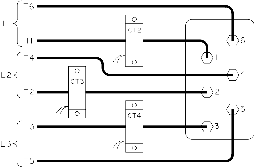
COMPRESSOR MOTOR FIELD CONNECTION DIAGRAM 200 TO 600 VOLTS
