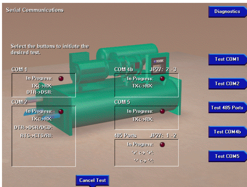
FIGURE 52 - SERIAL INPUTS / OUTPUTS TEST SCREEN
