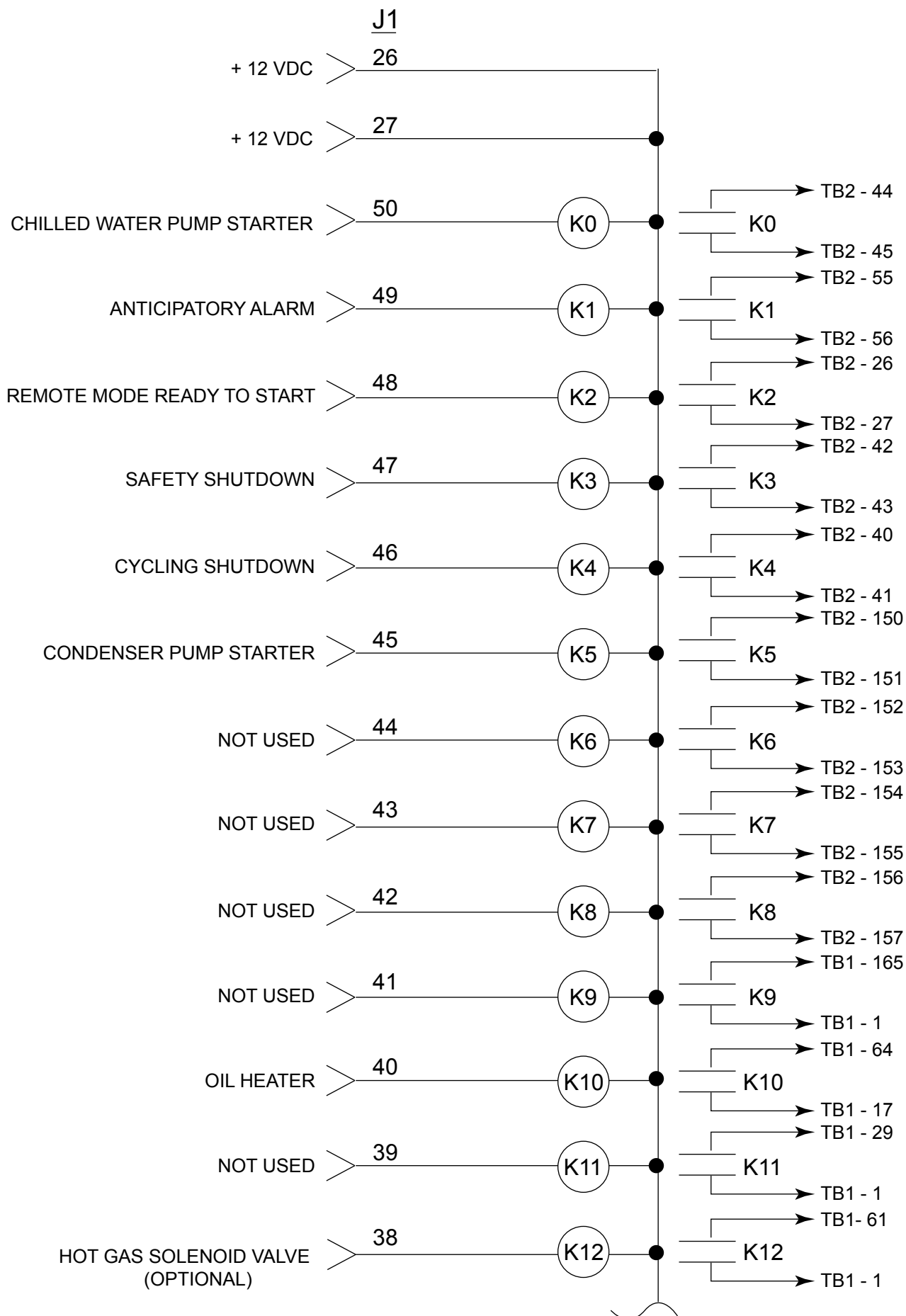
FIGURE 21 - I/O BOARD DIGITAL OUTPUTS
