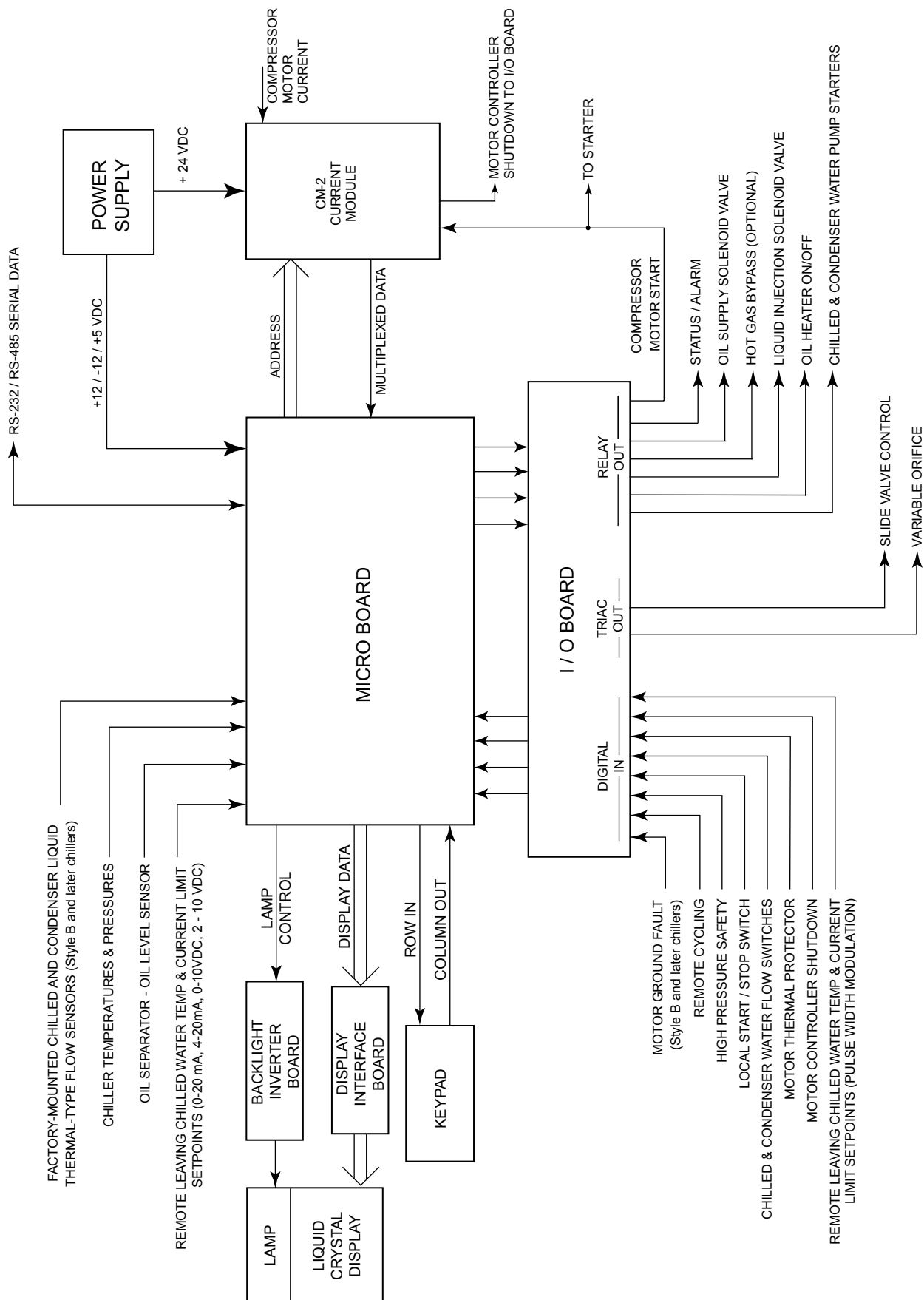
FIGURE 1 - CONTROL CENTER - ELECTRO-MECHANICAL STARTER APPLICATIONS
