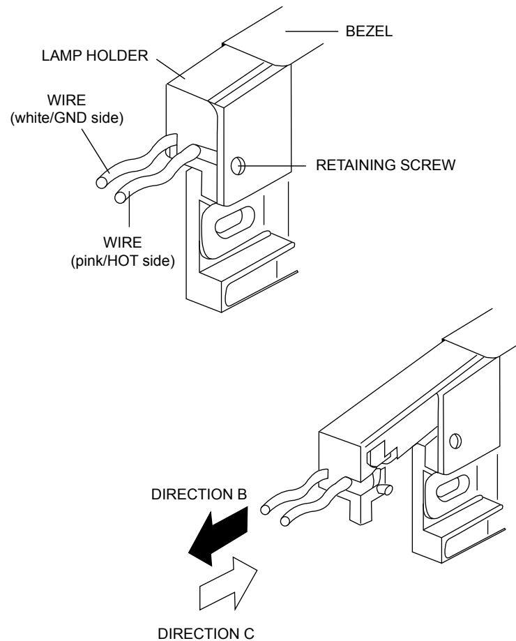
FIGURE 31 - DISPLAY (LG SEMICON LP104V2-W (031-02046-000)) LAMP REPLACEMENT
