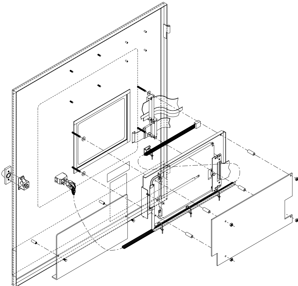
FIGURE 22 - DISPLAY, MOUNTING
