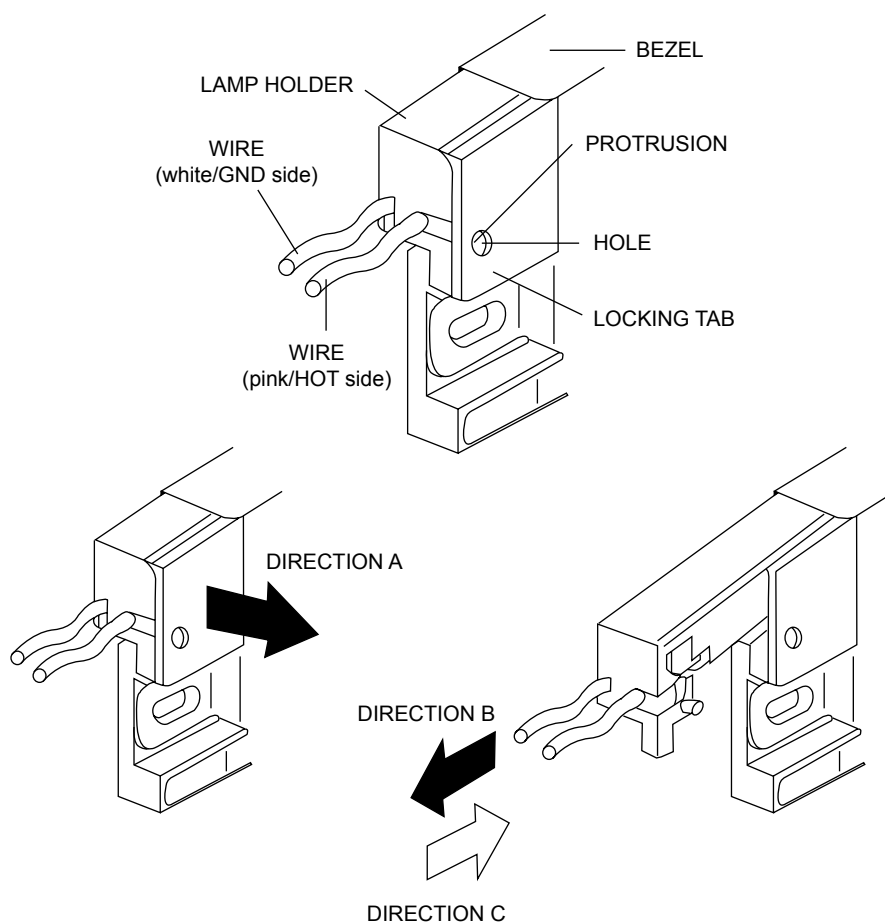
FIGURE 28 - DISPLAY (SHARP LQ10D367) LAMP REPLACEMENT
