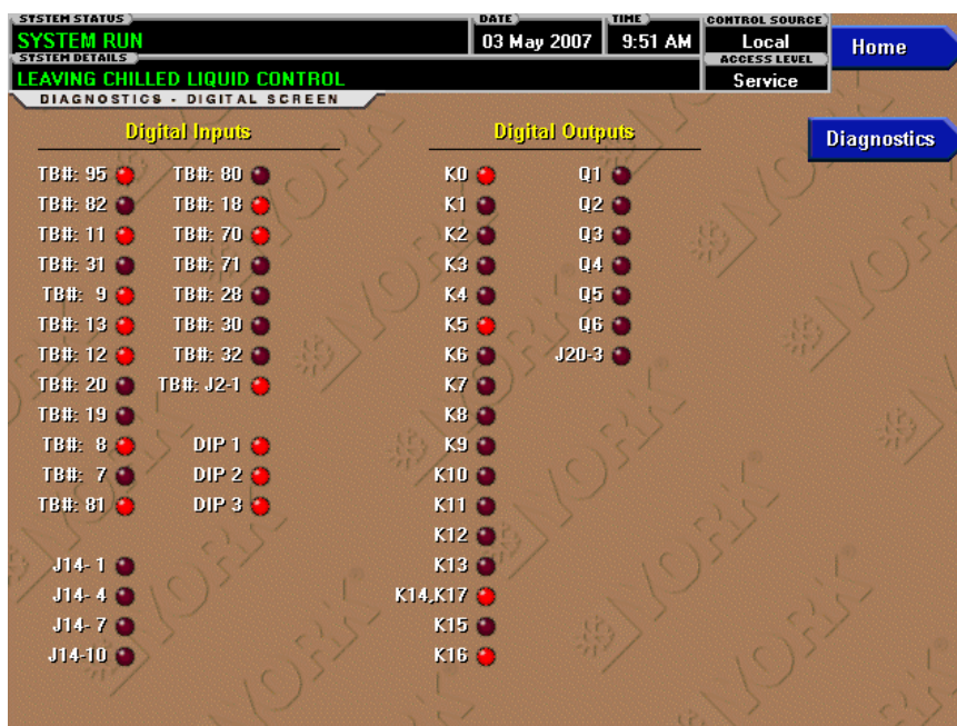
FIGURE 54 - DIGITAL INPUTS / OUTPUTS TEST SCREEN
