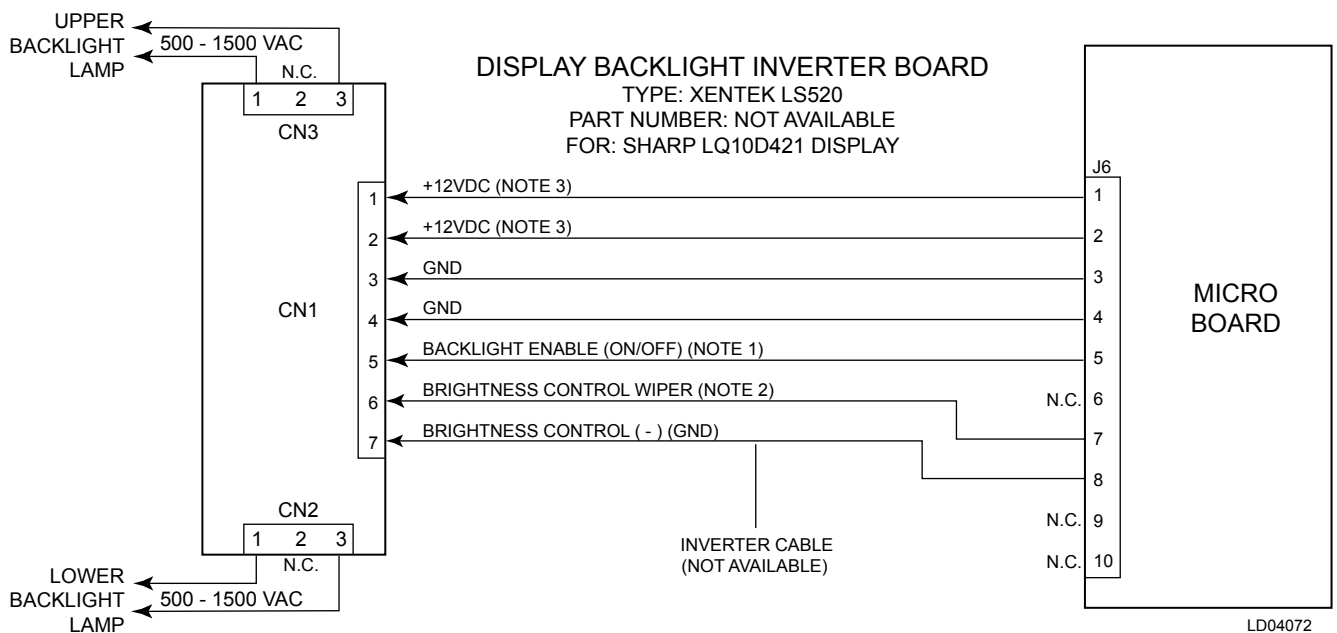
FIGURE 34 - DISPLAY BACKLIGHT INVERTER BOARD (NEC NL6448AC33-24)
