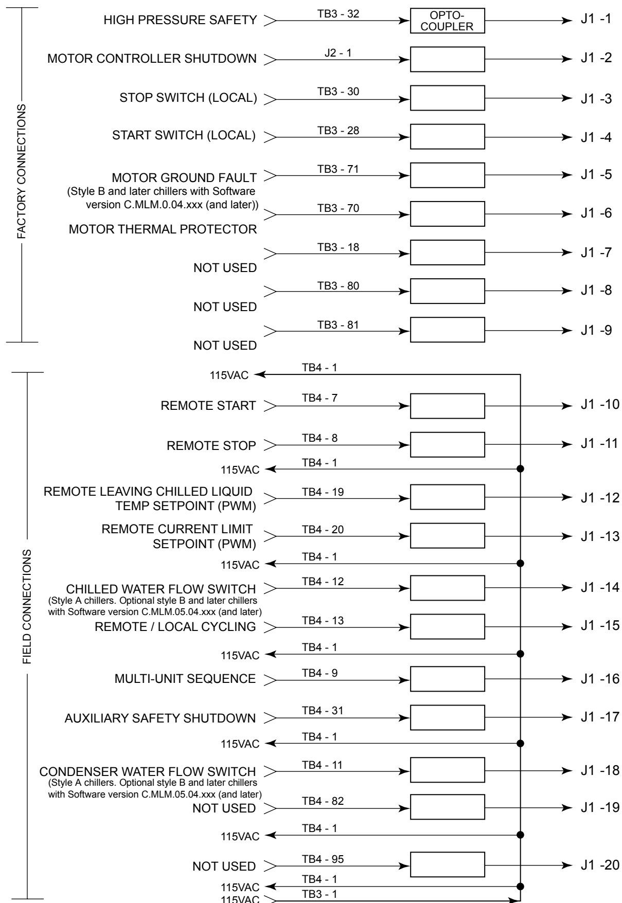
FIGURE 18 - I/O BOARD DIGITAL INPUTS
