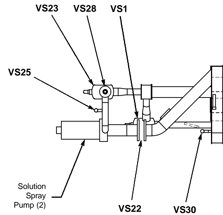
VIEW B-B
