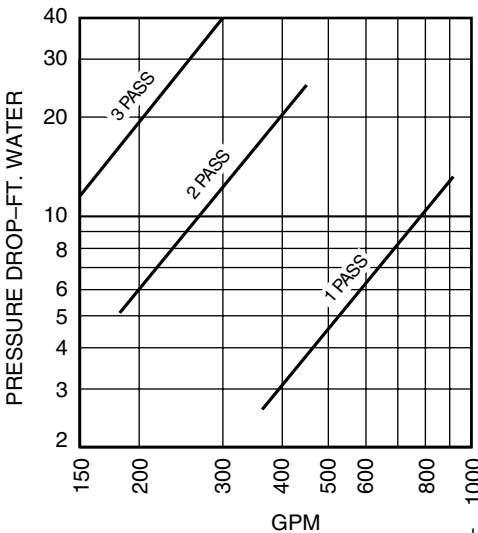
HOT WATER
