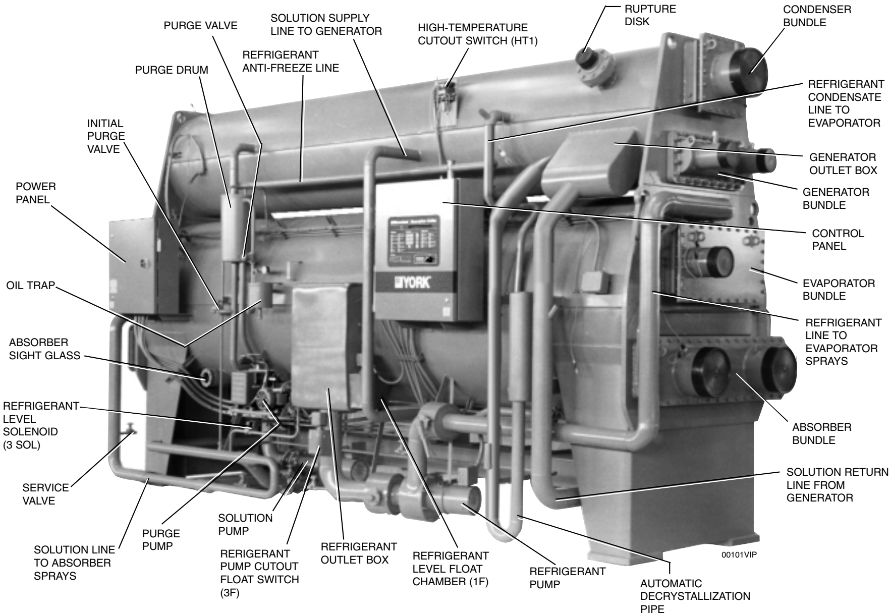
FIG. 3 – MODEL Y1A ABSORPTION UNIT, FRONT VIEW
