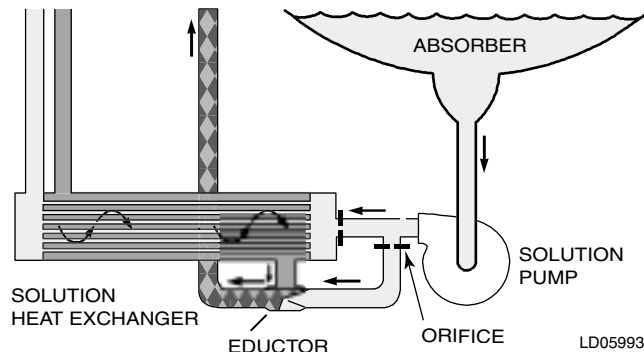
FIG. 7 – SOLUTION PUMP
