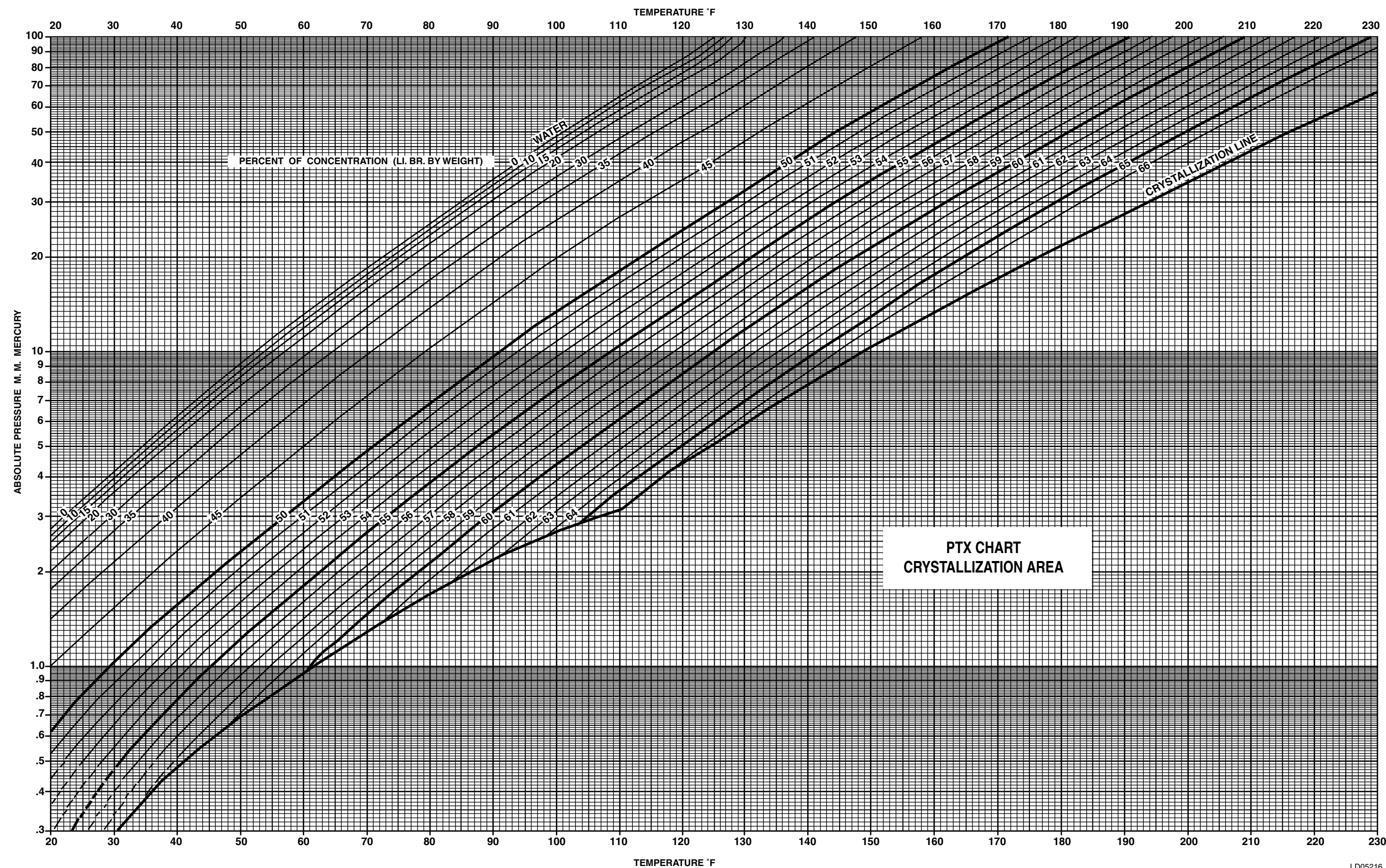
FIG. 23 – PTX CHART
