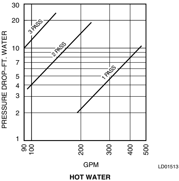
FIG. 24 – PRESSURE DROP CURVES (CONTINUED)
