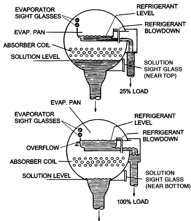
FIG. 12 – SOLUTION AND REFRIGERANT LEVEL VARIATION WITH LOAD
