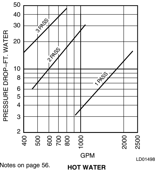
FIG. 24 – PRESSURE DROP CURVES (CONTINUED)
