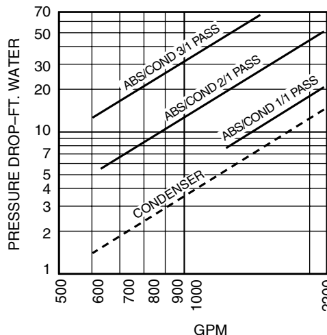
TOWER WATER *
