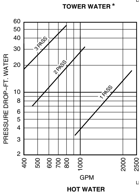
FIG. 24 – PRESSURE DROP CURVES (CONTINUED)
