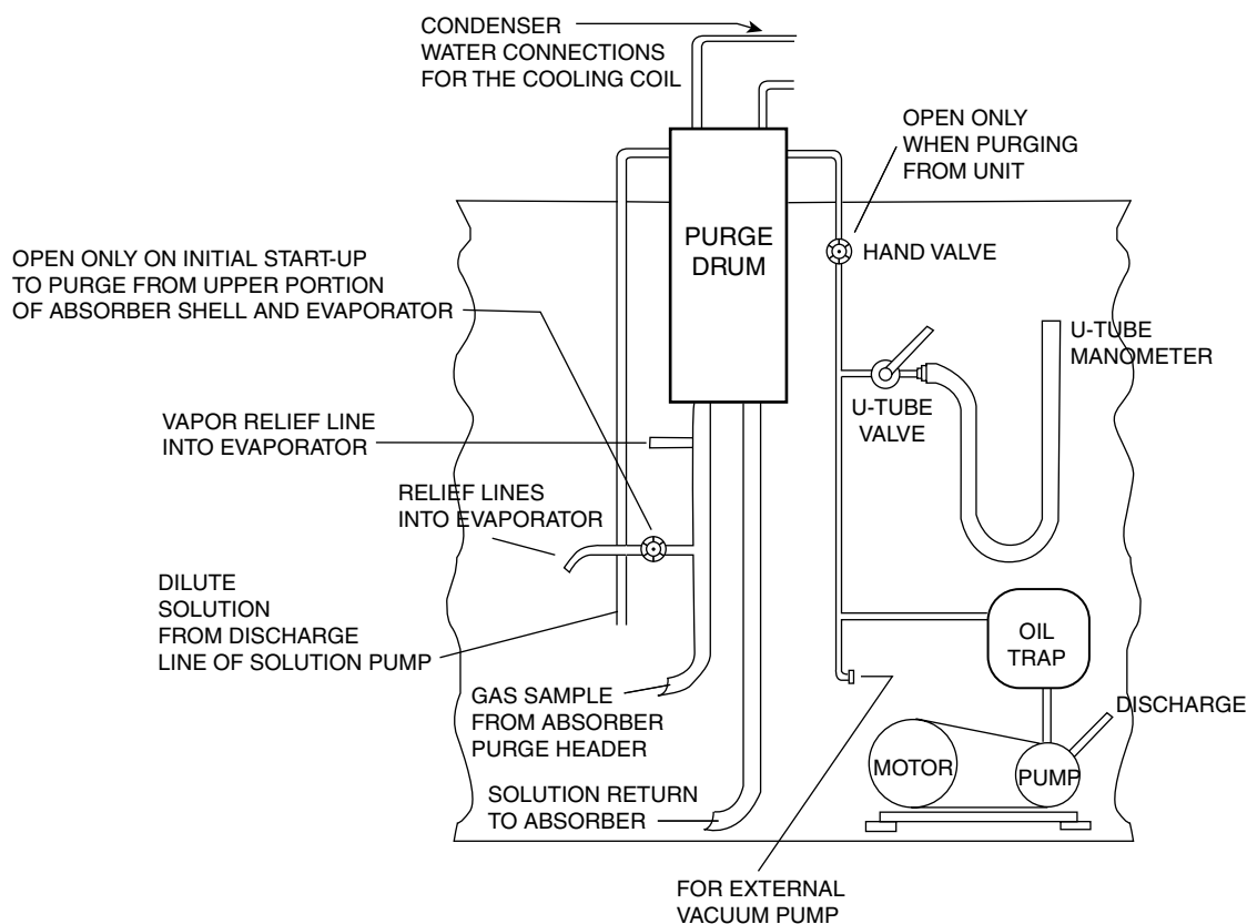
FIG. 17 – THE COMPLETE PURGE SYSTEM
