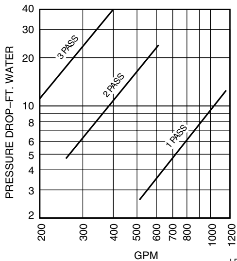
FIG. 24 – PRESSURE DROP CURVES (CONTINUED)
