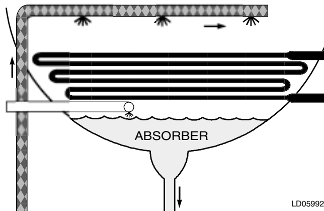
FIG. 6 – ABSORBER
