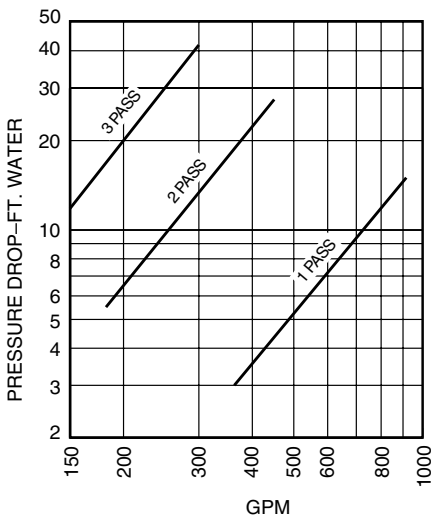
HOT WATER
