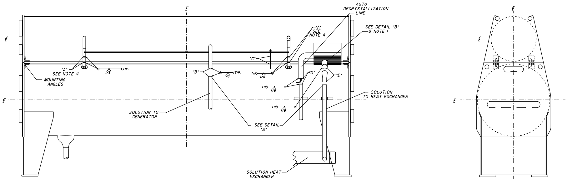
FIG. 9 – UNIT ASSEMBLY FOR MODELS 12F1 THRU 14F3
