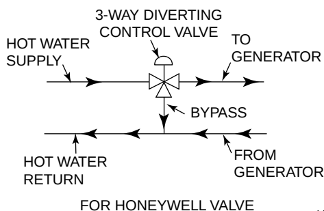
FIG. 17 – DIVERTING SERVICE FOR HONEYWELL VALVE
