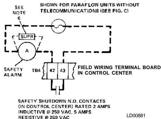
FIG. Y – EXTERNAL SIGNAL FOR SAFETY SHUTDOWN (NOTE 6)
