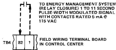
FIG. Q – REMOTE STEAM LIMIT SETPOINT WITH PWM SIGNAL (STEAM UNITS ONLY)
