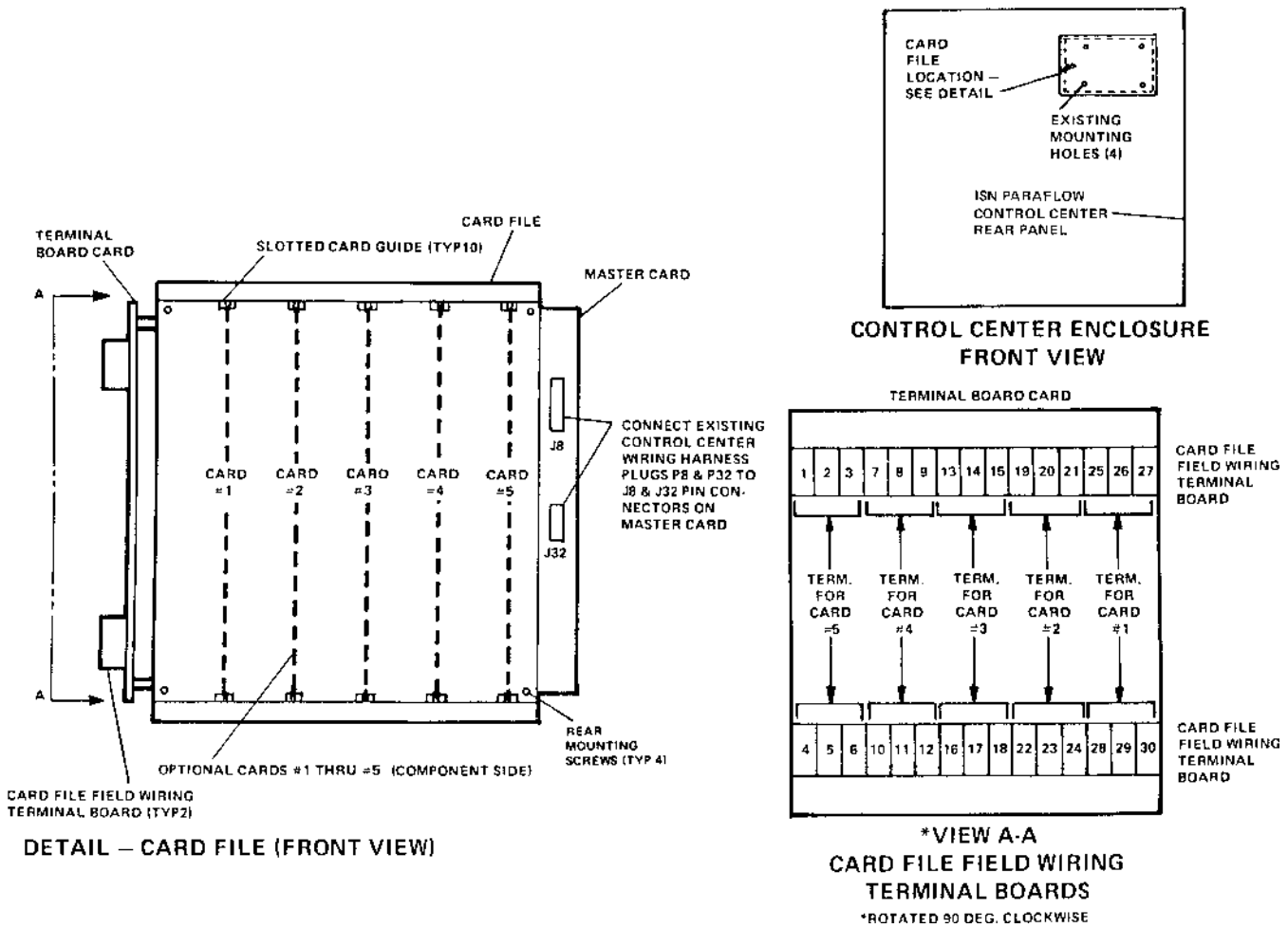
FIG. U – CARD FILE
