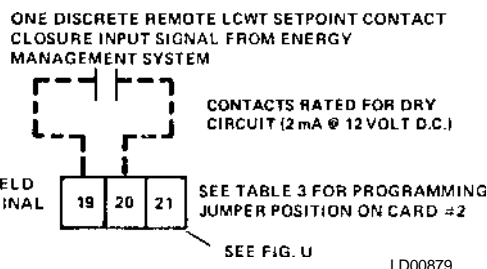
DETAIL 3 – CONTACT CLOSURE INPUT SIGNAL CONNECTIONS
