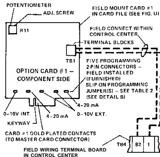
FIG. V - REMOTE STEAM LIMIT SETPOINT - OPTION CARD #1
