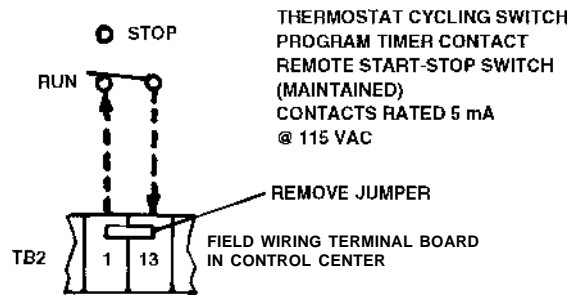
FIG. F – REMOTE/LOCAL CYCLING DEVICES
