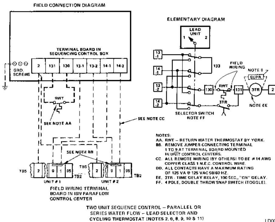
FIG. J – TWO UNIT SEQUENCE CONTROL (COOLING APPLICATION ONLY)
