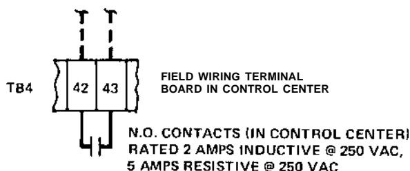
FIG. C – SAFETY SHUTDOWN CONTACTS
