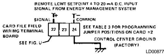
DETAIL 1 – 4 to 20 mA INPUT CURRENT SIGNAL CONNECTIONS
