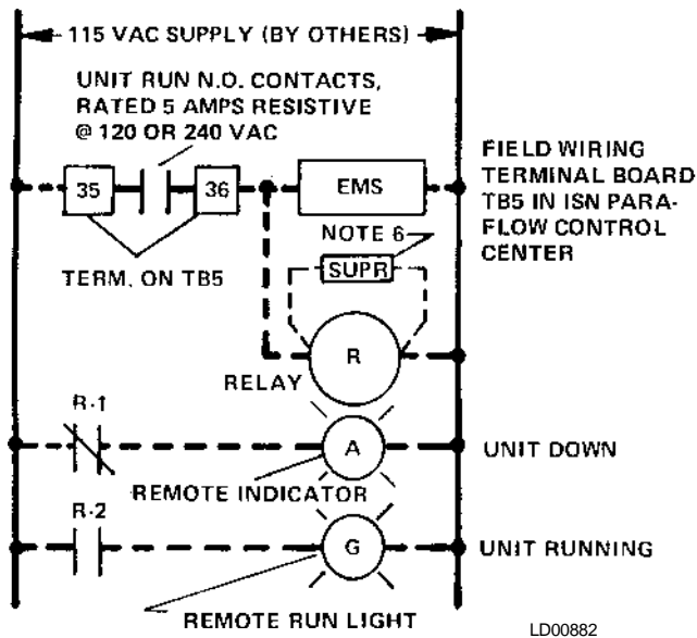
FIG. AA – RUN CONTACTS/REMOTE RUN LIGHT AND SHUTDOWN INDICATOR PLUS EMS
