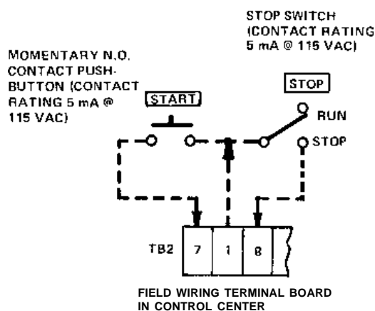
FIG. X – REMOTE START-STOP PUSHBUTTON STATION
