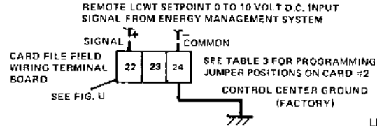
DETAIL 2 – 0 to 10 mA VOLT D.C. INPUT VOLTAGE SIGNAL CONNECTIONS
