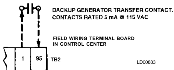
FIG. BB – BACKUP GENERATOR TRANSFER
