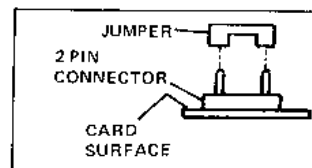
DETAIL C - JUMPER END VIEW
