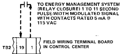
FIG. P – REMOTE LEAVING CHILLED OR HOT WATER TEMPERATURE SETPOINT WITH PWM SIGNAL (NOTE 14)
