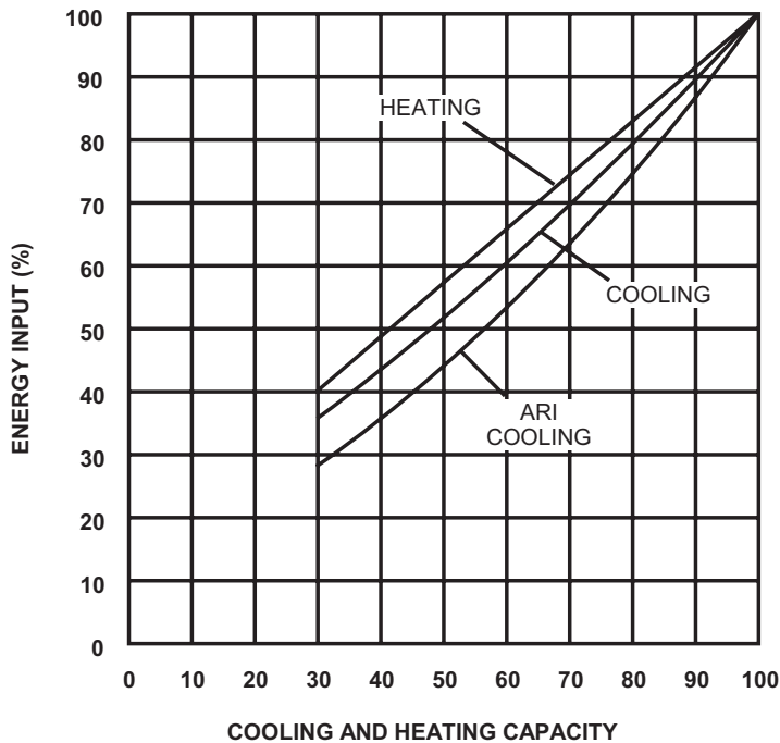
FIGURE 1 - ENERGY INPUT VS. OUTPUT*
