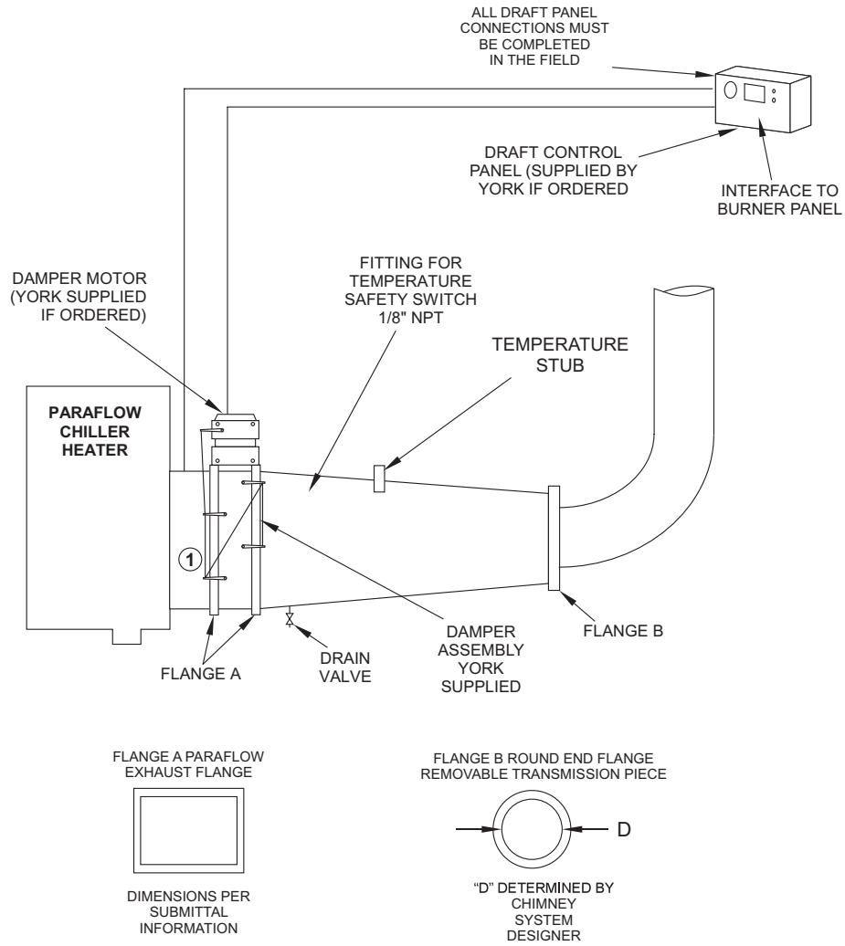
FIGURE 7 - MOTORIZED DRAFT CONTROL
