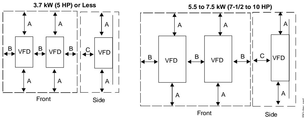
Figure 7: Required Clearance for Mounting Inside an Enclosure
