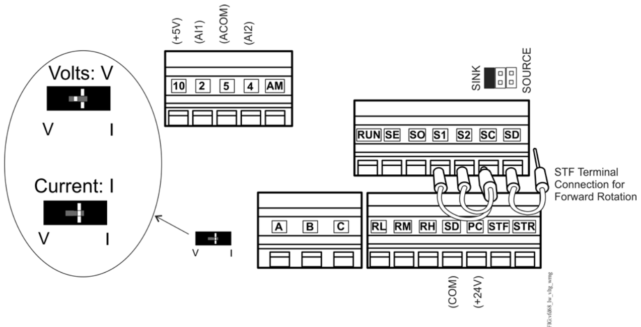
Figure 24: VFD68 Setup and Low-Voltage Connections
