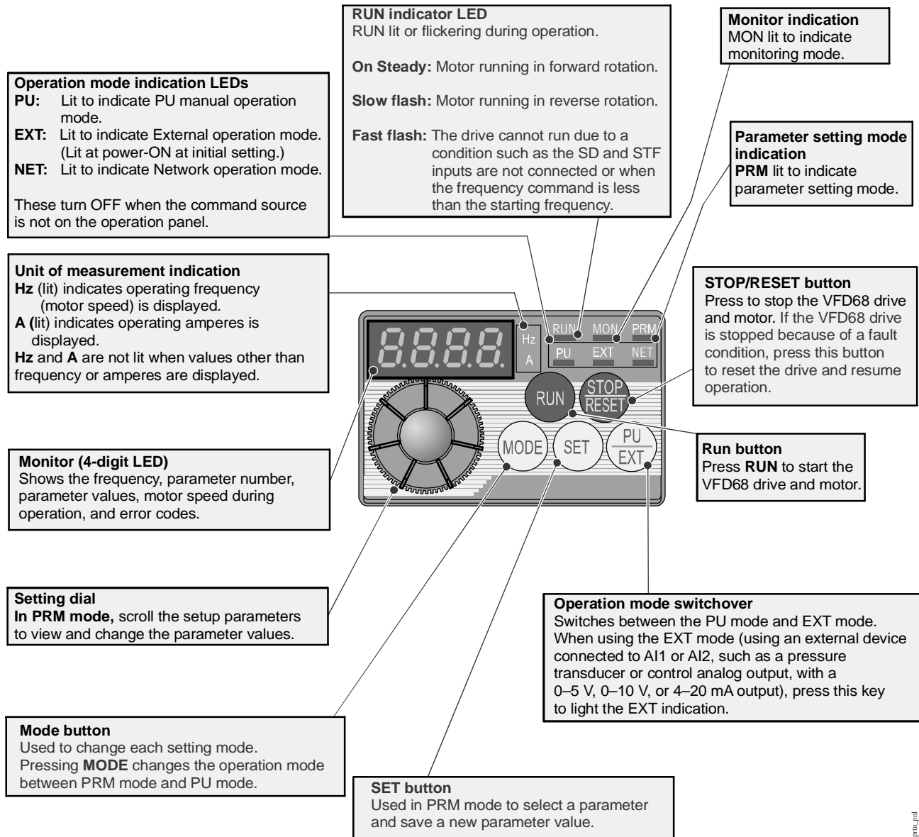
Figure 18: Operation Panel
