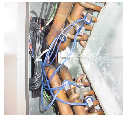
FIG. 18 - ROUTING FREEZESTAT WIRING FROM CONTROL PANEL TO COIL HEADER
