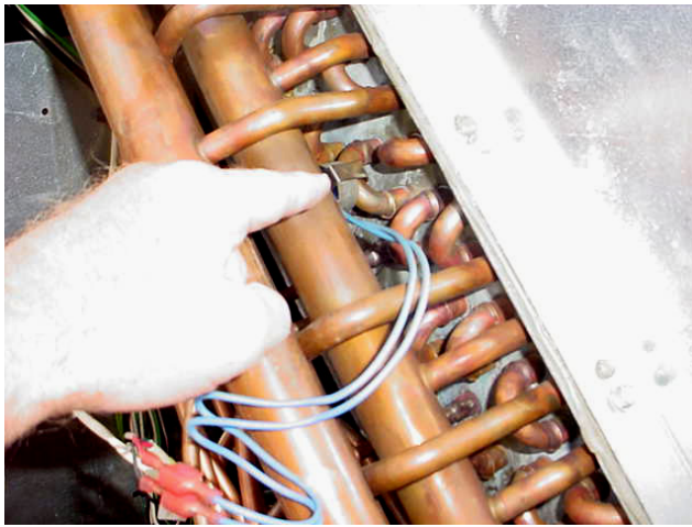
FIG. 19 - EXISTING FREEZESTAT MUST BE REMOVED (CONSTANT VOLUME UNITS ONLY)
