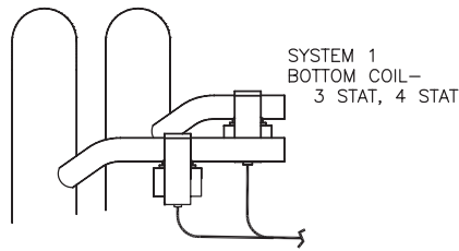
FREEZESTAT DETAIL
