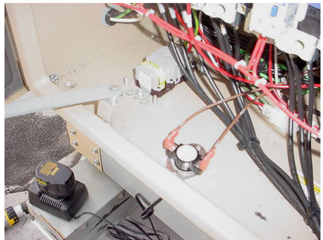
FIG. 24 - INSTALLATION OF OUTDOOR THERMOSTAT
