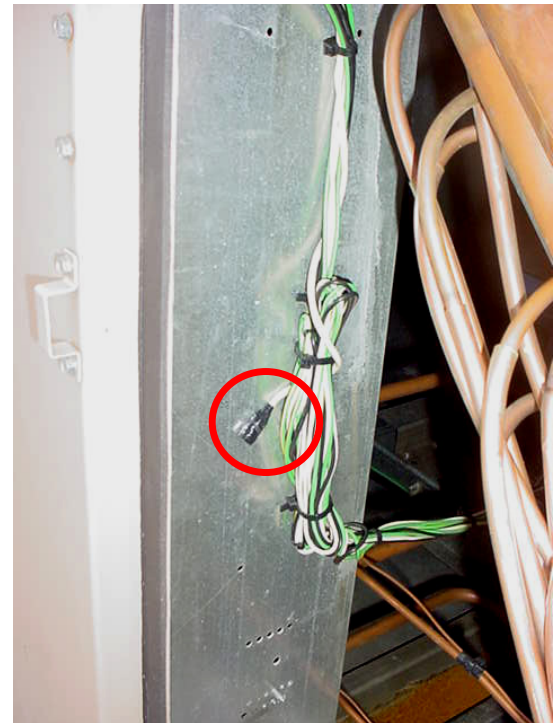
FIG. 20 - REMOVE AND TERMINATE EXISTING FREEZESTAT WIRING (CONSTANT VOLUME UNITS ONLY)
