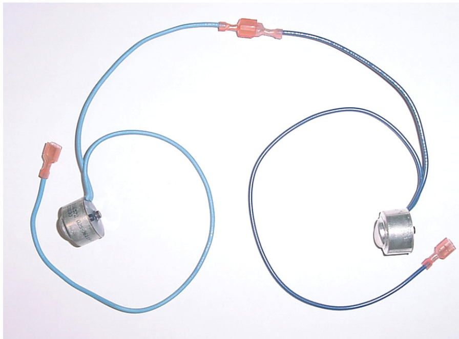
FIG. 21 - FREEZESTAT CONNECTIONS FOR EACH REFRIGERANT SYSTEM
