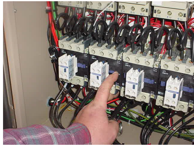
FIG. 14 - ENSURE CONTACTOR/TOP MOUNT AUXILIARY CONTACTS FUNCTION
