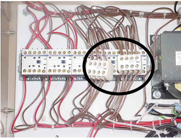
FIG. 9 - 12R & 13R AUXILIARY CONTACT BLOCKS
