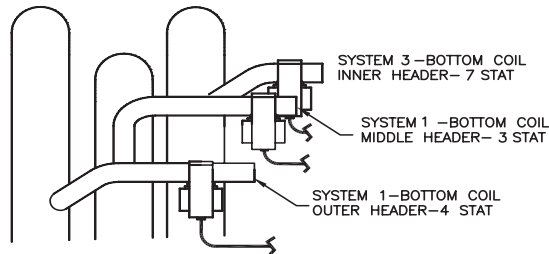
FREEZESTAT DETAIL
