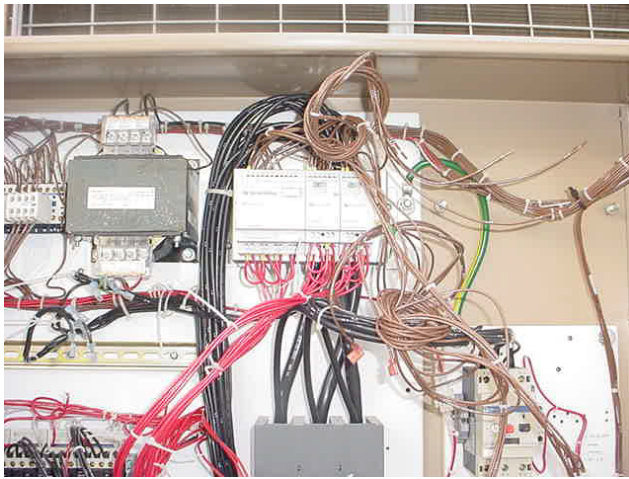
FIG. 6 - LOCATION OF SMART RELAY
