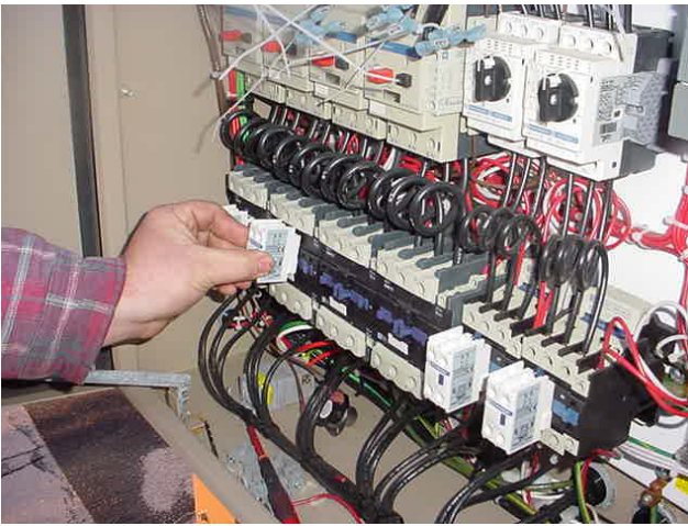
FIG. 13 - INSTALL TOP MOUNT AUXILIARY CONTACTS
