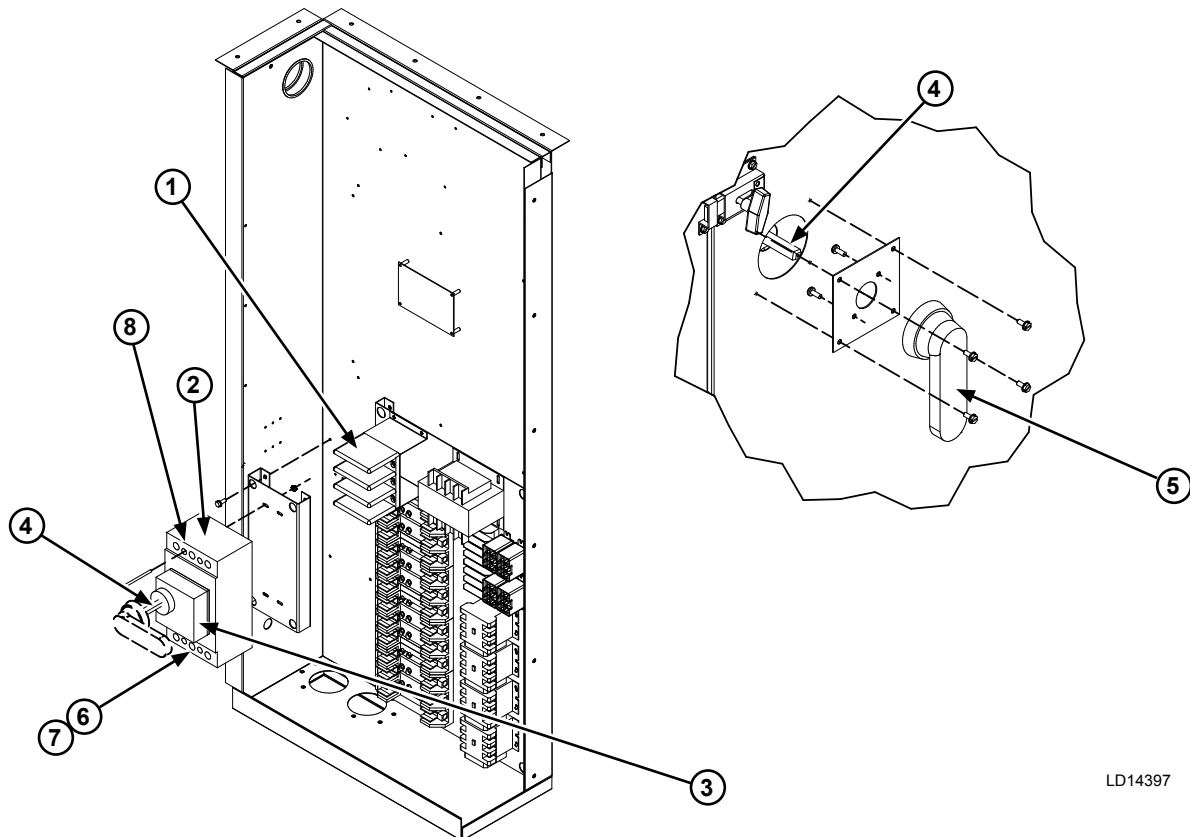
FIG. 37 - SINGLE POINT DISCONNECT SWITCH
