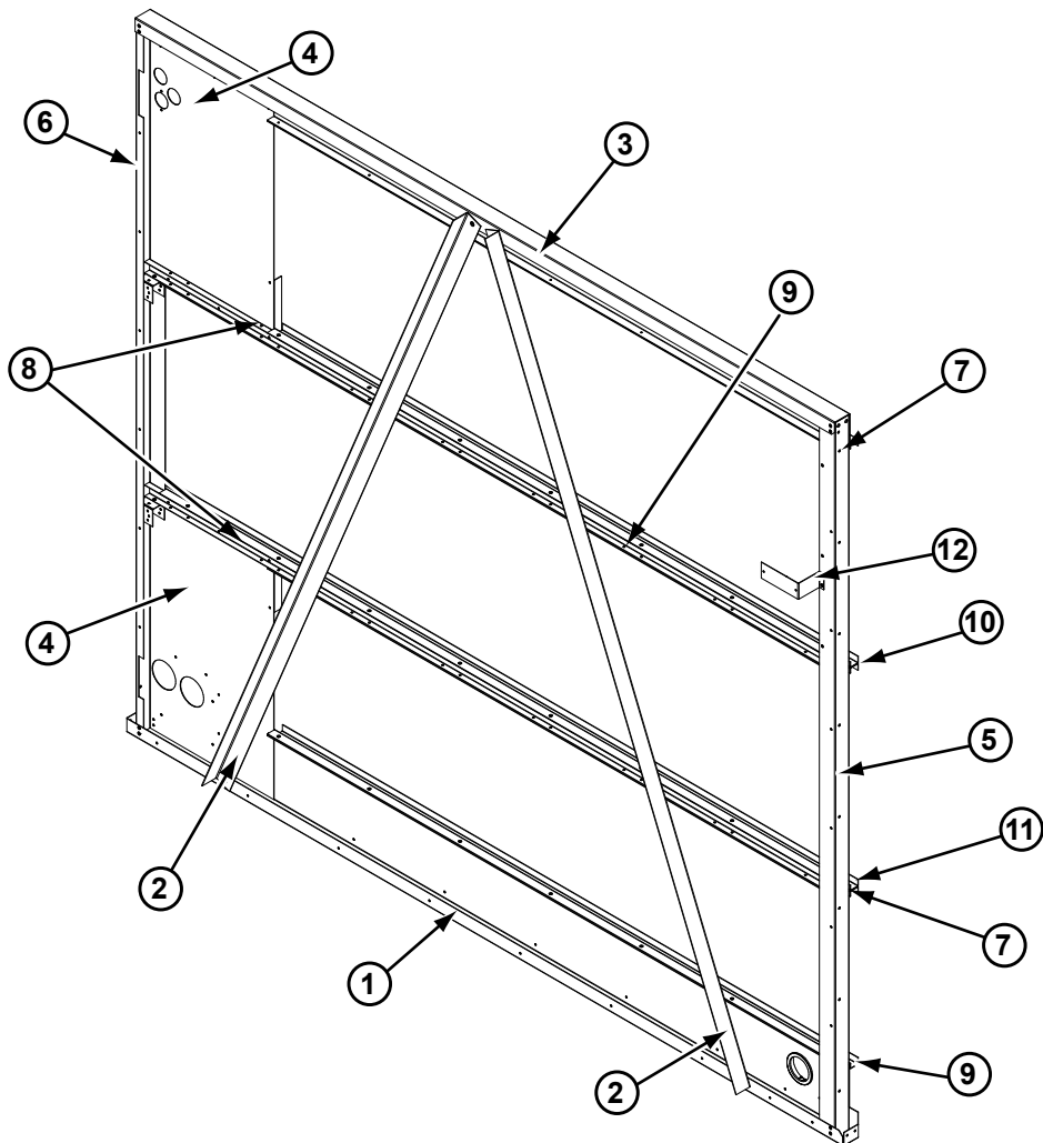
FIG. 48 - EXTENDED CABINET FILTER FRAME
