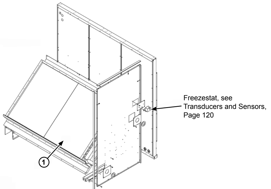
STEAM COIL
