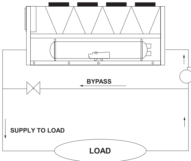
FIGURE 9 - LEAVING LIQUID TEMPERATURE OUT OF RANGE SUGGESTED LAYOUT
