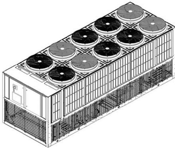
FIGURE 5 - LOUVERED/WIRE PANELS COMBINATION
