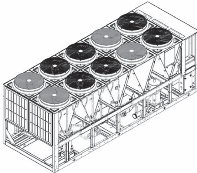
FIGURE 6 - END HAIL GUARD
