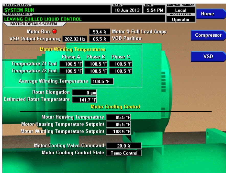
FIGURE 18 - MOTOR DETAILS SCREEN
