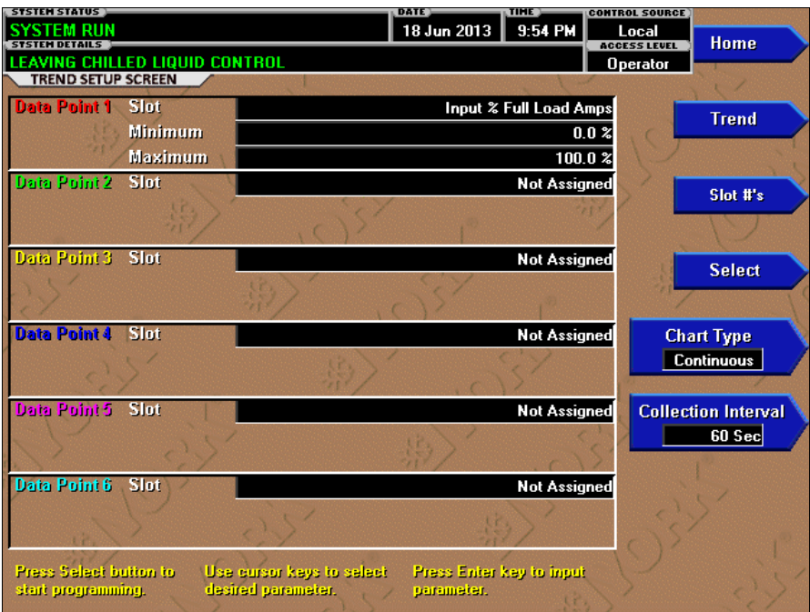
FIGURE 32 - TREND SETUP SCREEN
