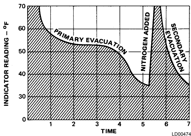
FIGURE 42 - SATURATION CURVE
