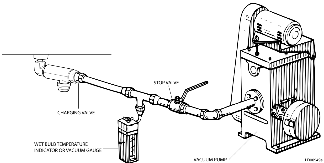
FIGURE 41 - EVACUATION OF CHILLER
