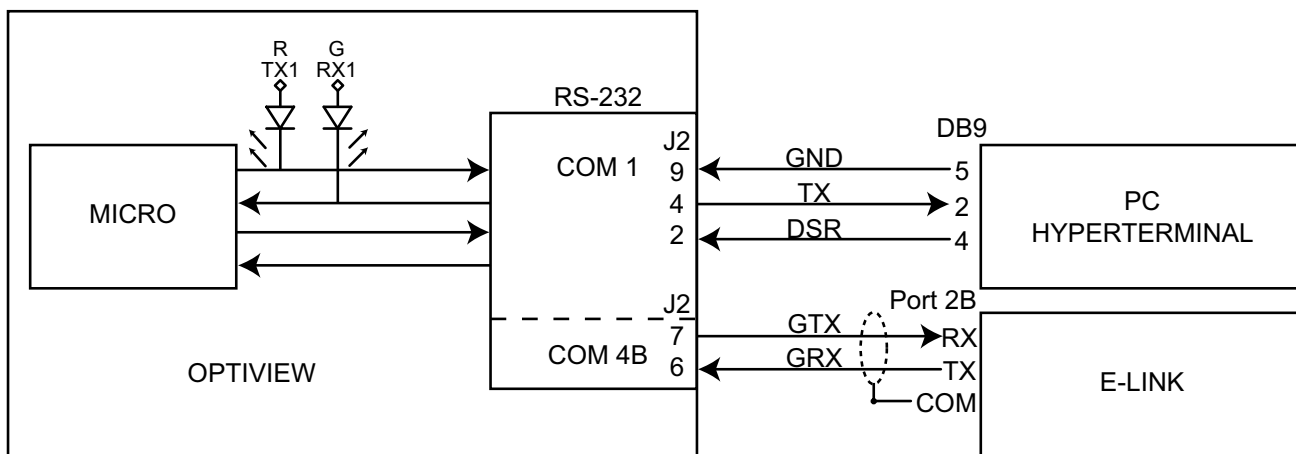
FIGURE 45 - COMMUNICATIONS BLOCK DIAGRAM
