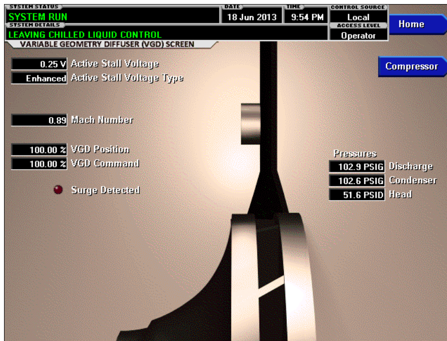
FIGURE 13 - VARIABLE GEOMETRY DIFFUSER SCREEN
