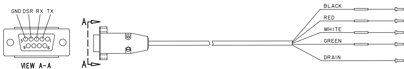
FIGURE 46 - OPTIVIEW PANEL TO PC SERIAL CABLE
