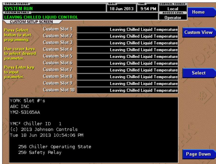
FIGURE 30 - CUSTOM SETUP SCREEN
