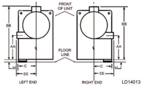
FIGURE 54 - EVAPORATOR - MARINE WATER BOXES (2-PASS NOZZLE ARRANGEMENTS)
