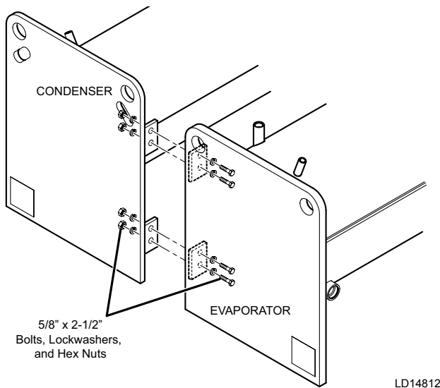
FIGURE 36 - SHELL REASSEMBLY
