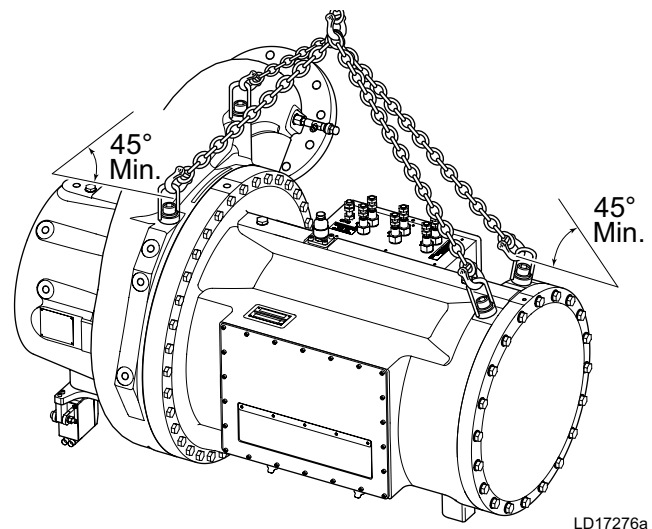
FIGURE 4 - DRIVELINE RIGGING
