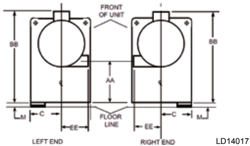
FIGURE 59 - CONDENSER - MARINE WATER BOXES (2-PASS NOZZLE ARRANGEMENTS)
