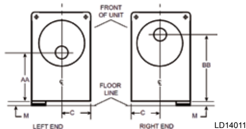
FIGURE 51 - CONDENSER - COMPACT WATER BOXES (2-PASS NOZZLE ARRANGEMENTS)
