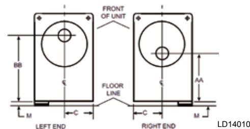
FIGURE 50 - CONDENSER - COMPACT WATER BOXES (3-PASS NOZZLE ARRANGEMENTS)
