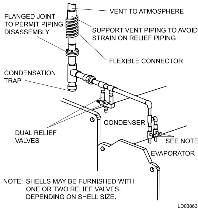
FIGURE 26 - TYPICAL REFRIGERANT VENT PIPING
