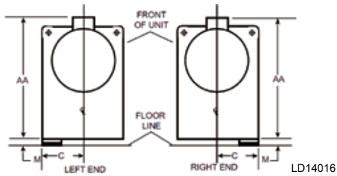
FIGURE 58 - CONDENSER - MARINE WATER BOXES (1-PASS NOZZLE ARRANGEMENTS)
