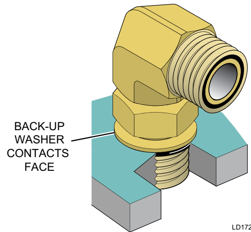
FIGURE 41 - SCREW FITTING INTO PORT
