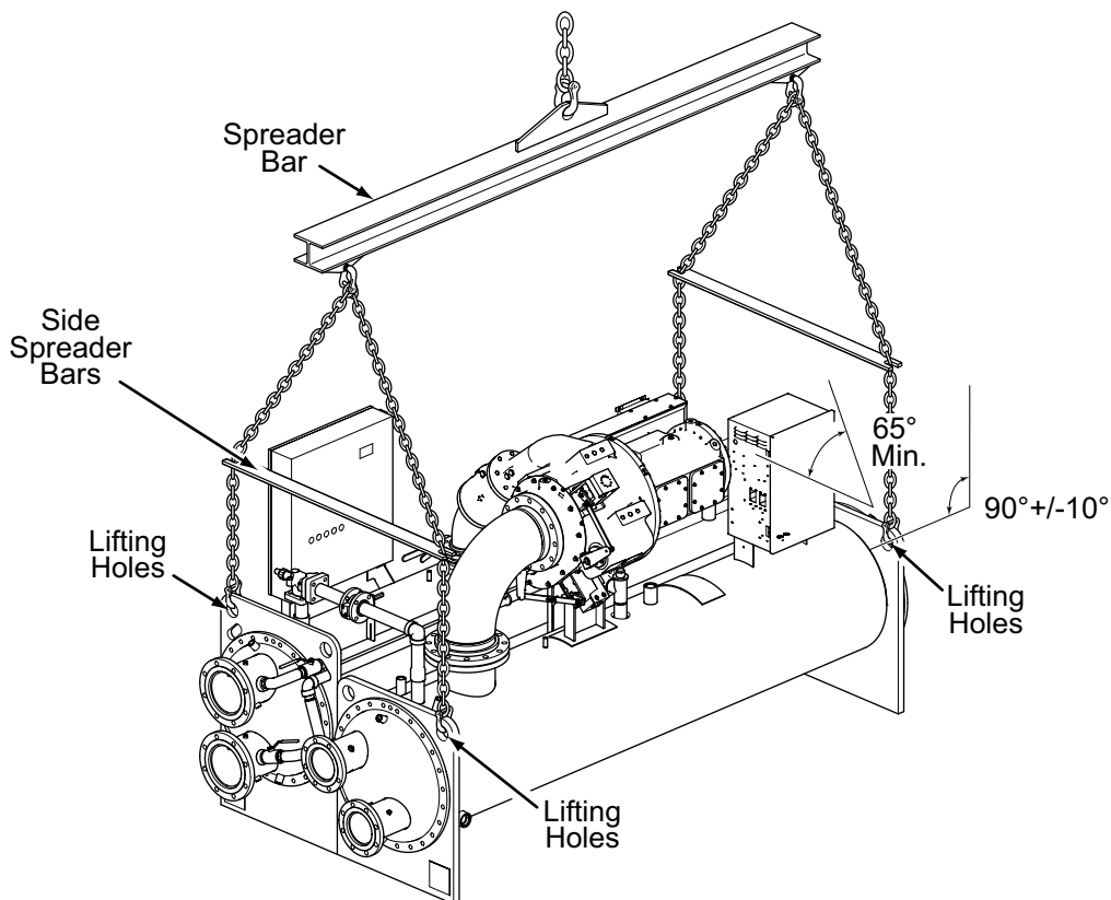
FIGURE 14 - FORM 9 AND 10 RIGGING WITH SIDE SPREADER BARS
