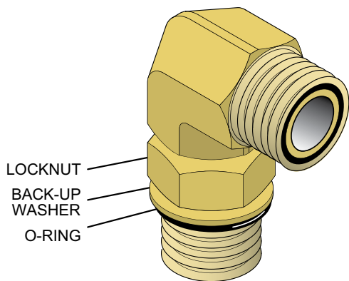
FIGURE 39 - ADJUSTABLE END FITTING
