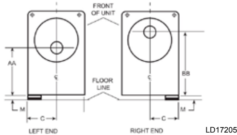
FIGURE 47 - EVAPORATOR - COMPACT WATER BOXES (3-PASS NOZZLE ARRANGEMENTS)
