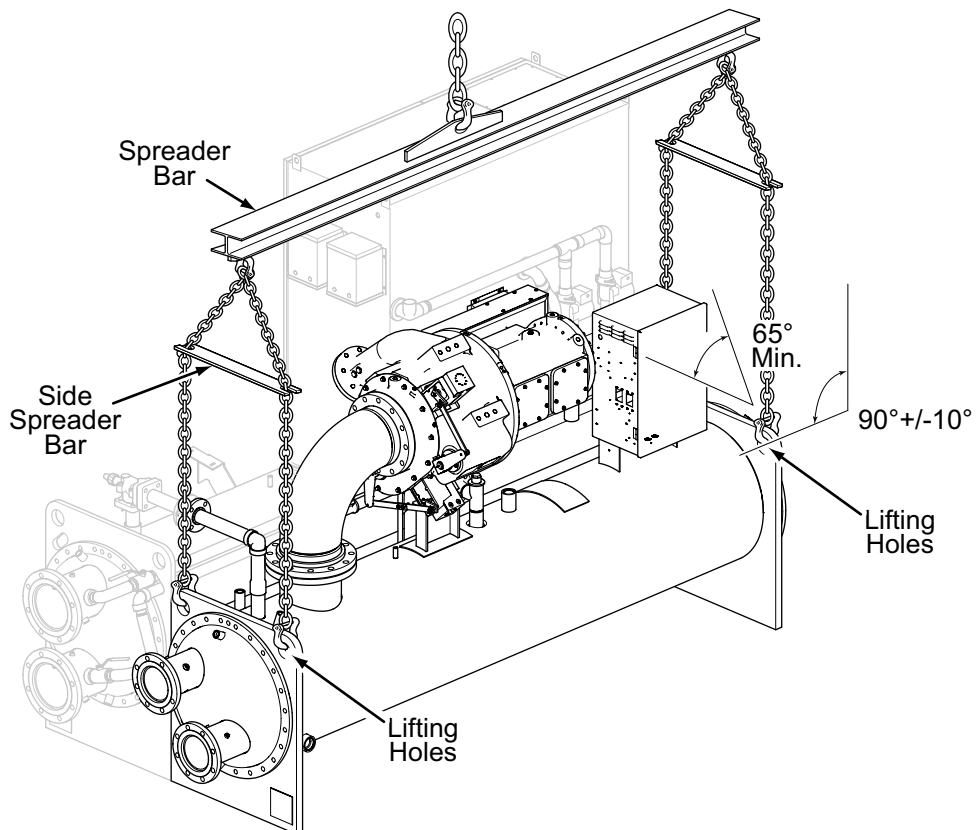
FIGURE 19 - FORM 11 EVAPORATOR ASSEMBLY RIGGING WITH SIDE SPREADER BARS
