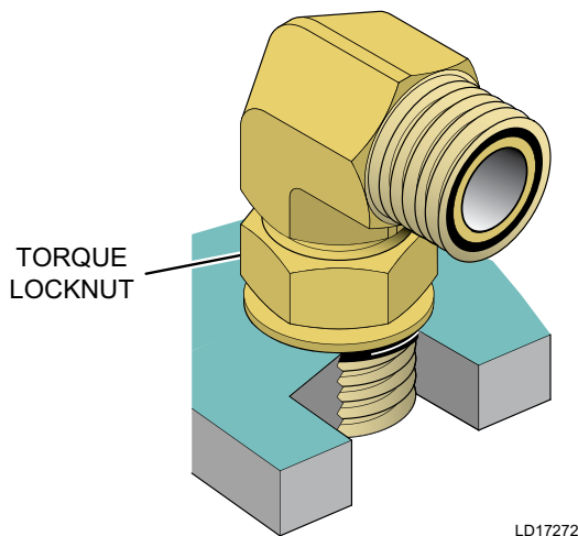
FIGURE 42 - TORQUE FITTING
