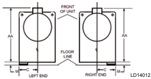
FIGURE 53 - EVAPORATOR - MARINE WATER BOXES (1-PASS NOZZLE ARRANGEMENTS)
