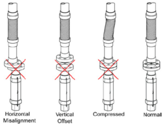
FIGURE 25 - PRESSURE RELIEF PIPING
