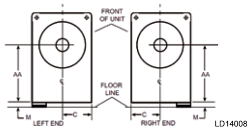
FIGURE 49 - CONDENSER - COMPACT WATER BOXES (1-PASS NOZZLE ARRANGEMENTS)
