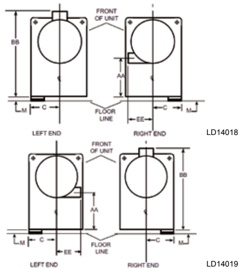
FIGURE 60 - CONDENSER - MARINE WATER BOXES (3-PASS NOZZLE ARRANGEMENTS)
