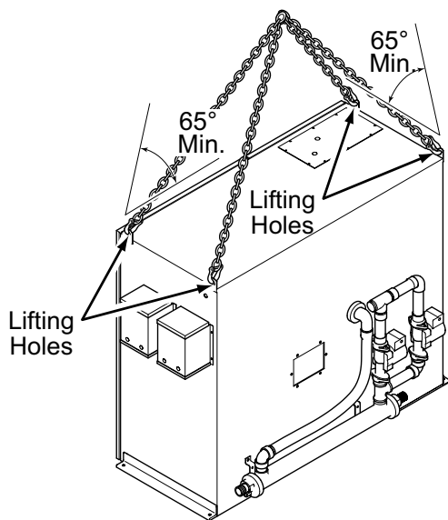
FIGURE 11 - VARIABLE SPEED DRIVE RIGGING
