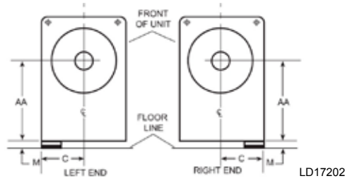
FIGURE 45 - EVAPORATOR - COMPACT WATER BOXES (1-PASS NOZZLE ARRANGEMENTS)
