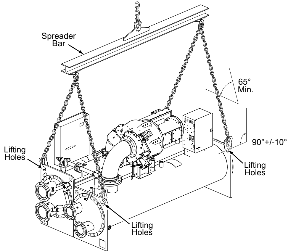
FIGURE 15 - FORM 9 AND 10 RIGGING WITHOUT SIDE SPREADER BARS
