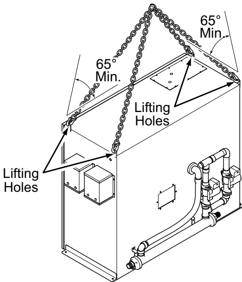
FIGURE 16 - VARIABLE SPEED DRIVE RIGGING
