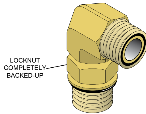
FIGURE 40 - BACK OFF LOCKNUT
