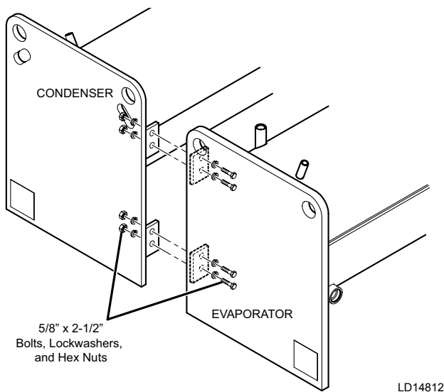
FIGURE 29 - SHELL REASSEMBLY
