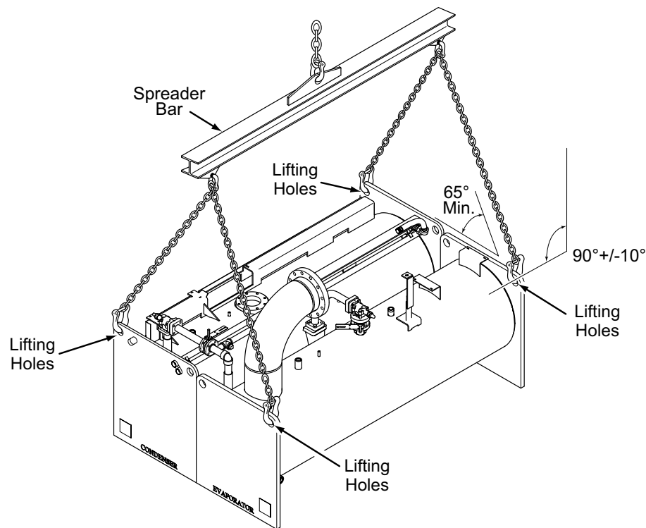
FIGURE 5 - FORM 3 RIGGING WITHOUT SIDE SPREADER BARS
