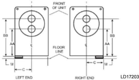
FIGURE 46 - EVAPORATOR - COMPACT WATER BOXES (2-PASS NOZZLE ARRANGEMENTS)
