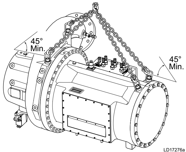
FIGURE 10 - DRIVELINE RIGGING
