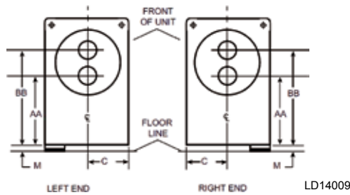
FIGURE 50 - CONDENSER - COMPACT WATER BOXES (3-PASS NOZZLE ARRANGEMENTS)
