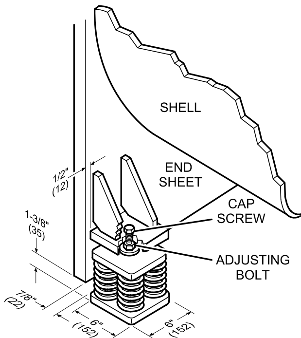
4-SPRING ISOLATORS
