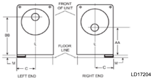
FIGURE 46 - EVAPORATOR - COMPACT WATER BOXES (2-PASS NOZZLE ARRANGEMENTS)
