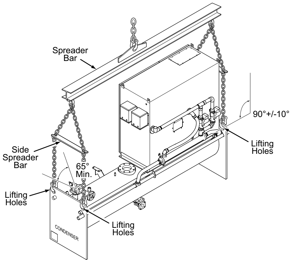
FIGURE 18 - FORM 11 CONDENSER ASSEMBLY RIGGING WITH SIDE SPREADER BARS
