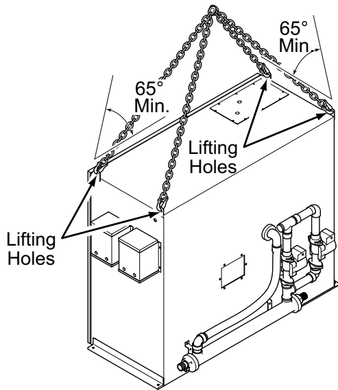
FIGURE 17 - VARIABLE SPEED DRIVE RIGGING
