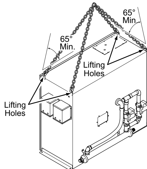
FIGURE 6 - VARIABLE SPEED DRIVE RIGGING
