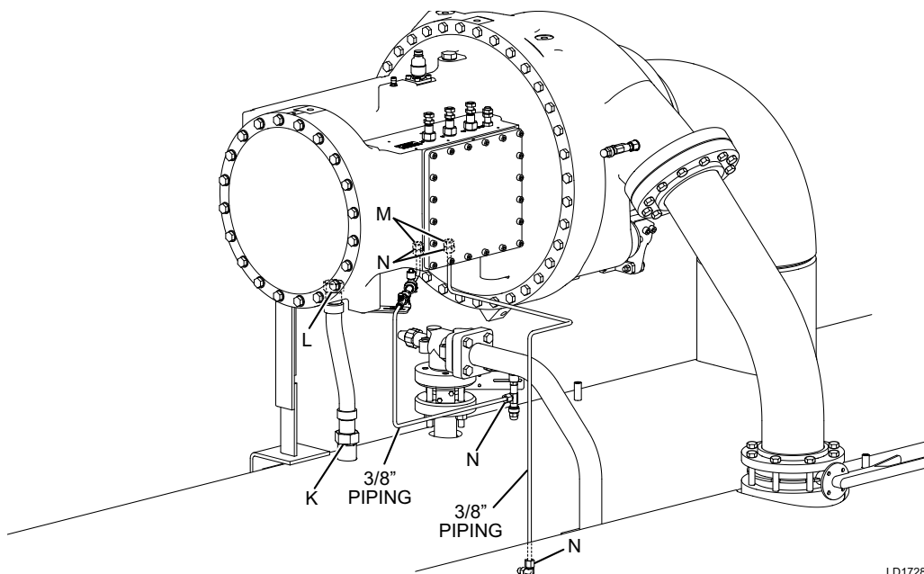
FIGURE 30 - YMC 2 PIPING REASSEMBLY HARDWARE IDENTIFICATION
