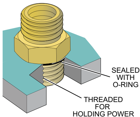
FIGURE 43 - SAE OR ISO 6149 STRAIGHT THREAD O-RING PORT
