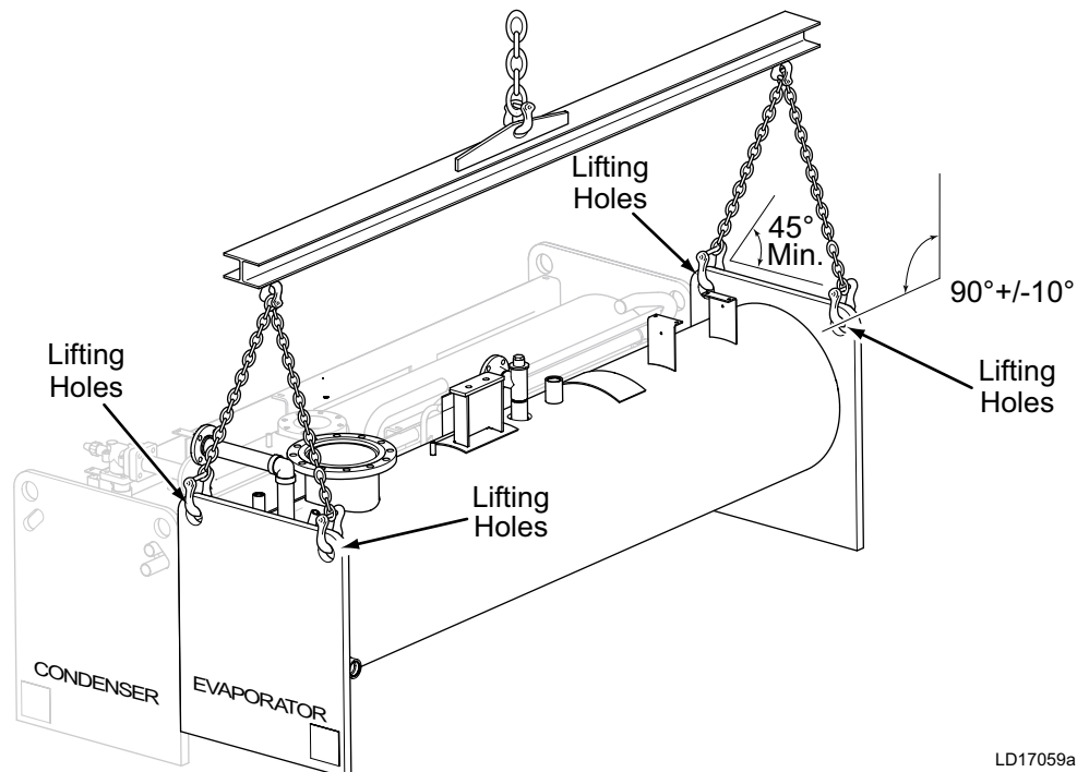
FIGURE 9 - FORM 7 RIGGING WITH SIDE SPREADER BARS
