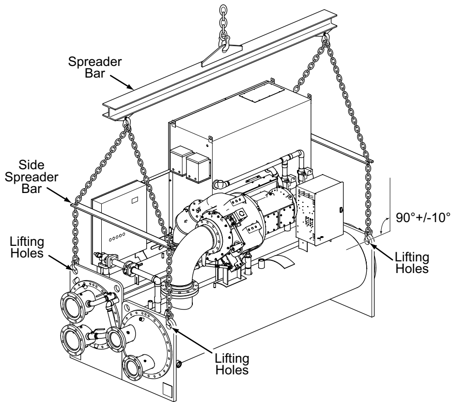
FIGURE 2 - FORM 1 AND 2 RIGGING WITH SIDE SPREADER BAR
