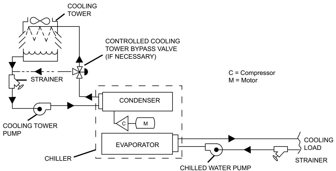
FIGURE 27 - SCHEMATIC OF A TYPICAL PIPING ARRANGEMENT
