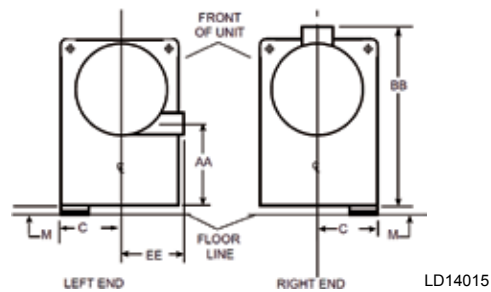
FIGURE 55 - EVAPORATOR - MARINE WATER BOXES (3-PASS NOZZLE ARRANGEMENTS)
