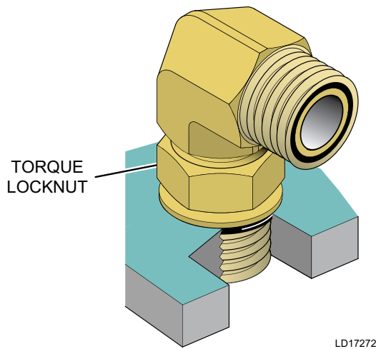
FIGURE 41 - TORQUE FITTING
