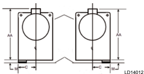
FIGURE 52 - EVAPORATOR - MARINE WATER BOXES (1-PASS NOZZLE ARRANGEMENTS)
