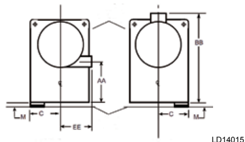
FIGURE 54 - EVAPORATOR - MARINE WATER BOXES (3-PASS NOZZLE ARRANGEMENTS)
