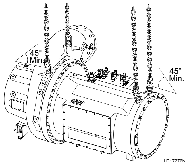
FIGURE 4 - DRIVELINE RIGGING
