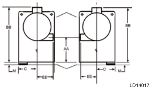
FIGURE 58 - CONDENSER - MARINE WATER BOXES (2-PASS NOZZLE ARRANGEMENTS)
