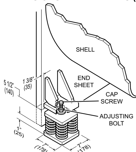
4-SPRING ISOLATORS
