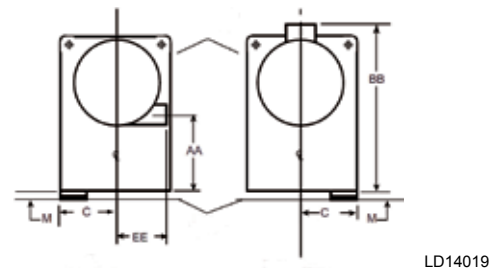
FIGURE 59 - CONDENSER - MARINE WATER BOXES (3-PASS NOZZLE ARRANGEMENTS)
