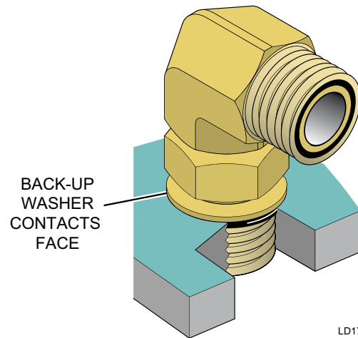
FIGURE 40 - SCREW FITTING INTO PORT
