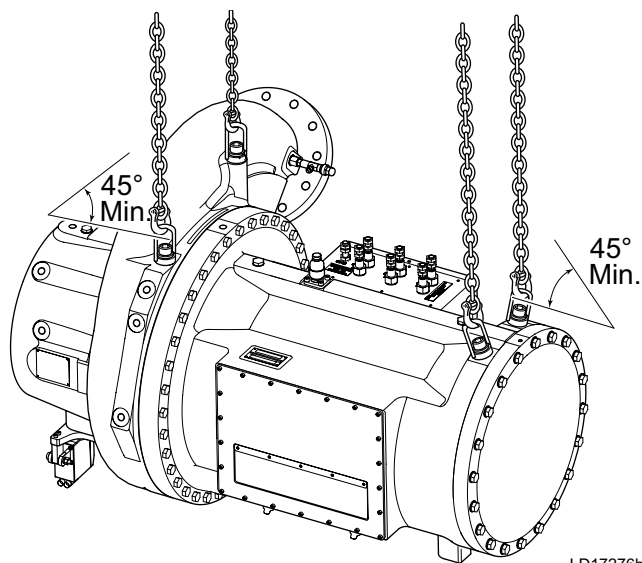
FIGURE 10 - DRIVELINE RIGGING
