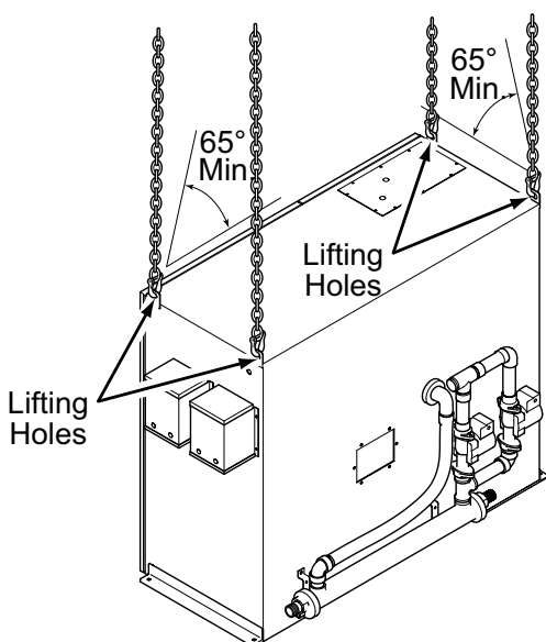
FIGURE 16 - VARIABLE SPEED DRIVE RIGGING
