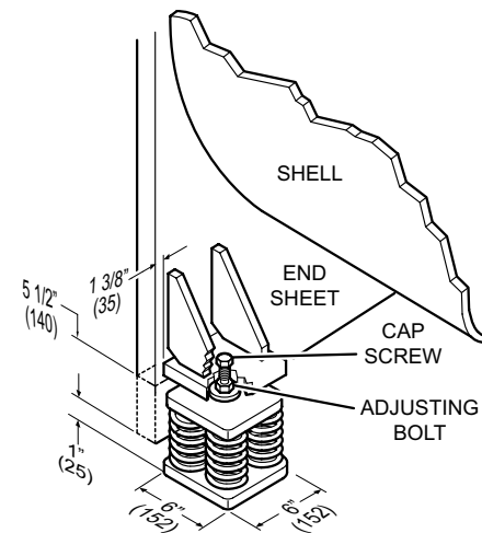
4-SPRING ISOLATORS
