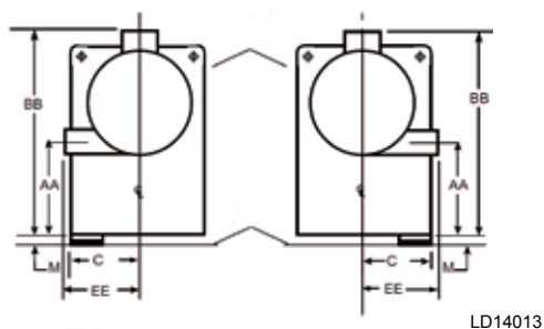
FIGURE 53 - EVAPORATOR - MARINE WATER BOXES (2-PASS NOZZLE ARRANGEMENTS)
