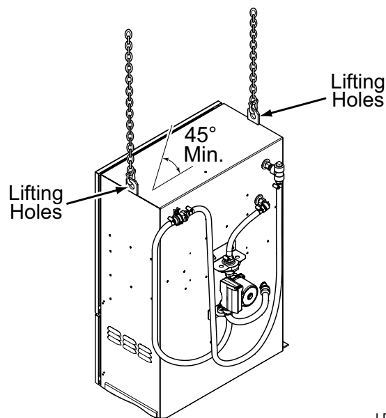
FIGURE 12 - POWER PANEL
