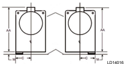
FIGURE 57 - CONDENSER - MARINE WATER BOXES (1-PASS NOZZLE ARRANGEMENTS)
