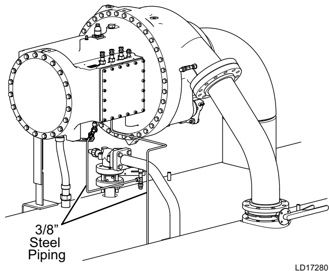
FIGURE 36 - REFRIGERANT PIPING
