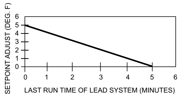
FIGURE 24 - SETPOINT ADJUST
