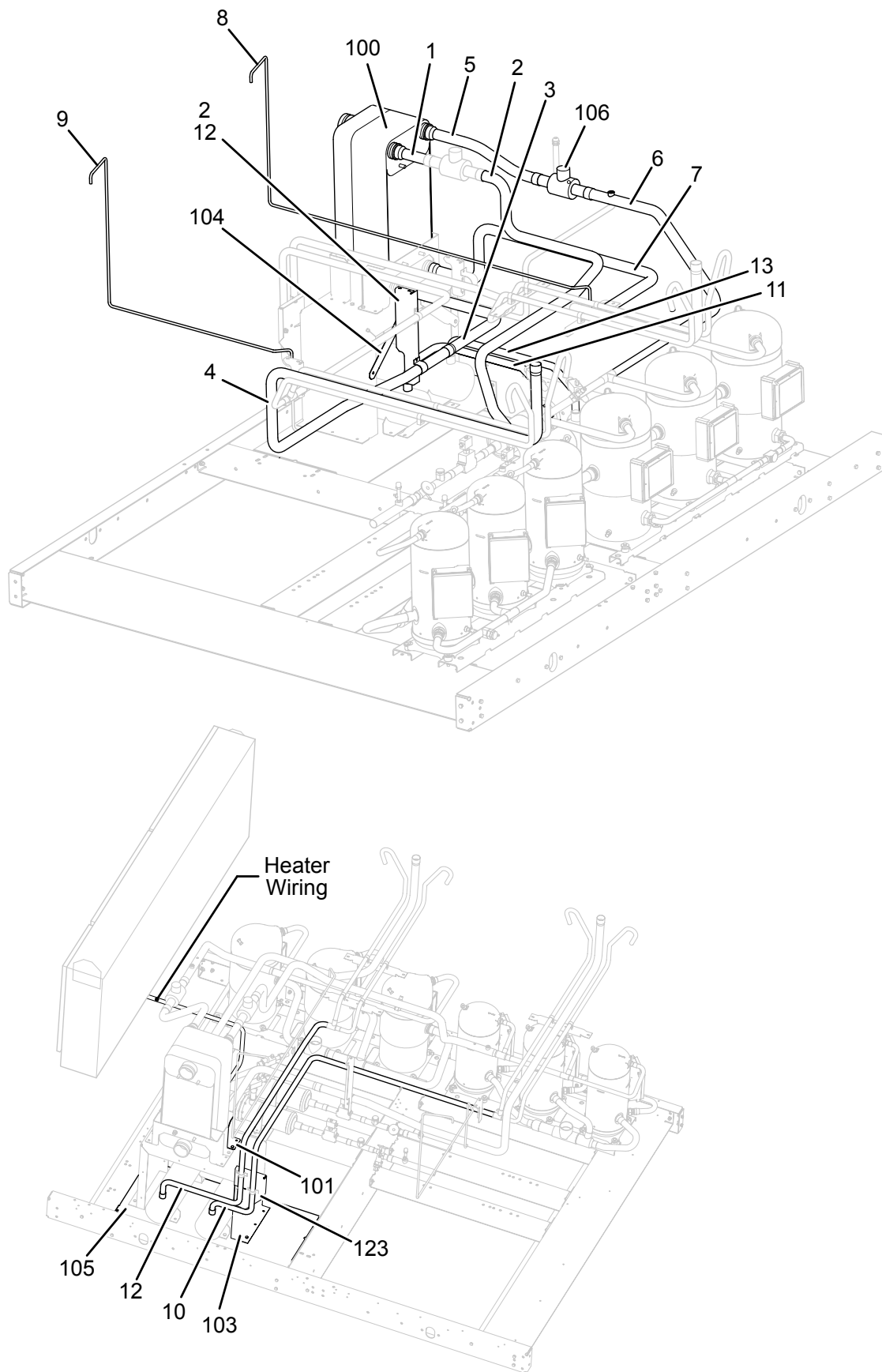
FIGURE 23 - HEAT RECOVERY ASSEMBLY (YLA0070 - YLA0090)
