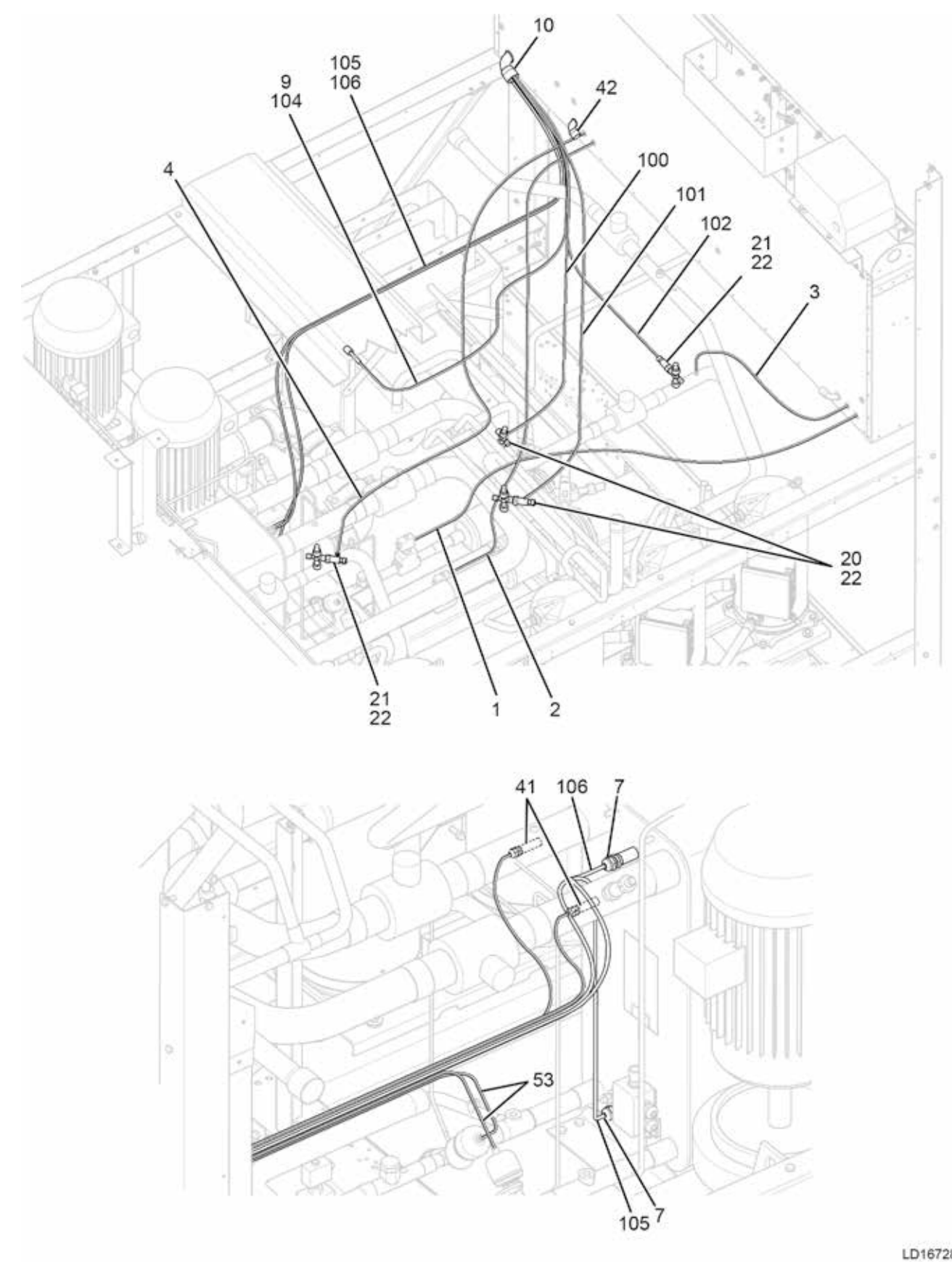
FIGURE 11 - SYSTEM WIRING
