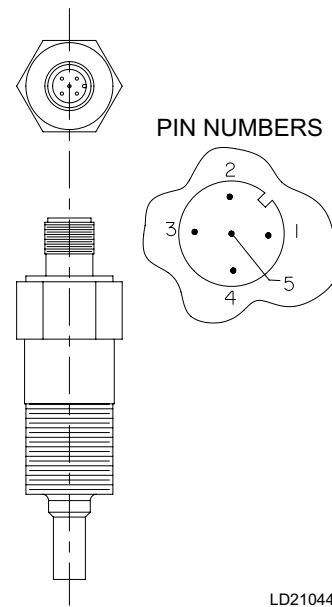
FIGURE 11 - THERMAL DISPERSION FLOW SWITCH
