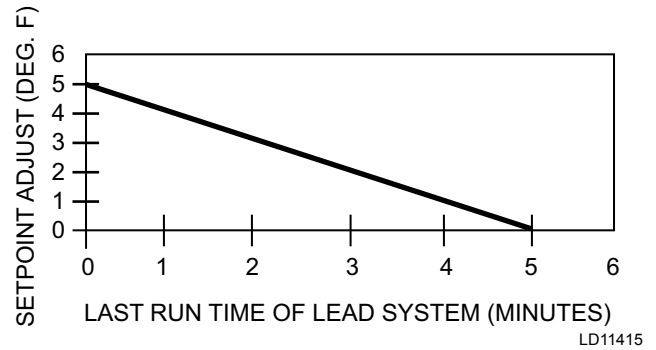
FIGURE 39 - SETPOINT ADJUST
