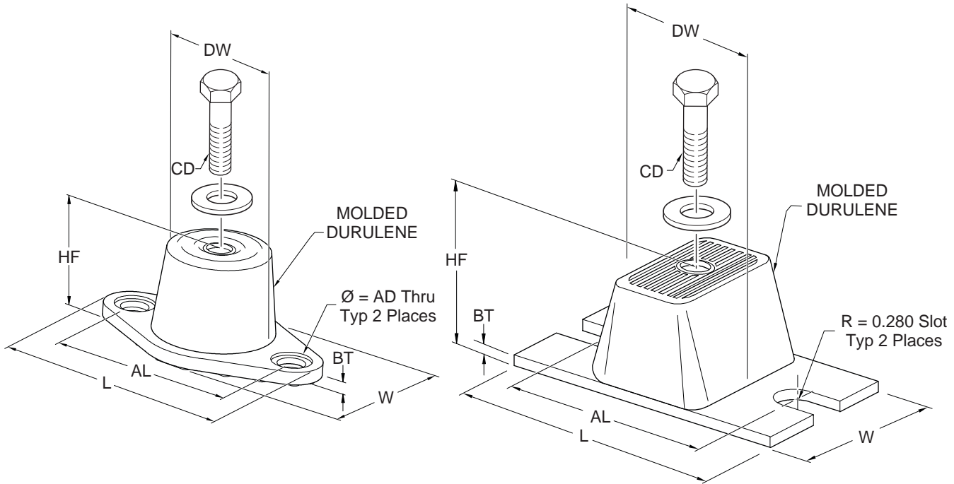
RD3 ISOLATORS
