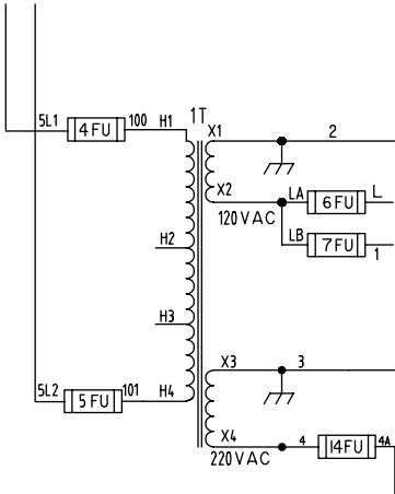
FIGURE 14 - TRANSFORMER WIRING ASIA DESIGN
