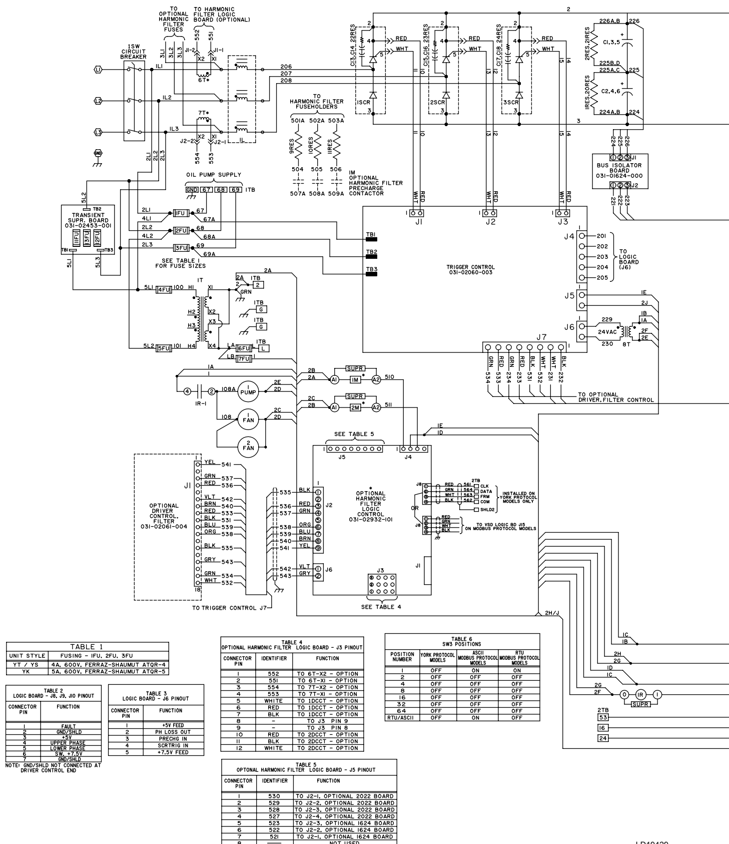
FIGURE 6 - ELEMENTARY WIRING DIAGRAM 424 HP FOR VSD MODELS GLOBAL DESIGN MANUFACTURED AFTER DECEMBER 2006
