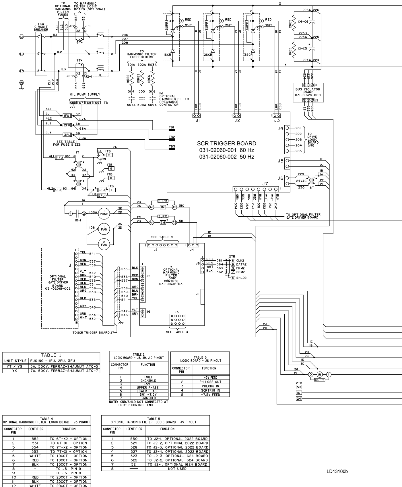
FIGURE 5 - ELEMENTARY WIRING DIAGRAM 270, 292 AND 351 HP FOR VSD MODELS GLOBAL DESIGN MANUFACTURED BEFORE DECEMBER 2006
