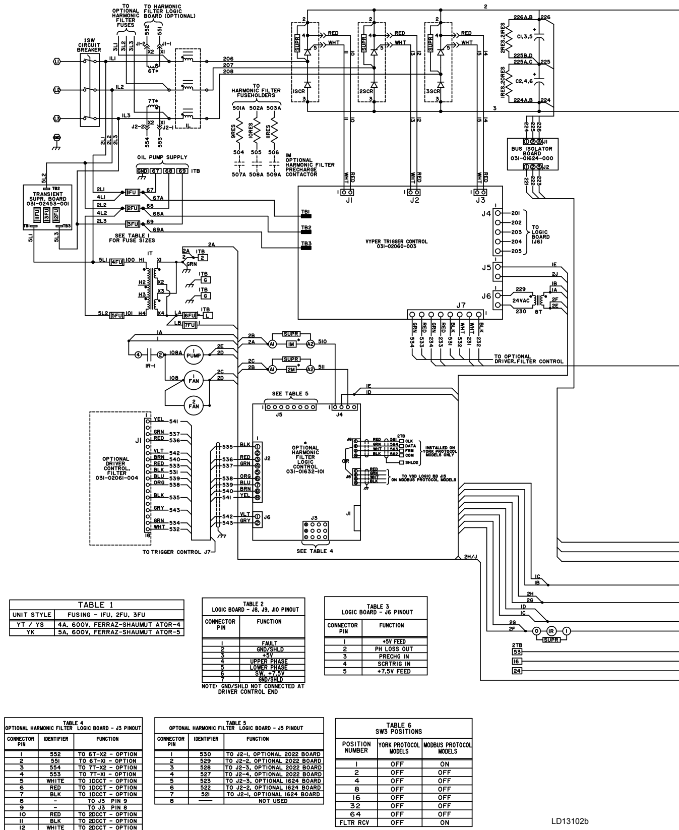
FIGURE 7 - ELEMENTARY WIRING DIAGRAM 424 HP FOR VSD MODELS GLOBAL DESIGN MANUFACTURED BEFORE DECEMBER 2006
