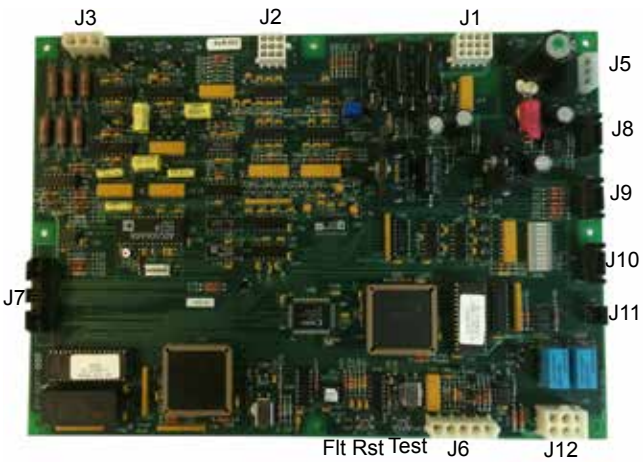
FIGURE 1 - VSD MODEL DRIVE LOGIC BOARD 031-02077-000,031-02077-001
