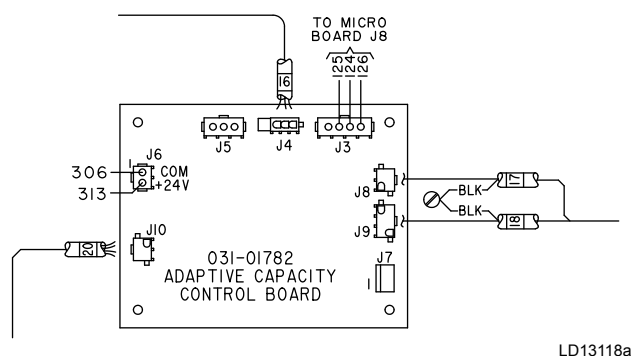
FIGURE 39 - ADAPTIVE CAPACITY CONTROL BOARD FOR OPTIVIEW CONTROL CENTER
