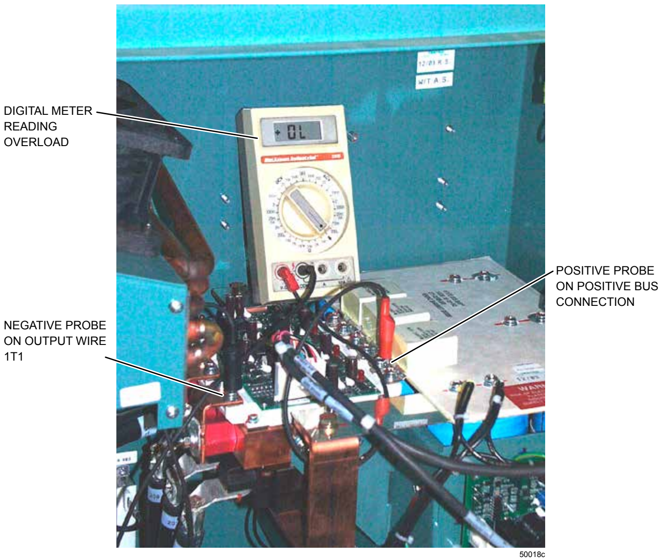
FIGURE 43 - 270/292/351/424 HP DRIVE IGBT MODULE VERIFICATION #3.
