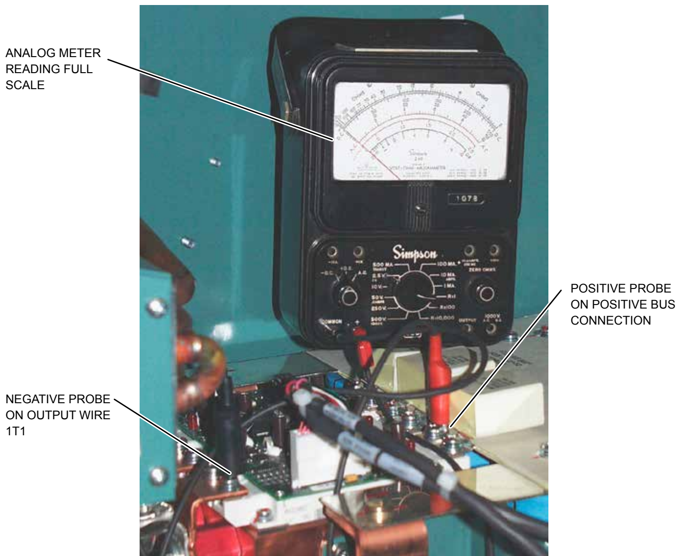
FIGURE 42 - 270/292/351/424 HP DRIVE IGBT MODULE VERIFICATION #2.
