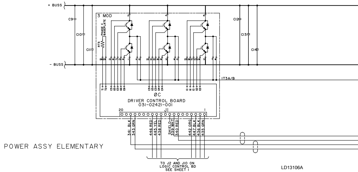
FIGURE 12 - POWER ASSEMBLY ELEMENTARY WIRING DIAGRAM 385/419/503 HP FOR VSD MODELS GLOBAL DESIGN
