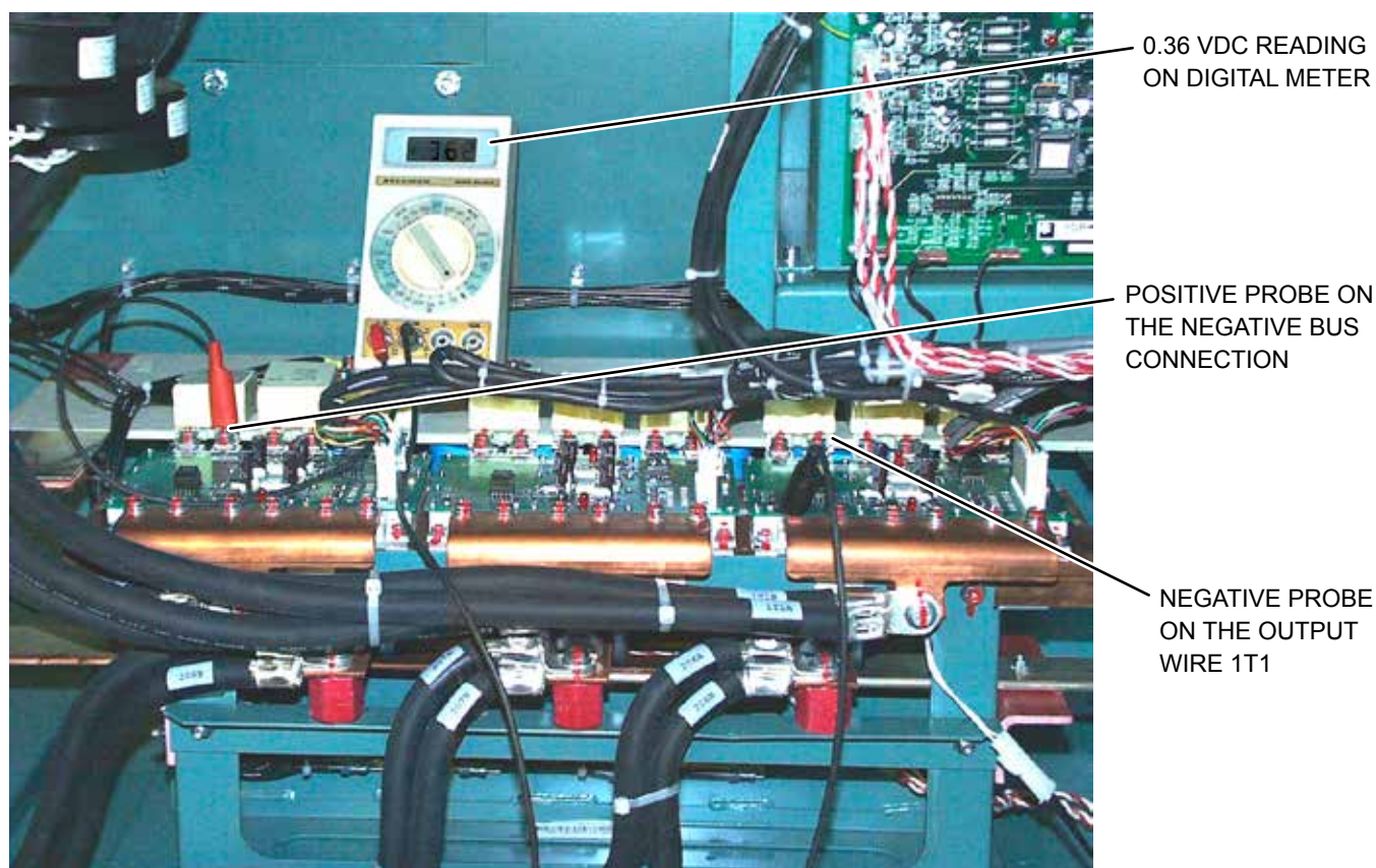
FIGURE 46 - 385/419/503/608/658/704/900 HP DRIVE IGBT MODULE VERIFICATION #3
