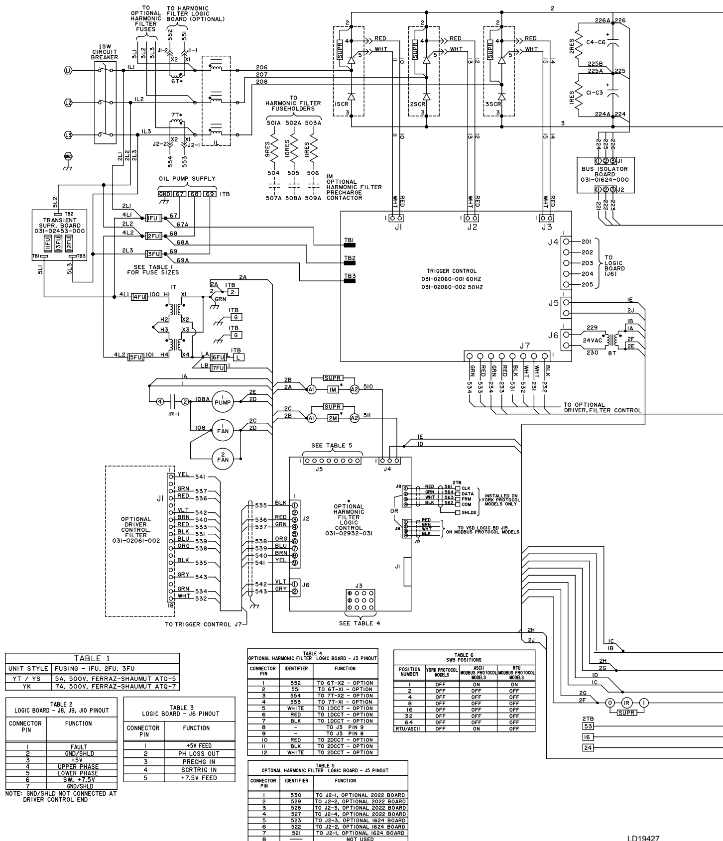
FIGURE 4 - ELEMENTARY WIRING DIAGRAM 270, 292 AND 351 HP FOR VSD MODELS GLOBAL DESIGN MANUFACTURED AFTER DECEMBER 2006
