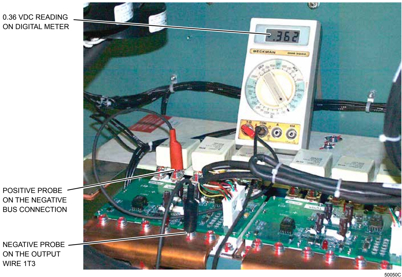
FIGURE 45 - 385/419/503/608/658/704/900 HP DRIVE IGBT MODULE VERIFICATION #2
