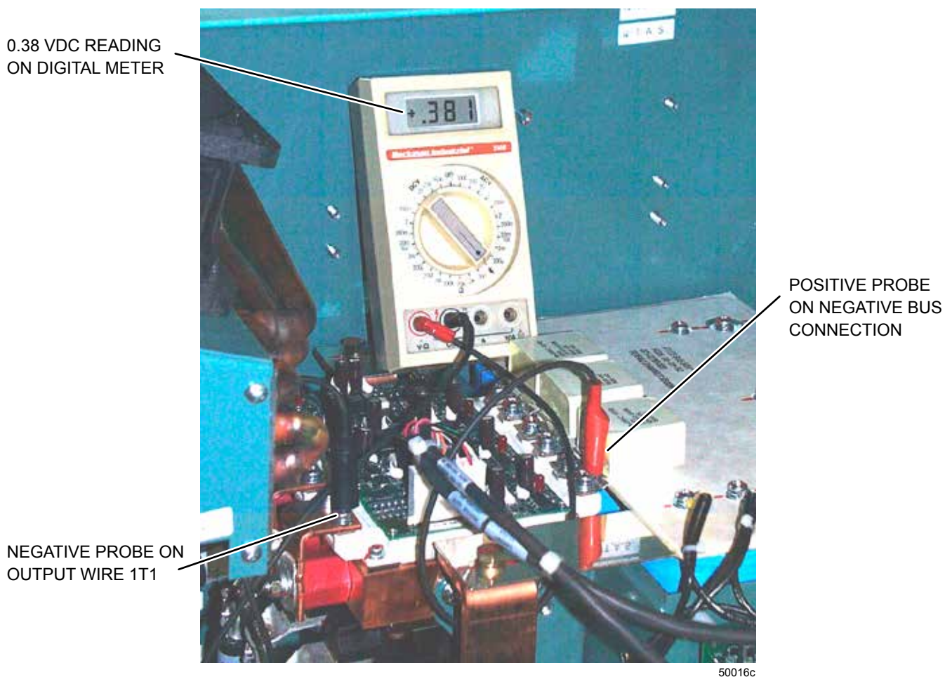
FIGURE 41 - 270/292/351/424 HP DRIVE IGBT MODULE VERIFICATION #1
