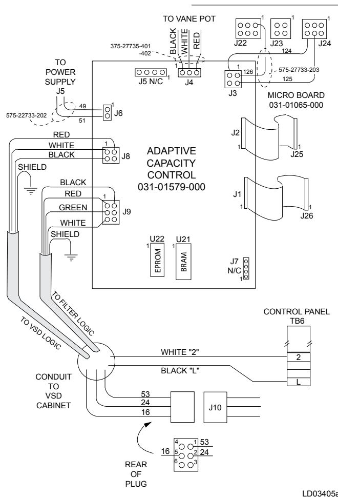
FIGURE 40 - ADAPTIVE CAPACITY CONTROL BOARD
