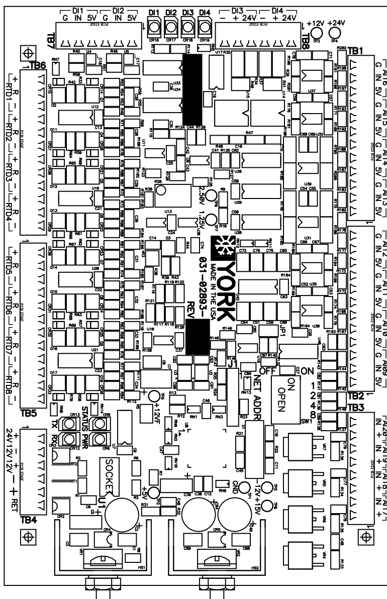
FIGURE 98 - MOTOR MONITORING BOARD (031-02893-000/001)
