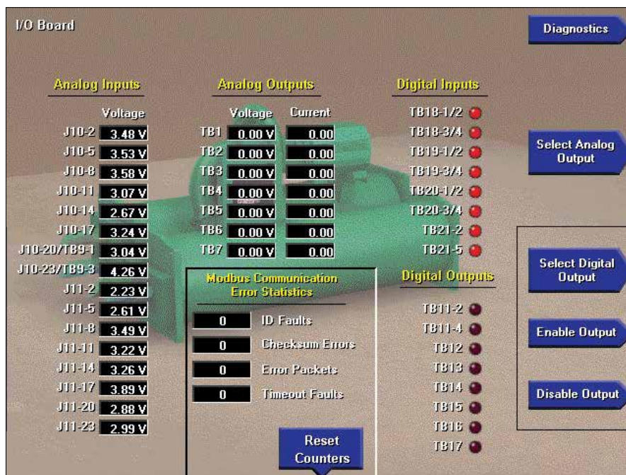
FIGURE 110 - I/O BOARD DIAGNOSTIC SCREEN
