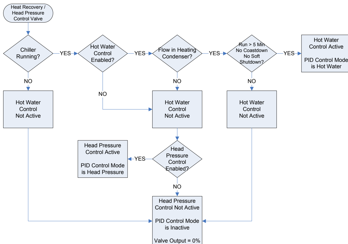
FIGURE 94 - HEAT RECOVERY FLOW DIAGRAM
