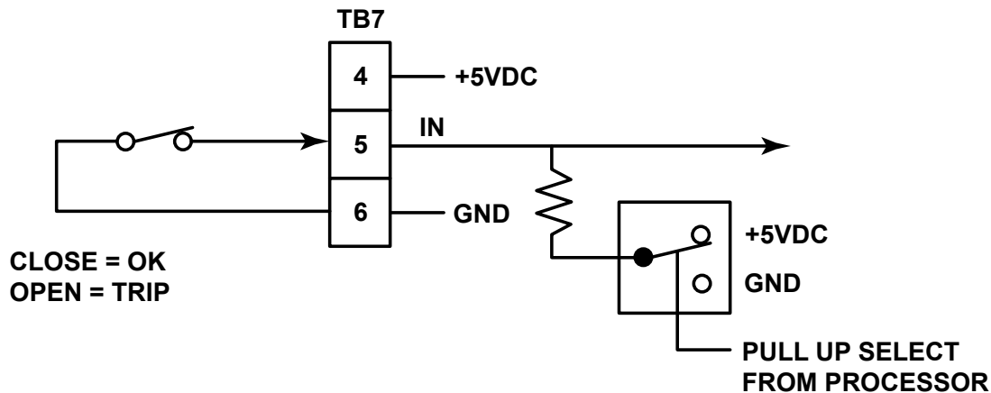
FIGURE 105 - MOTOR COOLING COIL LEAK DETECTOR – OPTICAL SENSOR
