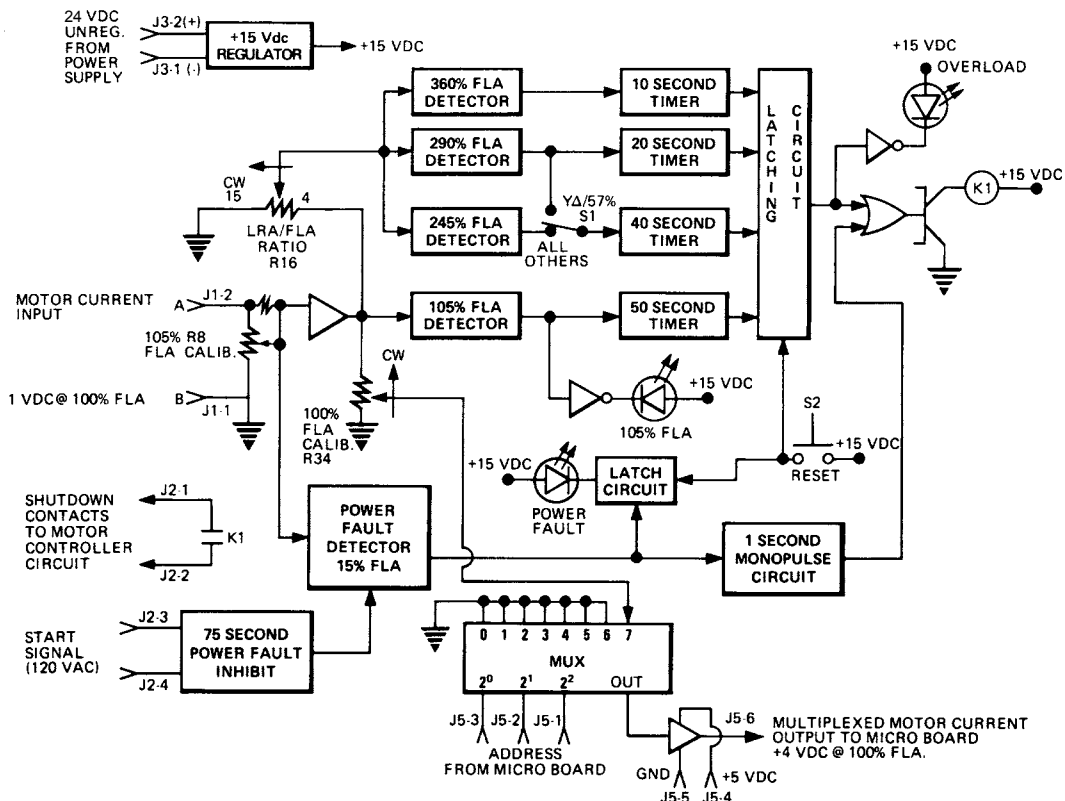
FIGURE 55 - CM-2 CURRENT MODULE (ELECTRO-MECHANICAL STARTER APPLICATIONS)
