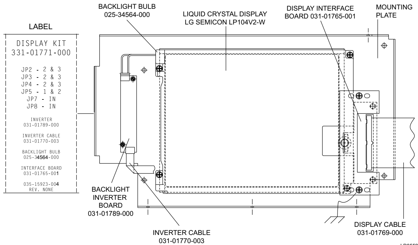
FIGURE 41 - LIQUID CRYSTAL DISPLAY ASSEMBLY – LG SEMICON LP104V2-W (031-02046-000)
