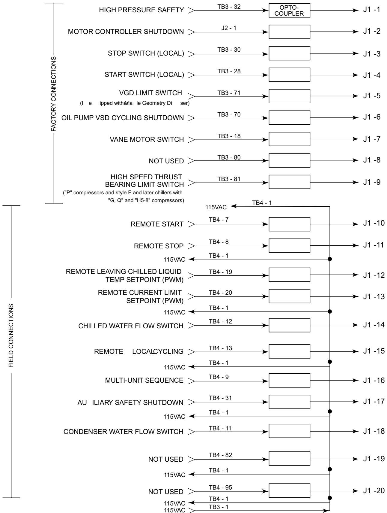
FIGURE 34 - I/O BOARD DIGITAL INPUTS
