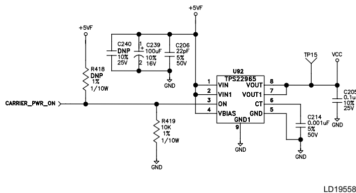
FIGURE 27 - MICROBOARD (031-03630-001)DC POWER SUPPLY TEST POINTS
