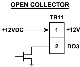
FIGURE 88 - OPEN COLLECTOR
