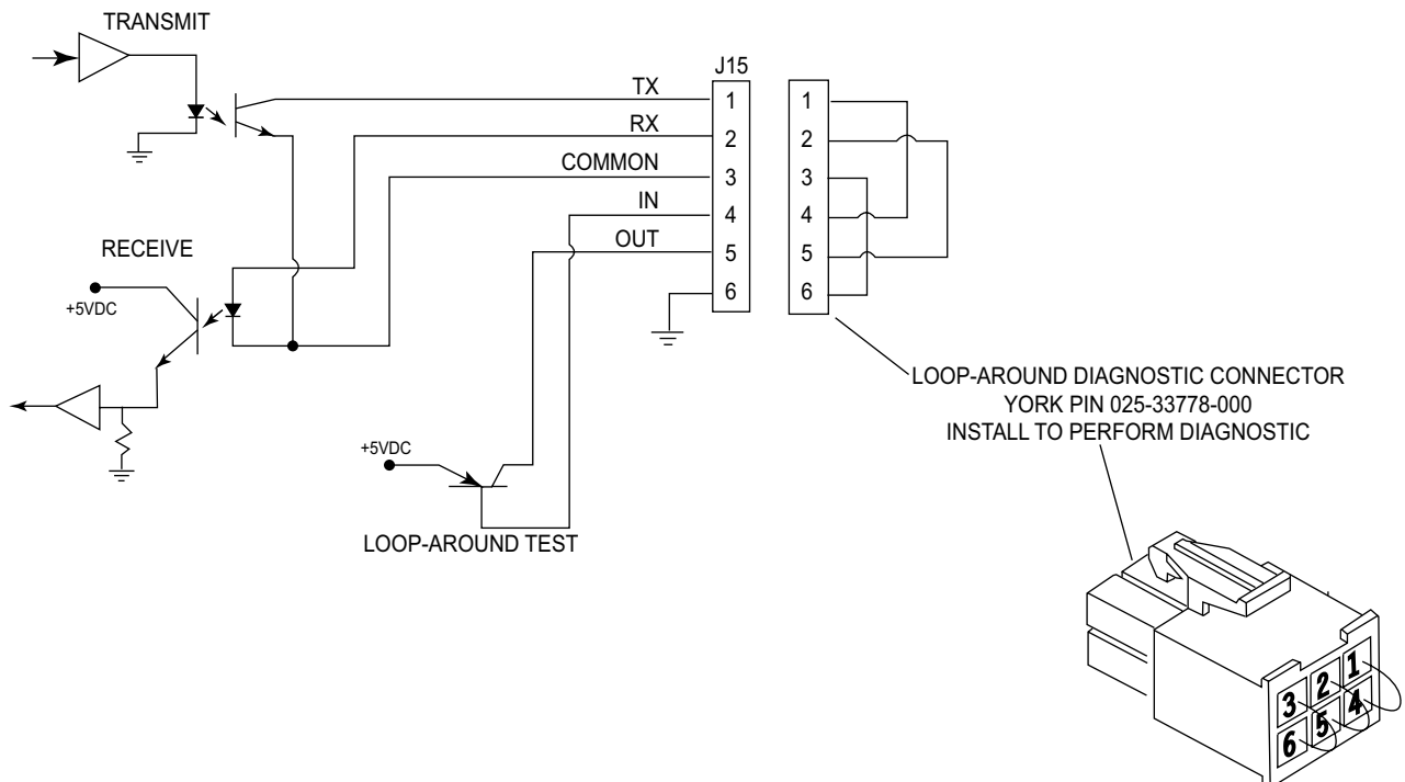
FIGURE 115 - MICROBOARD - COM 5 SERIAL DATA PORT
