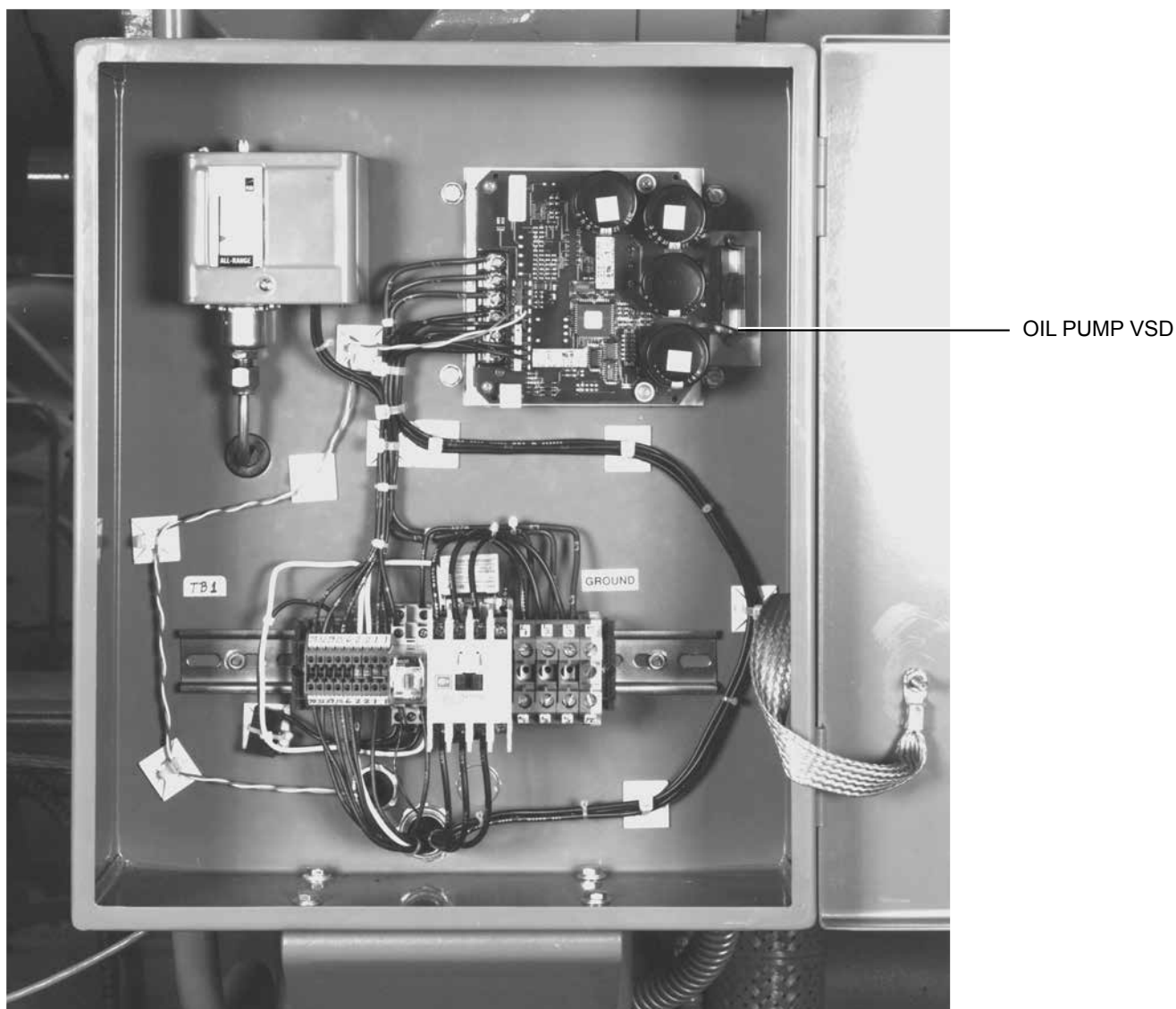
FIGURE 74 - OIL PUMP VARIABLE SPEED DRIVE (VSD)
