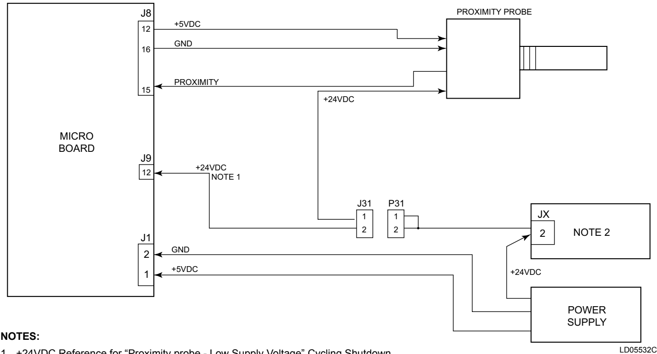
FIGURE 66 - PROXIMITY PROBE INTERFACE – PROBE PART NUMBER 025-30961-000
