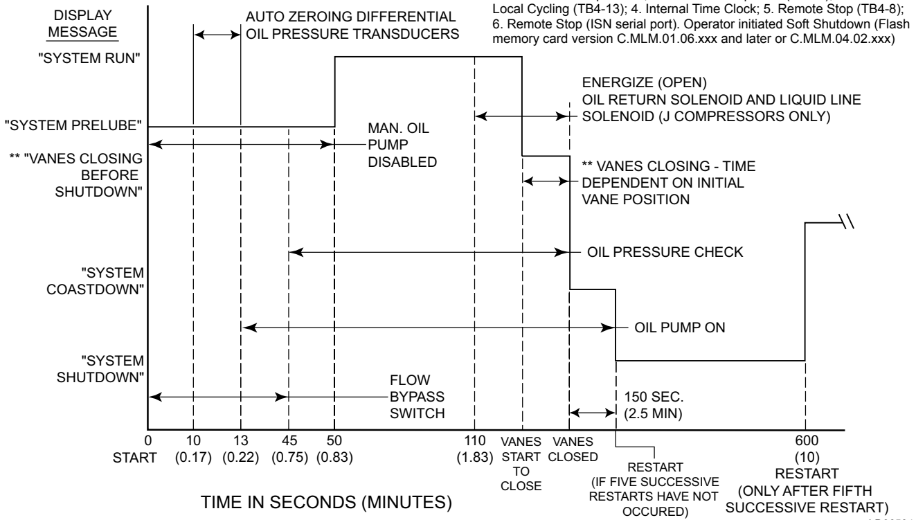
FIGURE 9 - OPERATION SEQUENCE TIMING DIAGRAM (COMPRESSOR MOTOR VARIABLE SPEED DRIVE APPLICATIONS)
