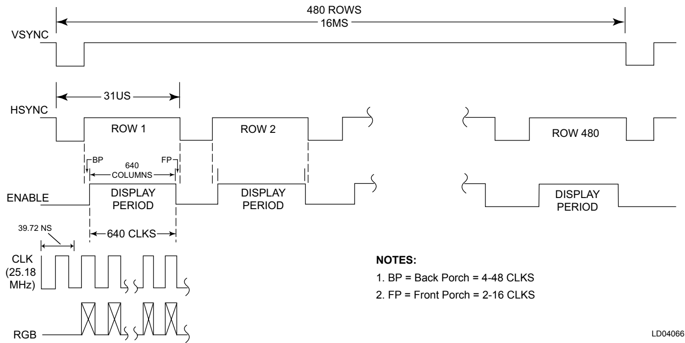
FIGURE 43 - LIQUID CRYSTAL DISPLAY TYPICAL CONTROL SIGNAL TIMING
