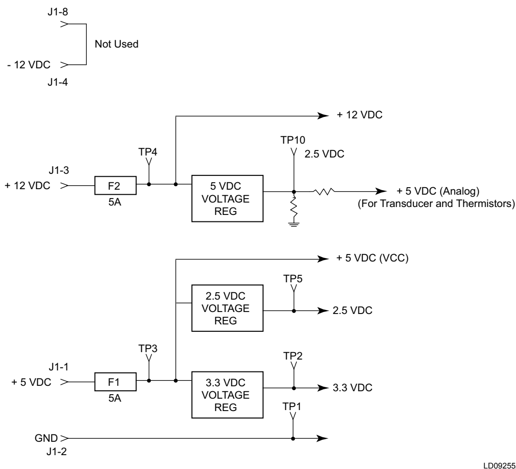
FIGURE 18 - PROGRAM CARD 031-02474-001
