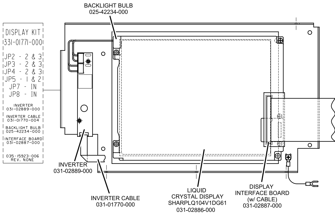
FIGURE 39 - LIQUID CRYSTAL DISPLAY ASSEMBLY – SHARP LQ10D367/368 (031-01774-000) DISPLAY
