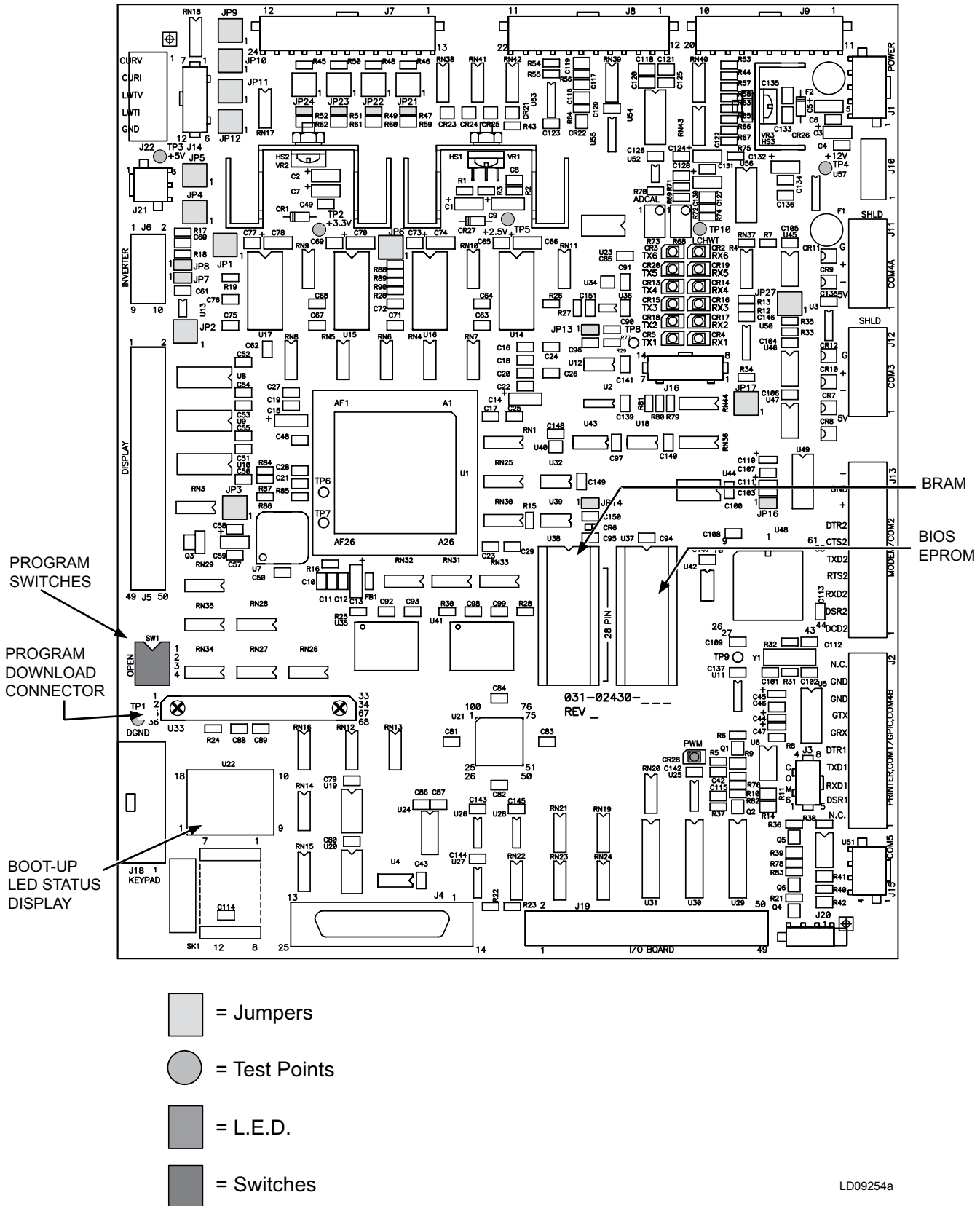
FIGURE 17 - MICROBOARD 031-02430-000 AND 031-02430-001
