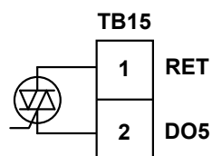
FIGURE 87 - TRIAC OUTPUTS
