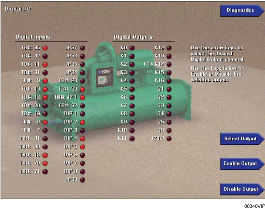
FIGURE 116 - DIGITAL INPUTS / OUTPUTS TEST SCREEN
