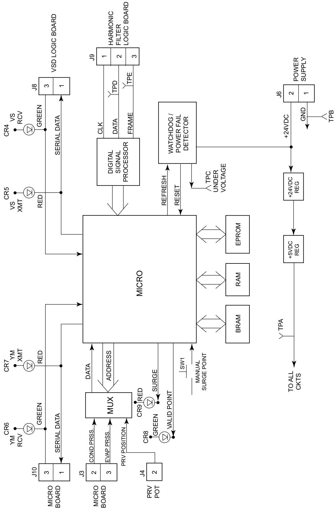
FIGURE 65 - ADAPTIVE CAPACITY CONTROL (ACC) BOARD
