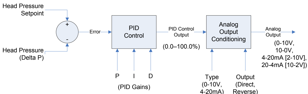
FIGURE 96 - HEAD PRESSURE CONTROL FLOW DIAGRAM
