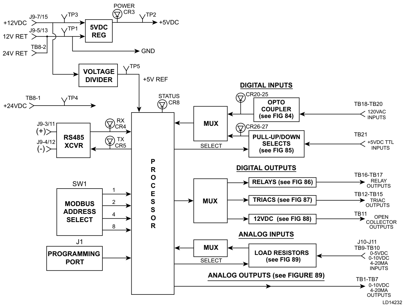
FIGURE 83 - LTC I/O BOARD BASIC BLOCK DIAGRAM
