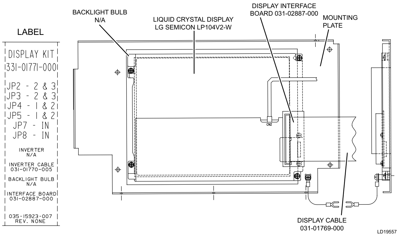
FIGURE 42 - LIQUID CRYSTAL DISPLAY ASSEMBLY – SHARP LQ104V1DG81 (031-01771-000)
