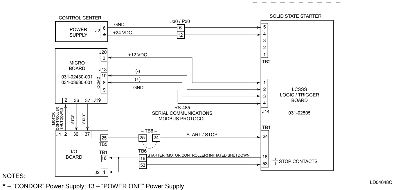
FIGURE 59 - STYLE B LIQUID COOLED SOLID STATE STARTER (LCSSS) – INTERFACE (MODBUS PROTOCOL)
