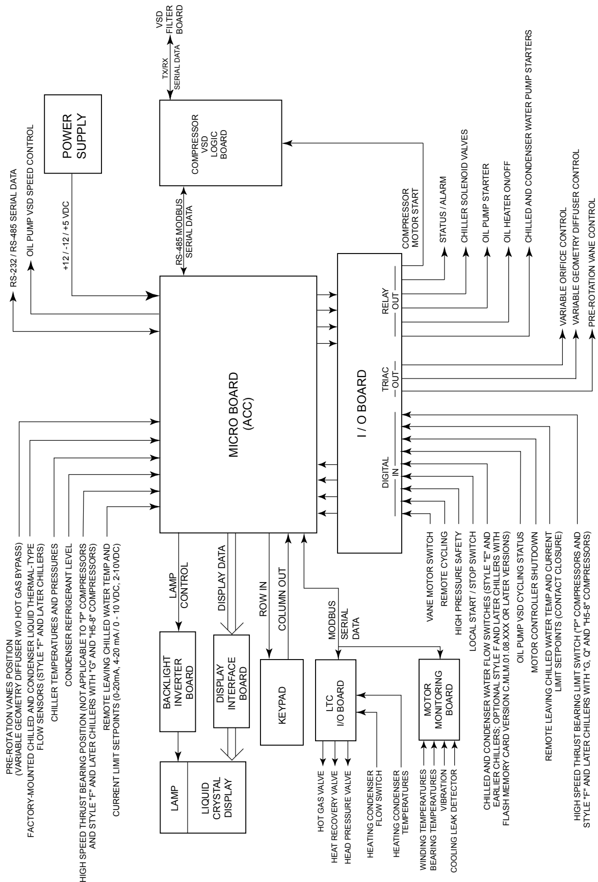
FIGURE 6 - OPTIVIEW™ CONTROL CENTER - COMPRESSOR MOTOR VARIABLE SPEED DRIVE (MODBUS SERIAL COMMUNICATIONS PROTOCOL)
