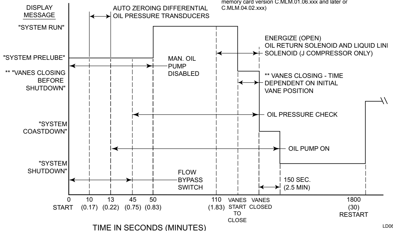
FIGURE 8 - OPERATION SEQUENCE TIMING DIAGRAM (ELECTRO-MECHANICAL AND SOLID STATE STARTER APPLICATIONS)
