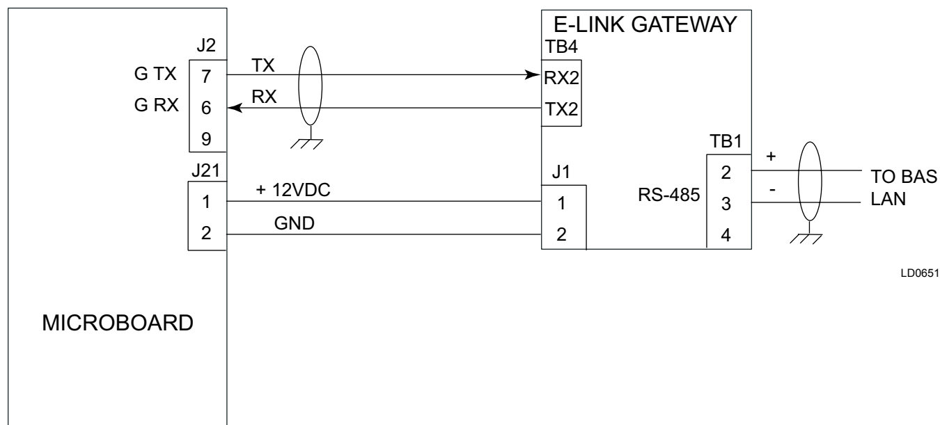
FIGURE 77 - E-LINK GATEWAY INTERFACE BLOCK DIAGRAM
