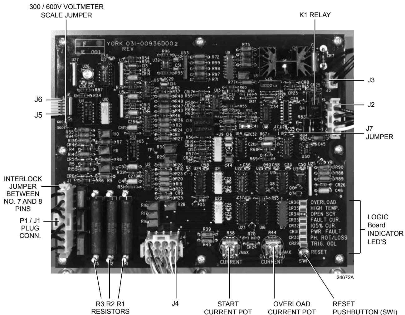
FIGURE 60 - SOLID STATE STARTER LOGIC BOARD
