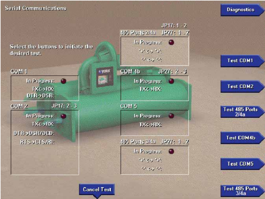
FIGURE 114 - SERIAL INPUTS / OUTPUTS TEST SCREEN
