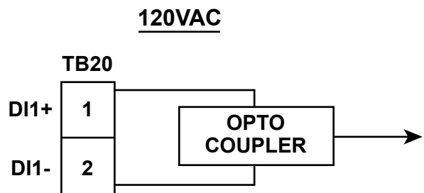
FIGURE 84 - 120VAC DIGITAL INPUT
