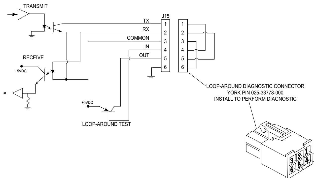
FIGURE 114 - MICROBOARD - COM 5 SERIAL DATA PORT
