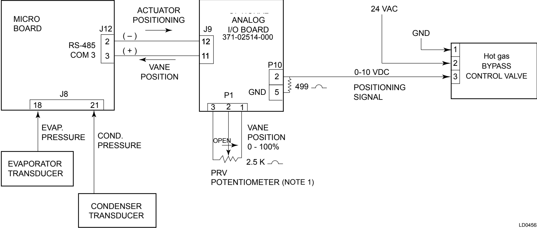
FIGURE 79 - INTERFACE, HOT GAS BYPASS (ANALOG I/O BOARD 371-02514-000)
