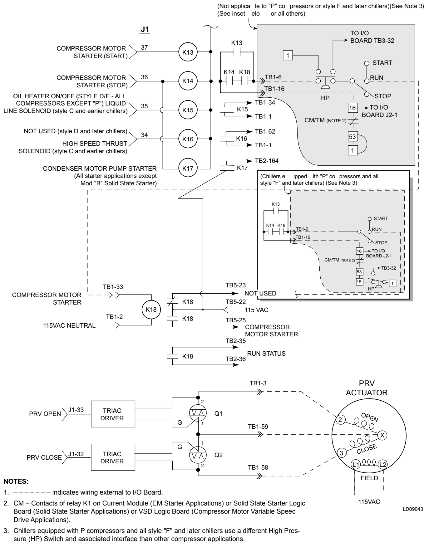
FIGURE 29 - J1 I/O BOARD DIGITAL OUTPUTS (CONT'D)
