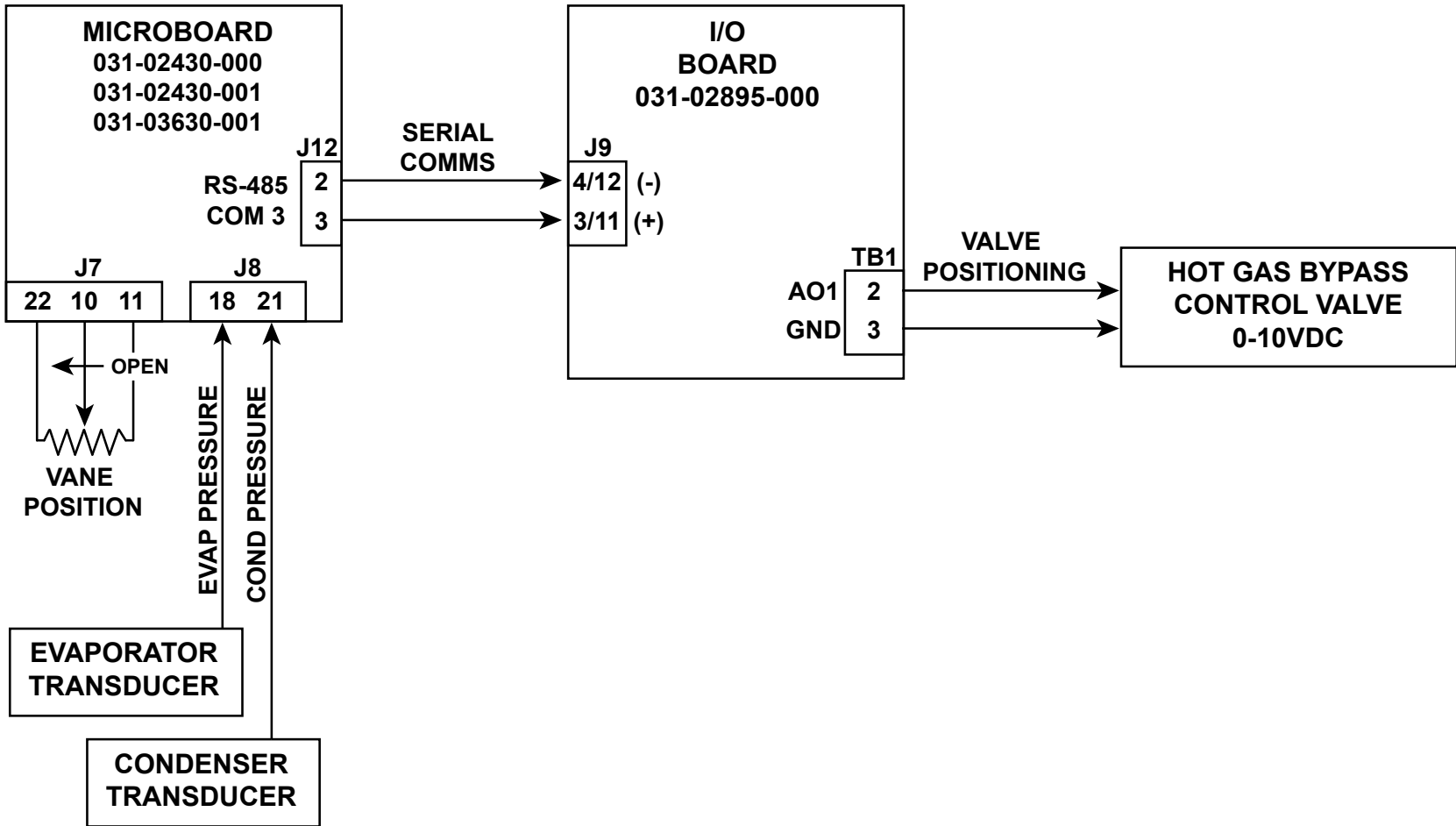
FIGURE 80 - INTERFACE, HOT GAS BYPASS (I/O BOARD 031-02895-000)
