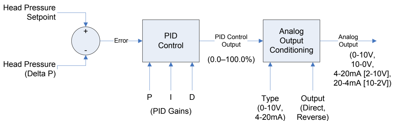
FIGURE 96 - HEAD PRESSURE CONTROL FLOW DIAGRAM
