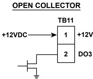
FIGURE 88 - OPEN COLLECTOR
