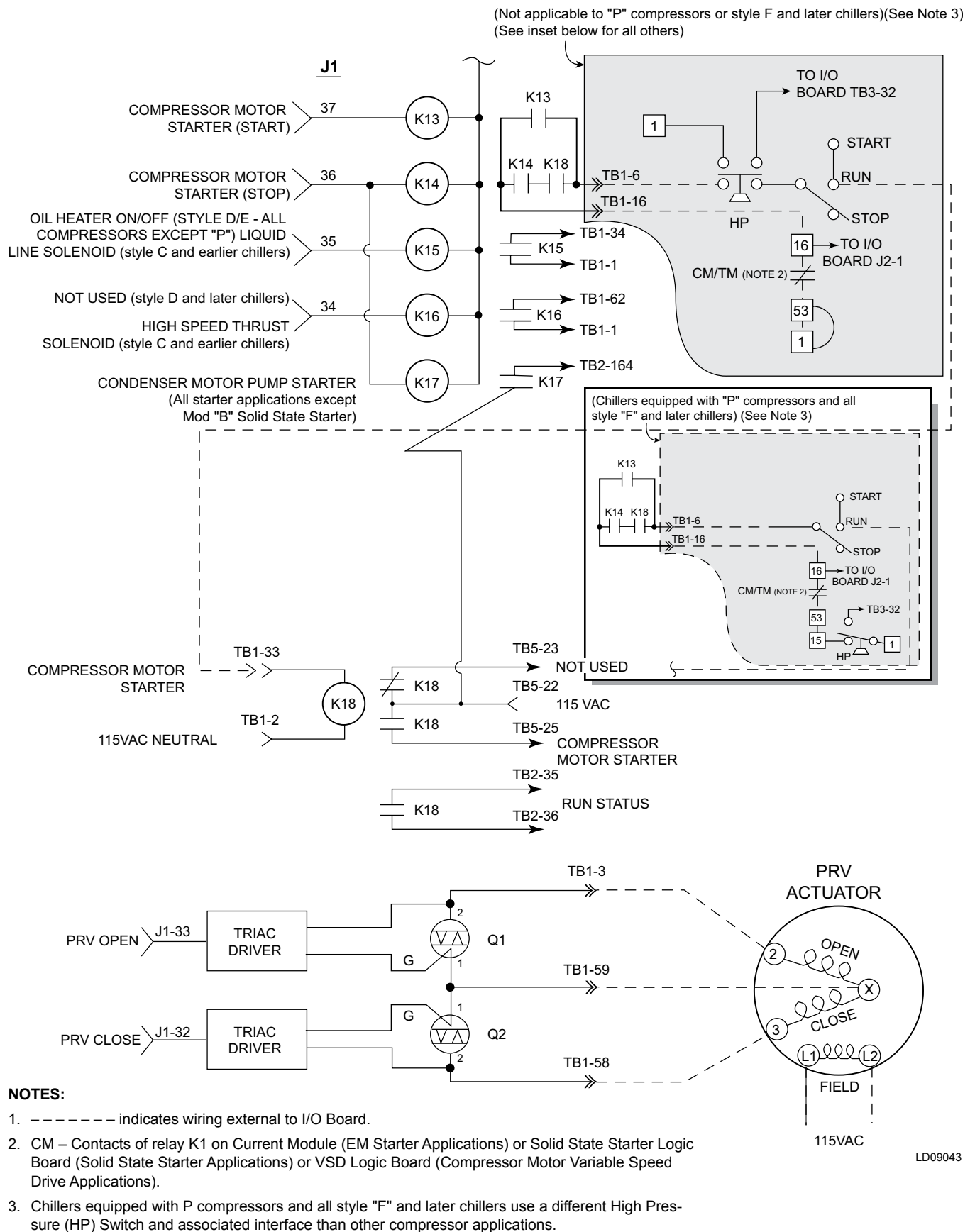
FIGURE 37 - J1 I/O BOARD DIGITAL OUTPUTS (CONT'D)
