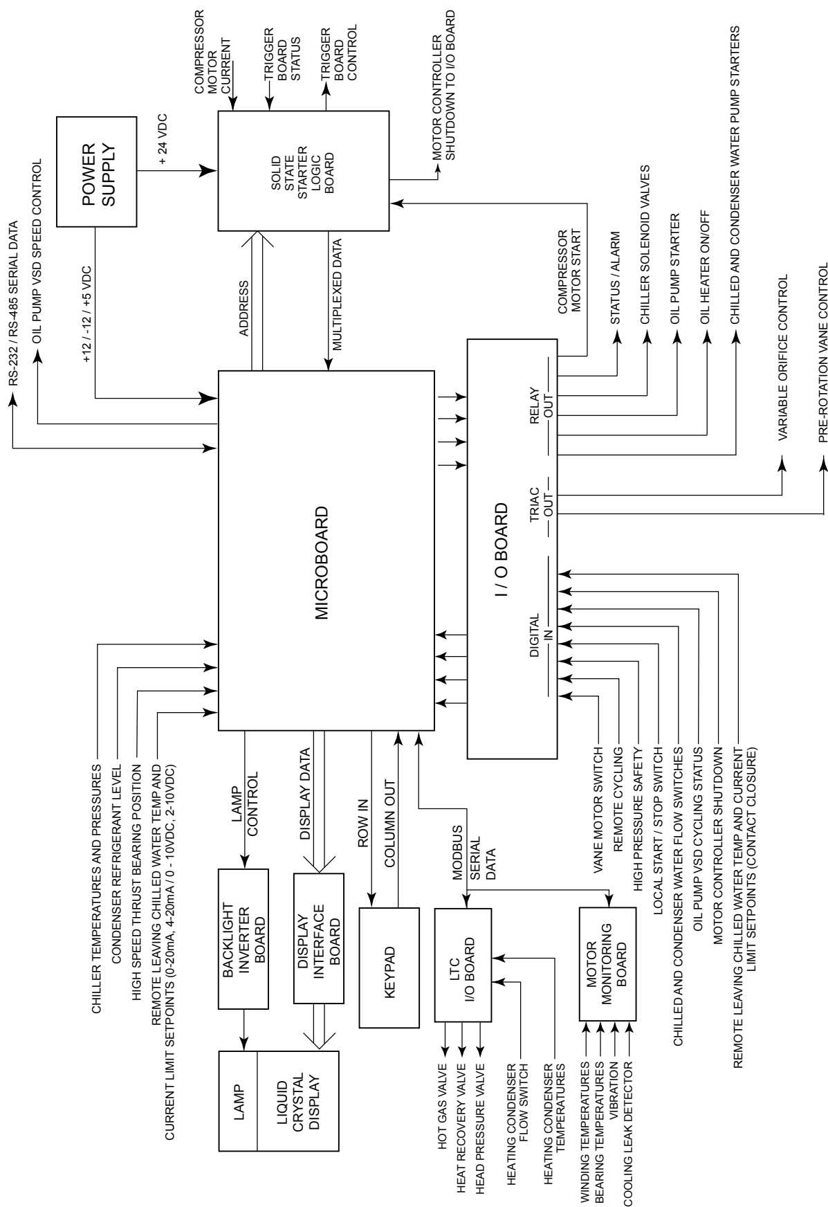
FIGURE 2 - OPTIVIEW™ CONTROL CENTER - MOD A SOLID STATE STARTER APPLICATIONS
