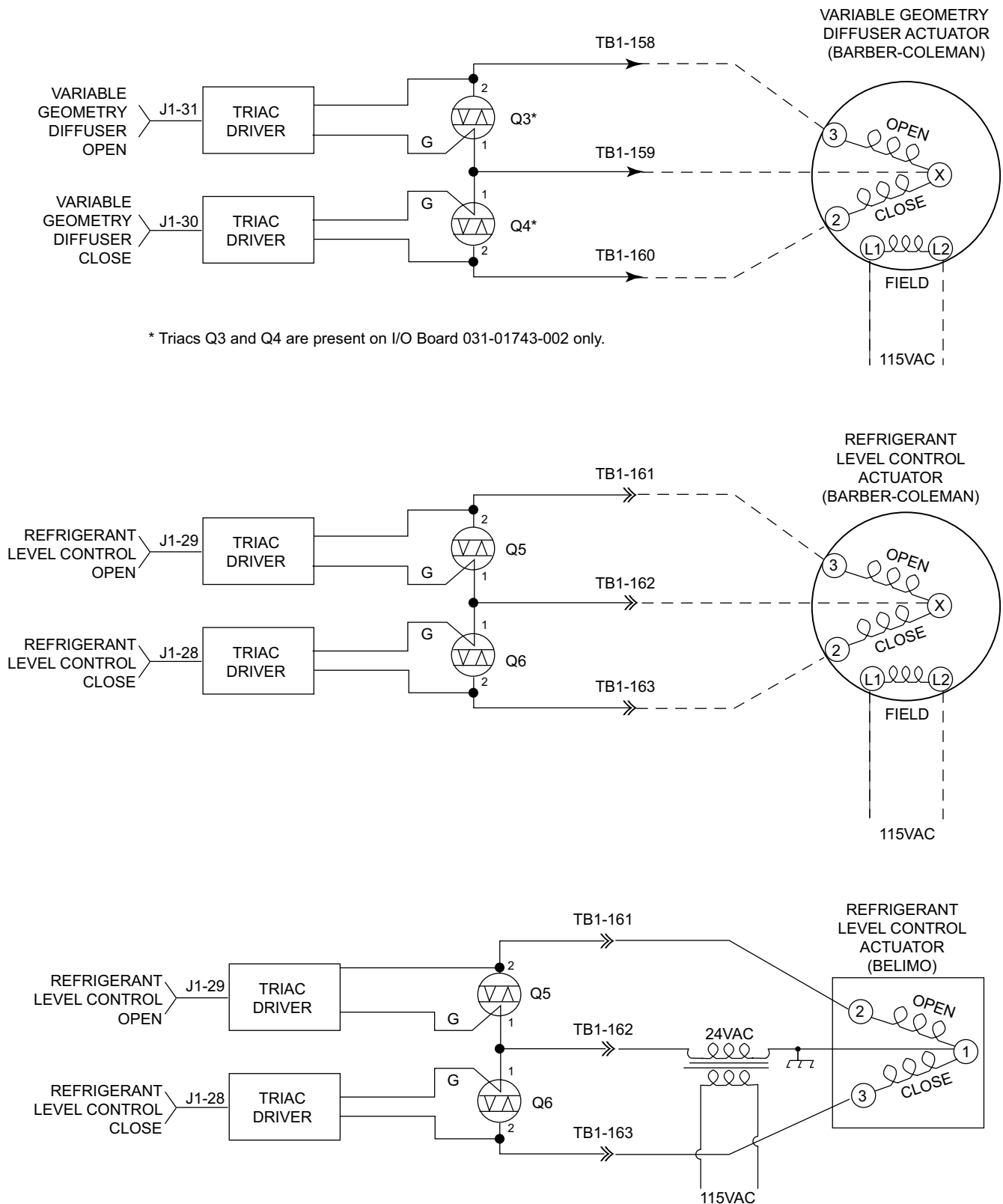
FIGURE 37 - J1 I/O BOARD DIGITAL OUTPUTS (CONT'D)
