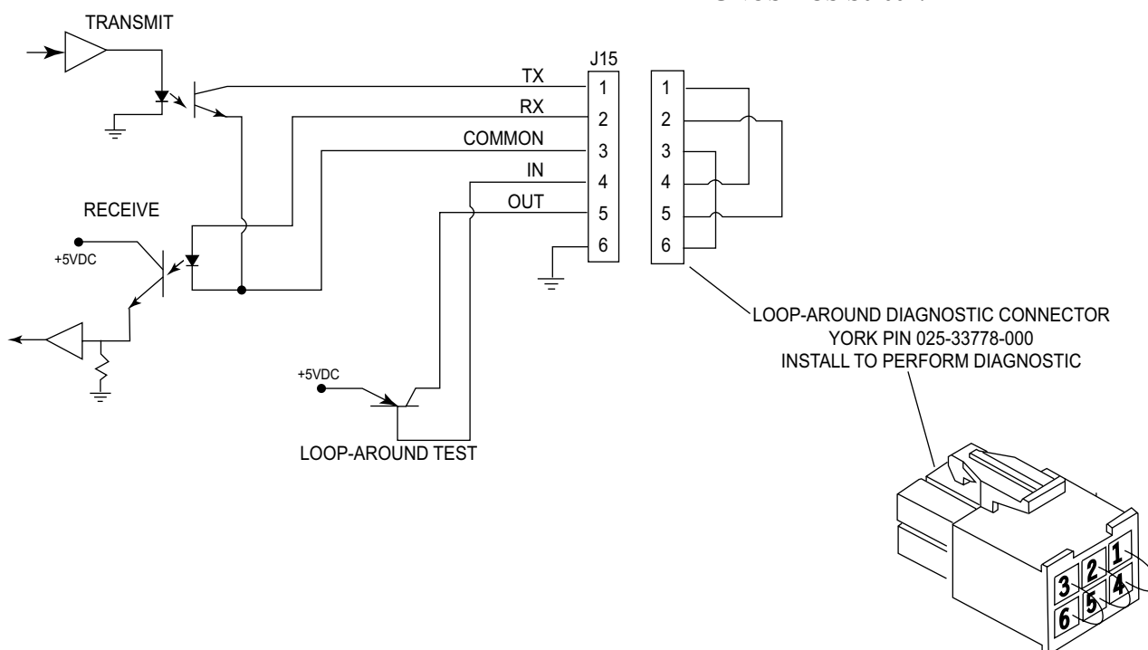
FIGURE 115 - MICROBOARD - COM 5 SERIAL DATA PORT
