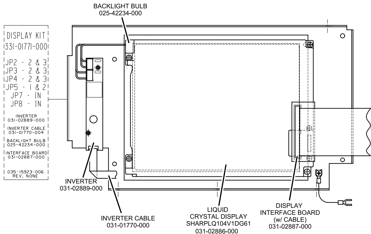
FIGURE 39 - LIQUID CRYSTAL DISPLAY ASSEMBLY – SHARP LQ10D367/368 (031-01774-000) DISPLAY
