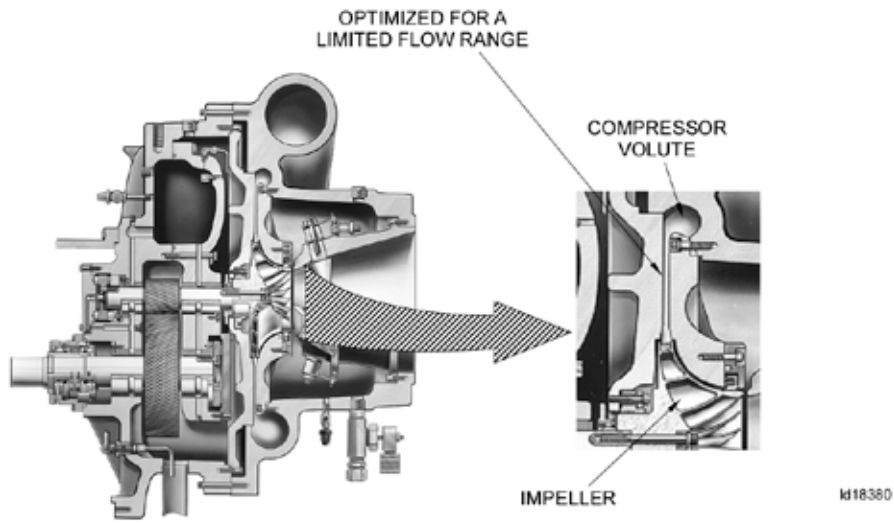
FIGURE 4 - TYPICAL OPTIMIZED CENTRIFUGAL COMPRESSOR
