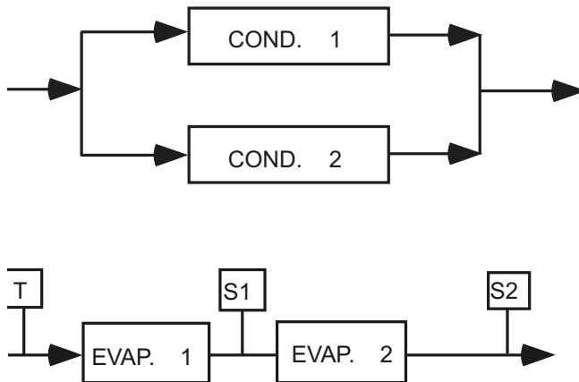
FIGURE 6 - SERIES EVAPORATORS PARALLEL CONDENSERS
