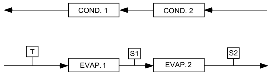
FIGURE 7 - SERIES EVAPORATORS SERIES COUNTERFLOW CONDENSERS
