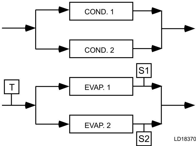
FIGURE 5 - PARALLEL EVAPORATORS PARALLEL CONDENSERS
