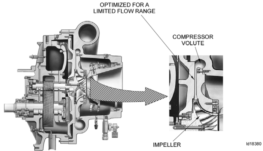
FIGURE 2 - TYPICAL OPTIMIZED CENTRIFUGAL COMPRESSOR
