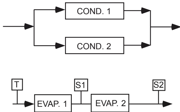
FIGURE 4 - SERIES EVAPORATORS PARALLEL CONDENSERS
