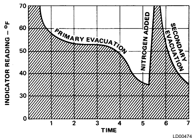
FIGURE 15 - SATURATION CURVE
