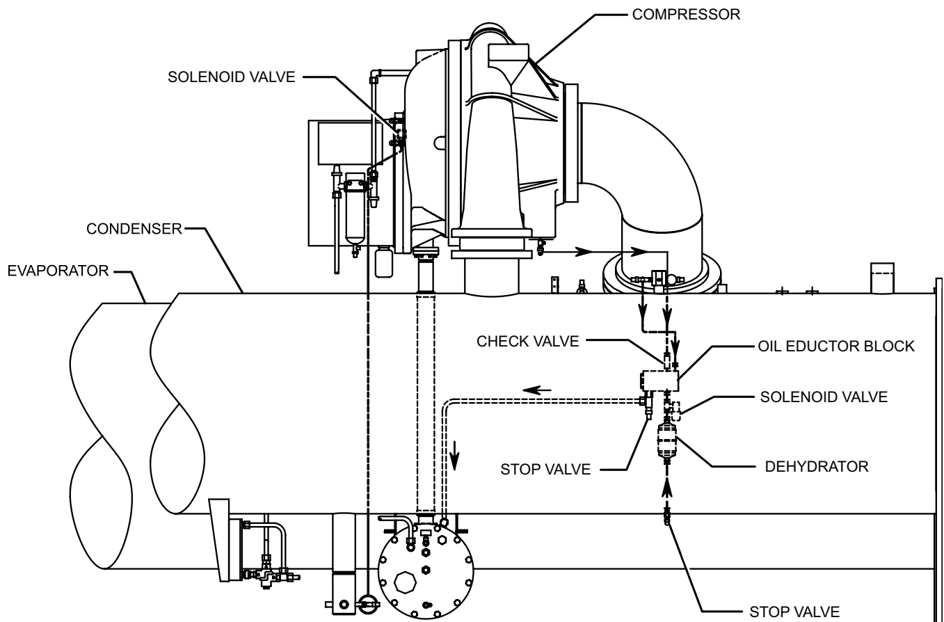
FIGURE 12 - OIL RETURN SYSTEM
