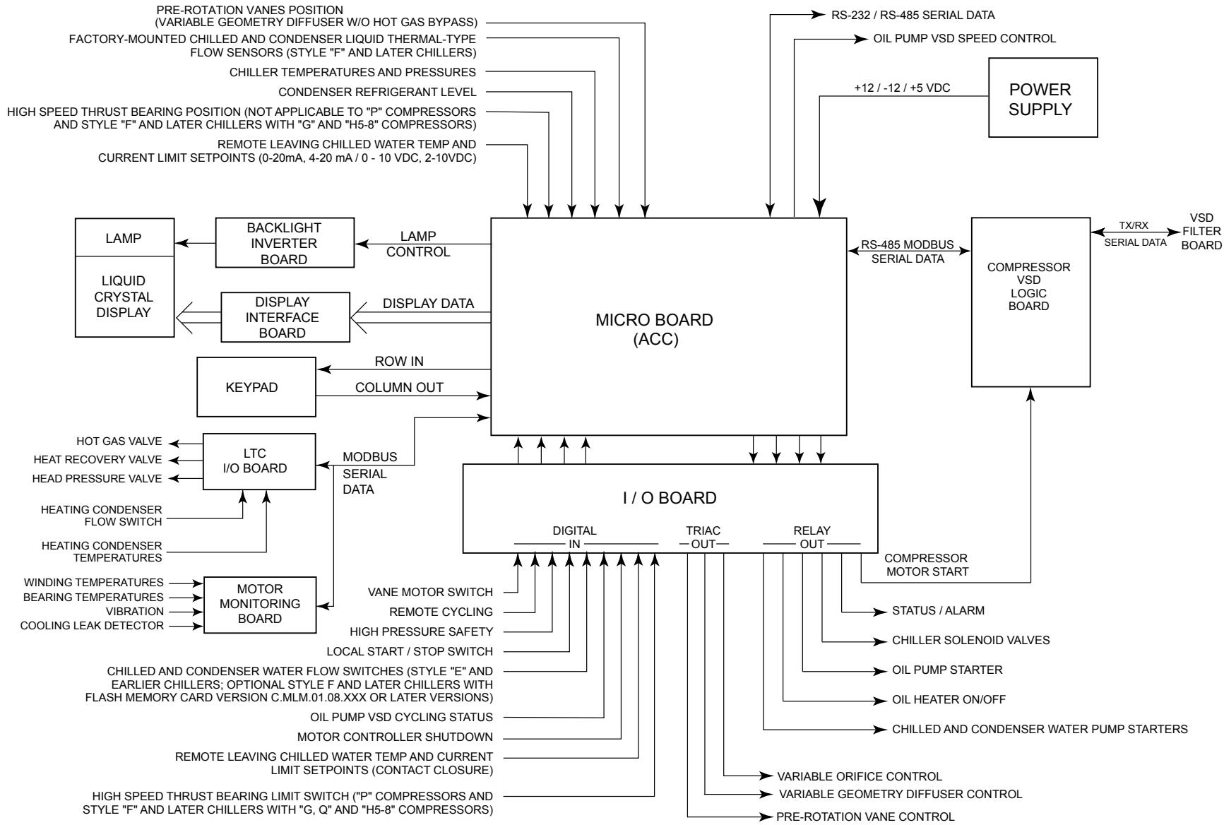
FIGURE 6 - OPTIVIEW™ CONTROL CENTER - COMPRESSOR MOTOR VARIABLE SPEED DRIVE (MODBUS SERIAL COMMUNICATIONS PROTOCOL)
