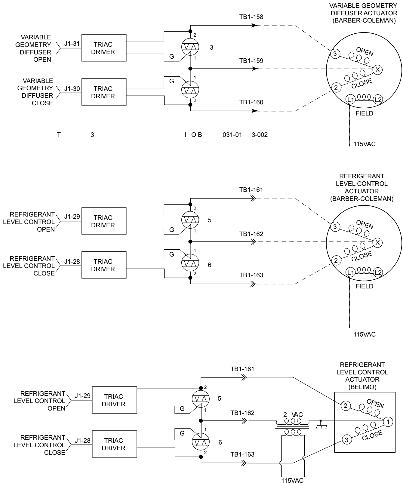
FIGURE 29 - J1 I/O BOARD DIGITAL OUTPUTS (CONT'D)
