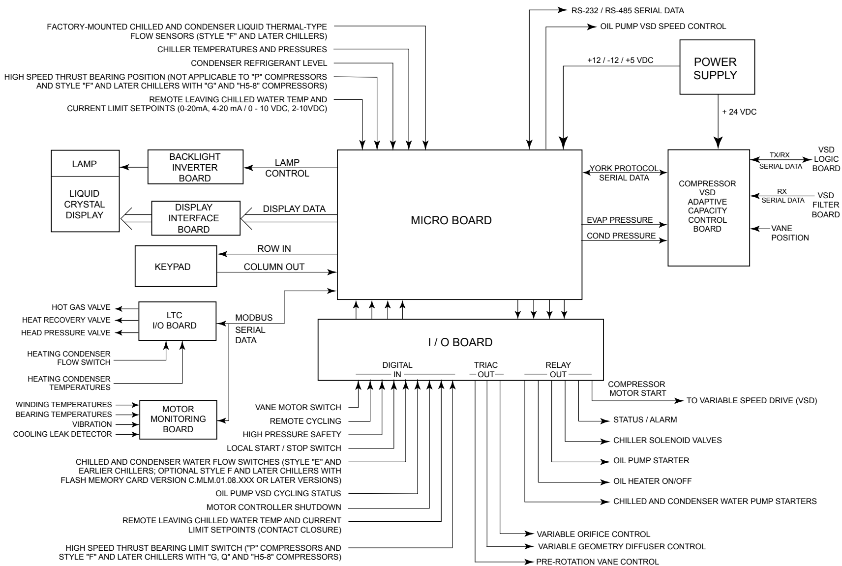
FIGURE 5 - OPTIVIEW™ CONTROL CENTER - COMPRESSOR MOTOR VARIABLE SPEED DRIVE (YORK SERIAL COMMUNICATIONS PROTOCOL)
