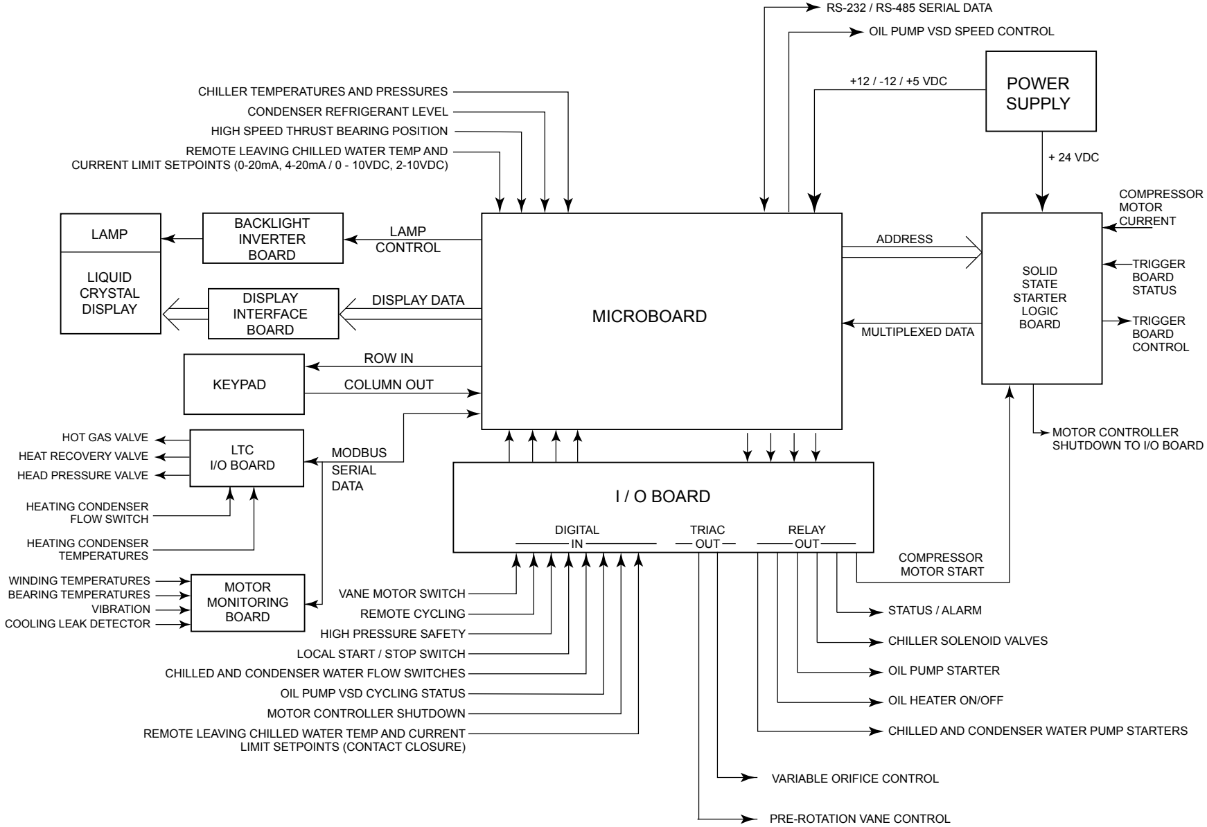
FIGURE 2 - OPTIVIEW™ CONTROL CENTER - MOD A SOLID STATE STARTER APPLICATIONS
