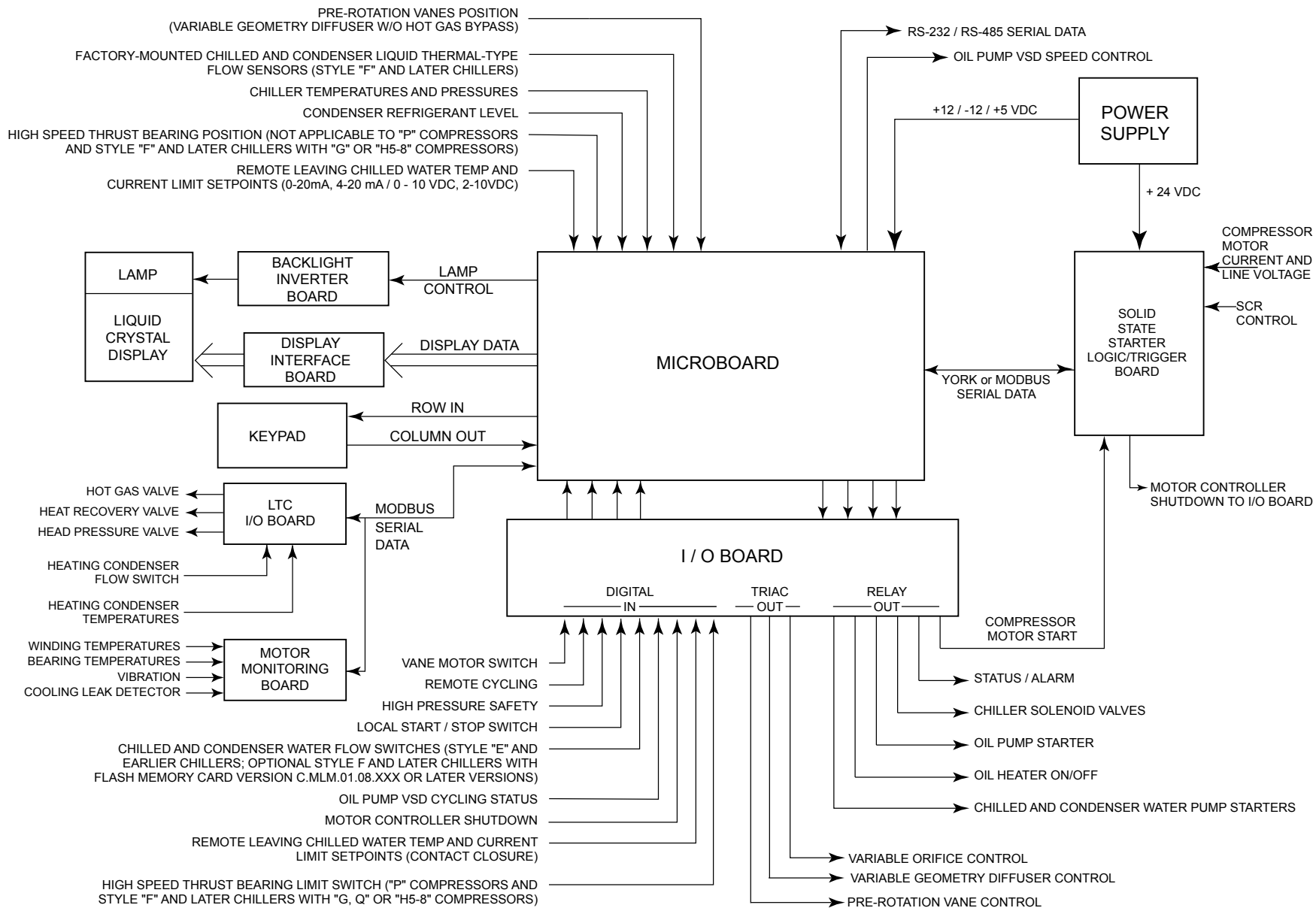
FIGURE 3 - OPTIVIEW™ CONTROL CENTER - MOD B SOLID STATE STARTER APPLICATIONS
