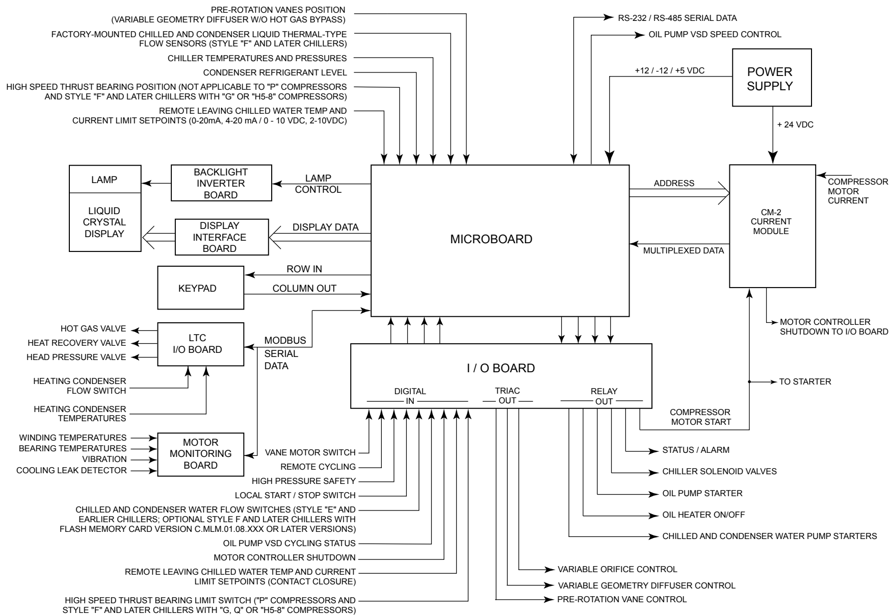
FIGURE 1 - OPTIVIEW™ CONTROL CENTER - ELECTRO-MECHANICAL STARTER APPLICATIONS
