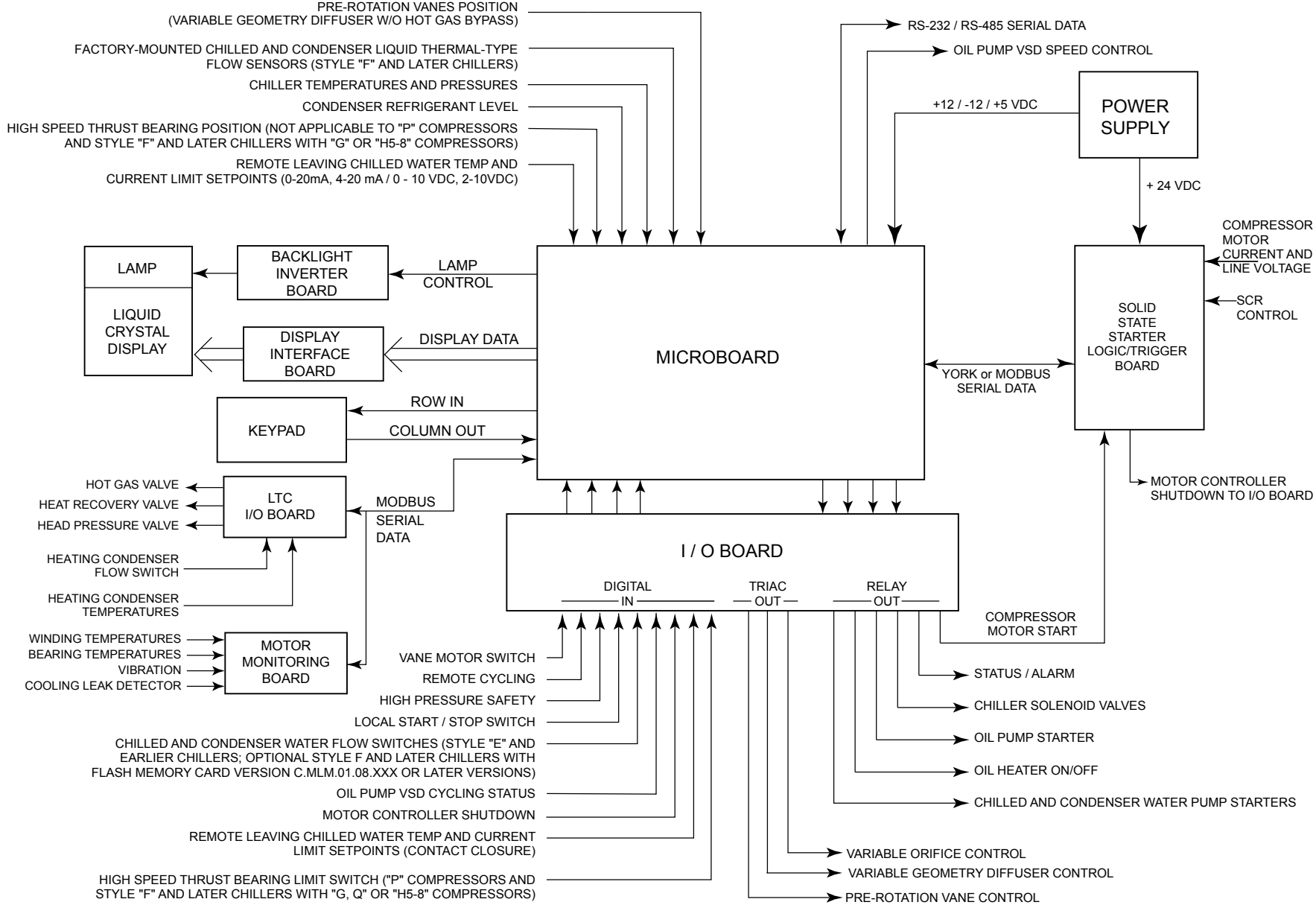
FIGURE 4 - OPTIVIEW™ CONTROL CENTER - MEDIUM VOLTAGE SOLID STATE STARTER APPLICATIONS
