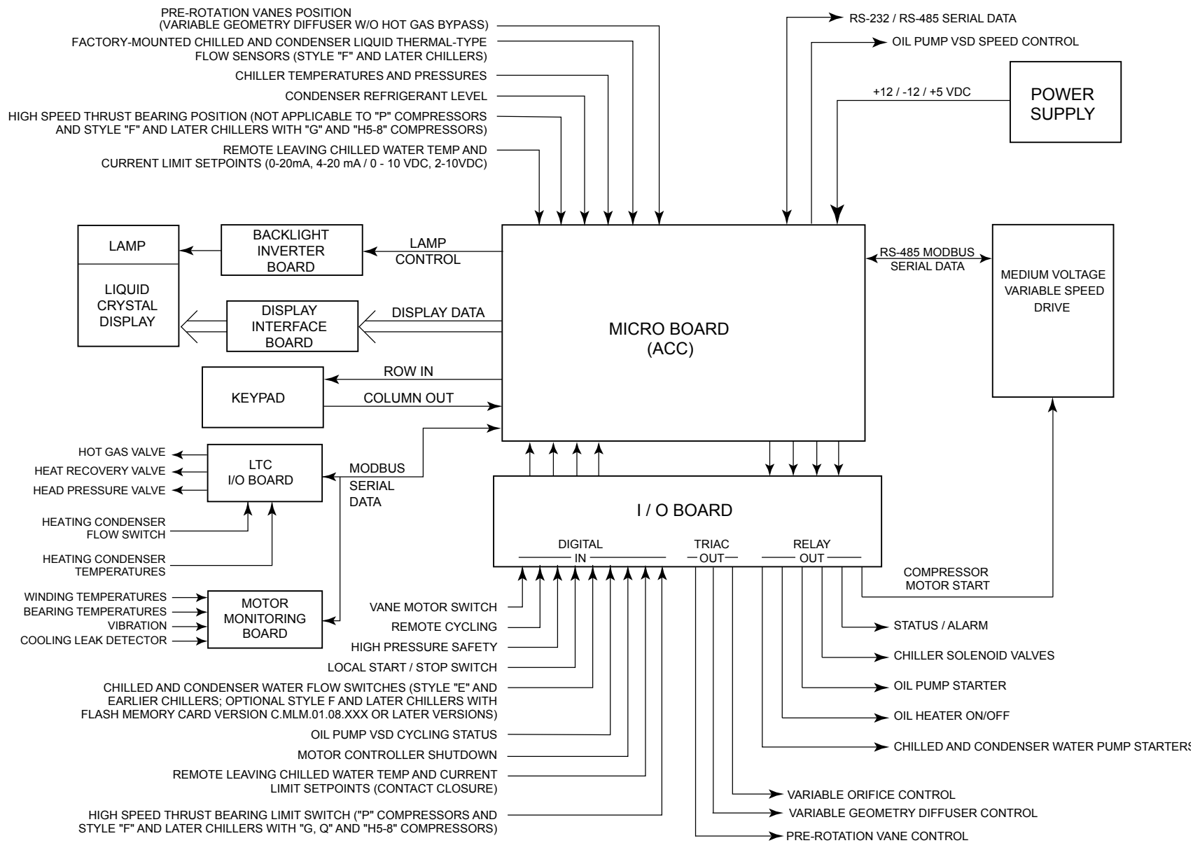
FIGURE 7 - OPTIVIEW™ CONTROL CENTER - COMPRESSOR MOTOR MEDIUM VOLTAGE VARIABLE SPEED DRIVE
