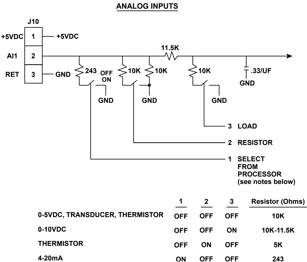
FIGURE 89 - ANALOG INPUTS
