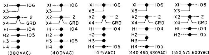
5T TRANSFORMER CONNECTIONS
