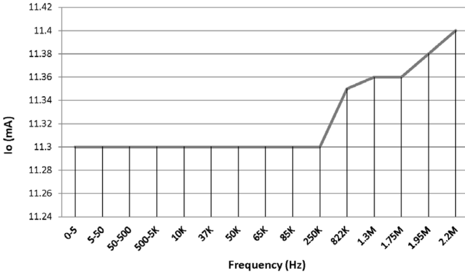
CS02: RF NOISE IMMUNITY TEST RESULTS
