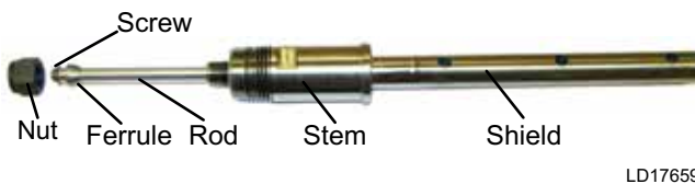
FIGURE 5 - CS01 PROBE WITH ROD
