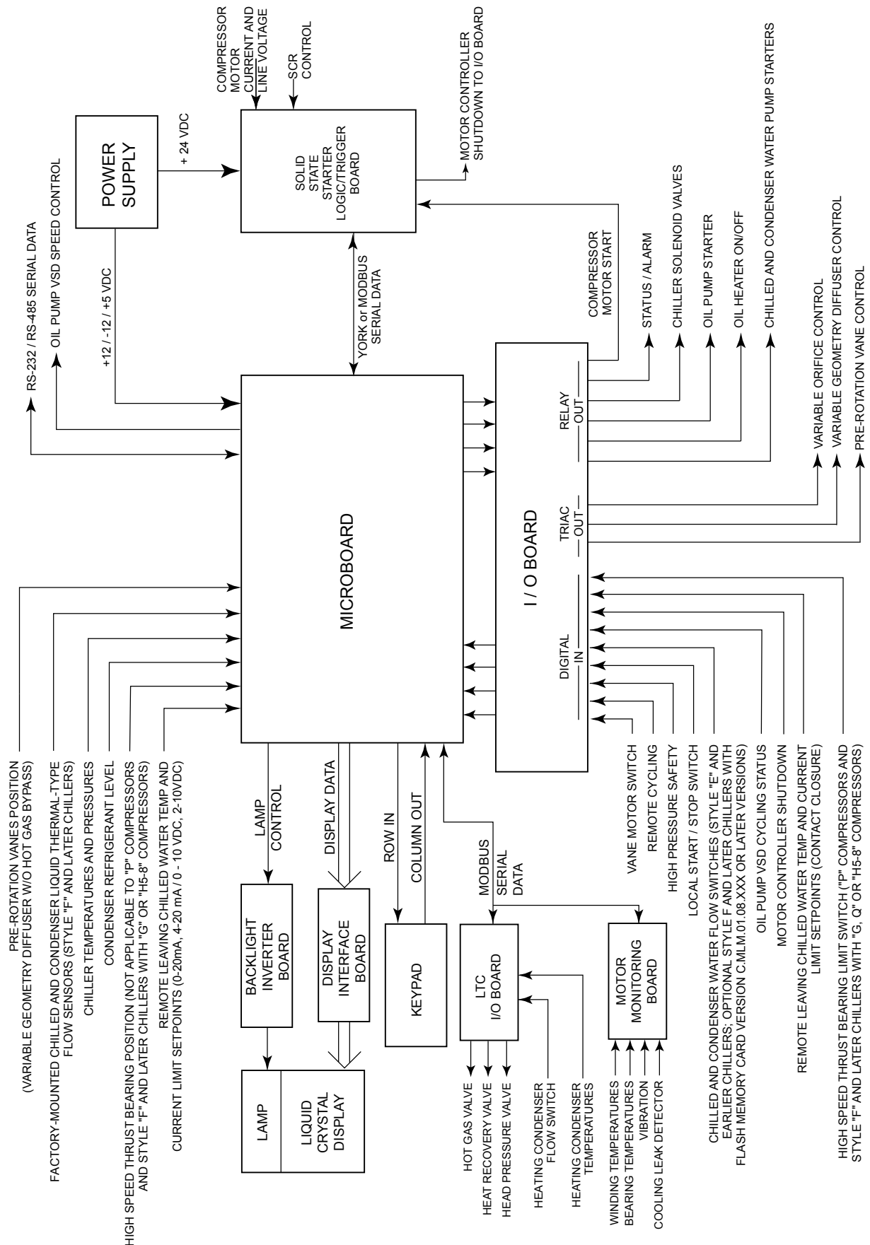
FIGURE 4 - OPTIVIEW™ CONTROL CENTER - MEDIUM VOLTAGE SOLID STATE STARTER APPLICATIONS
