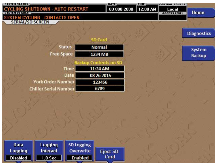
FIGURE 107 - SERIAL/SD SCREEN
