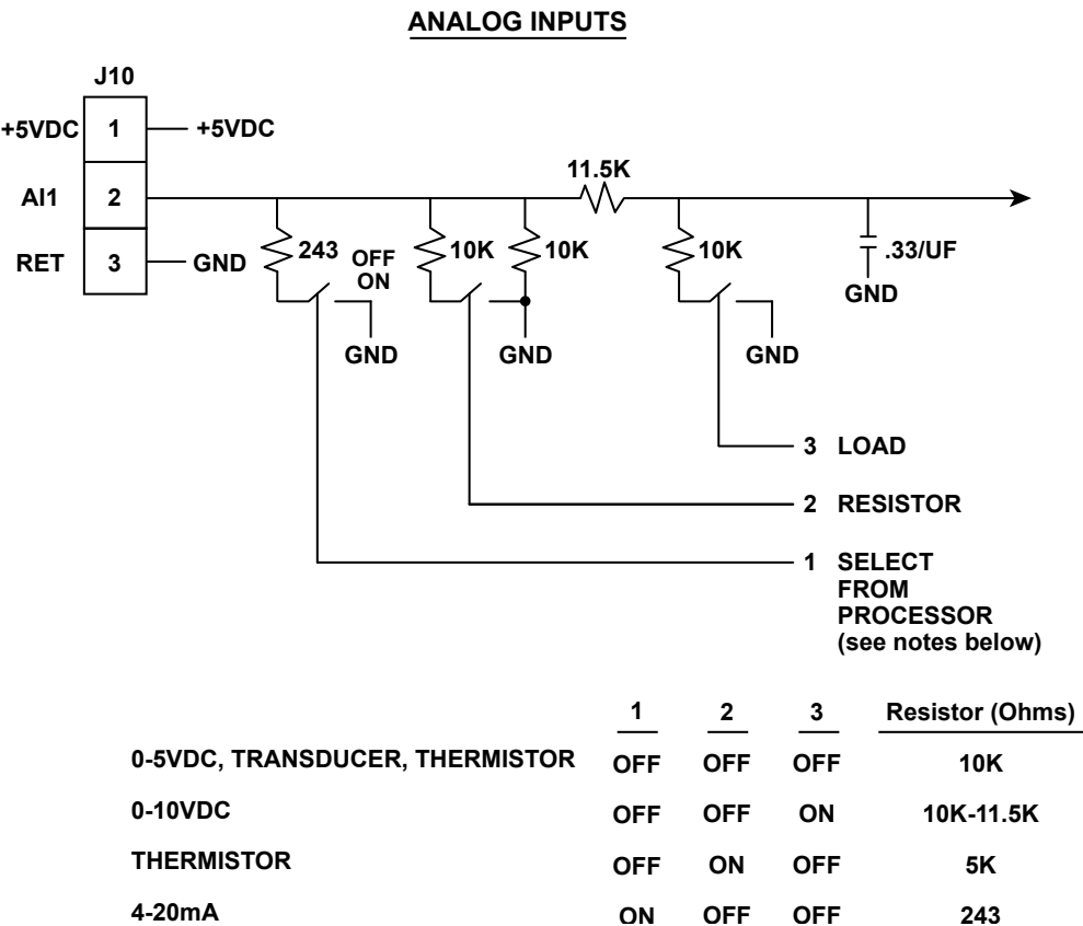
FIGURE 89 - ANALOG INPUTS
