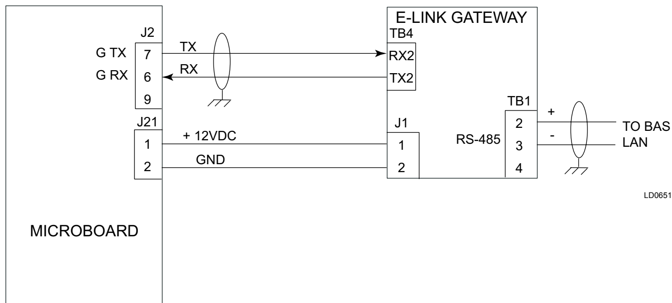
FIGURE 69 - E-LINK GATEWAY INTERFACE BLOCK DIAGRAM
