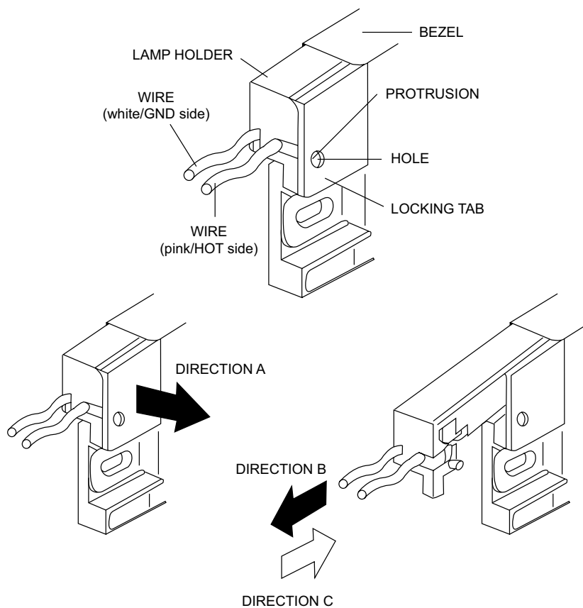
FIGURE 35 - DISPLAY (SHARP LQ10D367/368) LAMP REPLACEMENT
