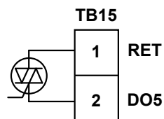
FIGURE 79 - TRIAC OUTPUTS
