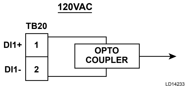
FIGURE 76 - 120VAC DIGITAL INPUT
