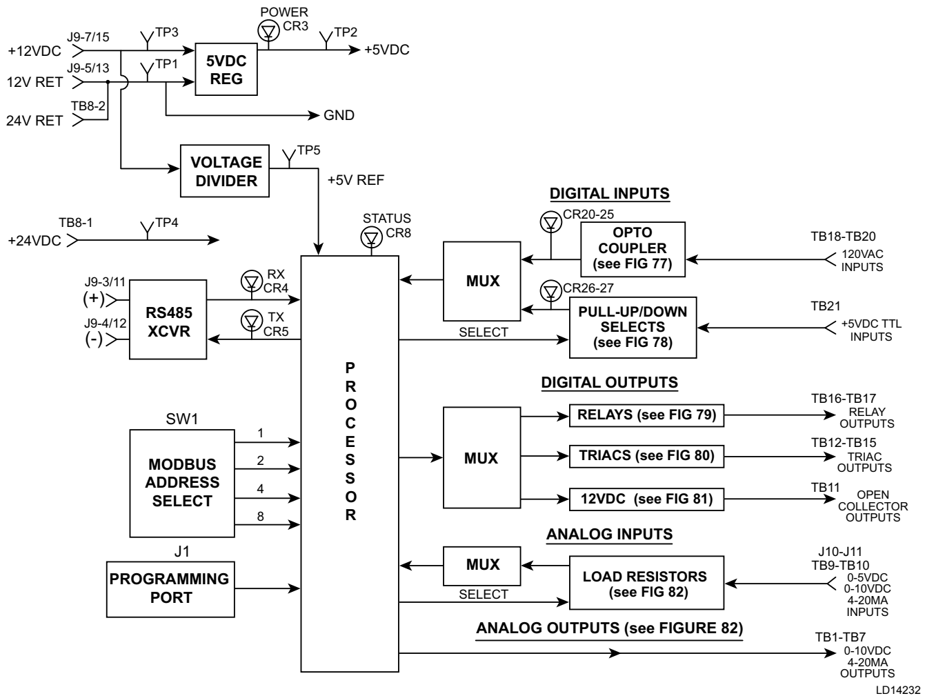
FIGURE 75 - LTC I/O BOARD BASIC BLOCK DIAGRAM
