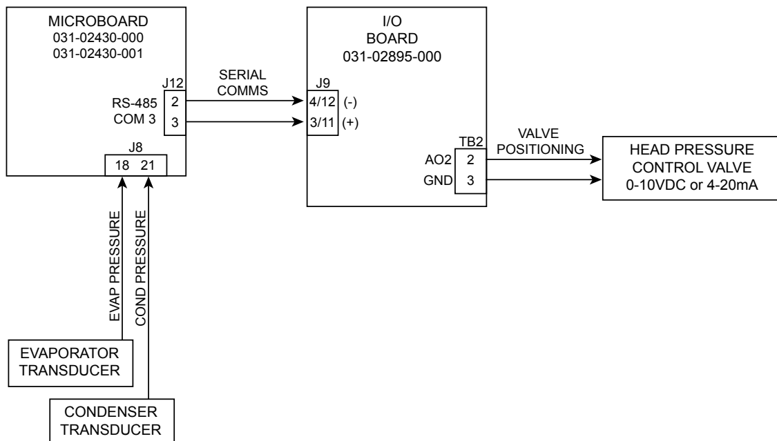
FIGURE 87 - HEAD PRESSURE CONTROL BLOCK DIAGRAM
