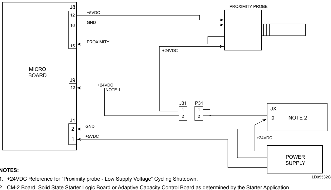
FIGURE 59 - PROXIMITY PROBE INTERFACE – PROBE PART NUMBER 025-35900-000 AND 025-35900-001
