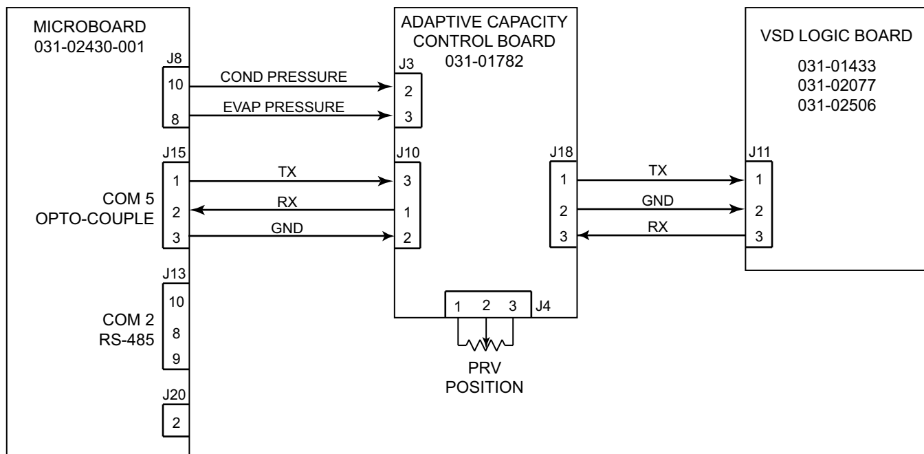
FIGURE 55 - SERIAL COMMUNICATIONS INTERFACE – YORK PROTOCOL
