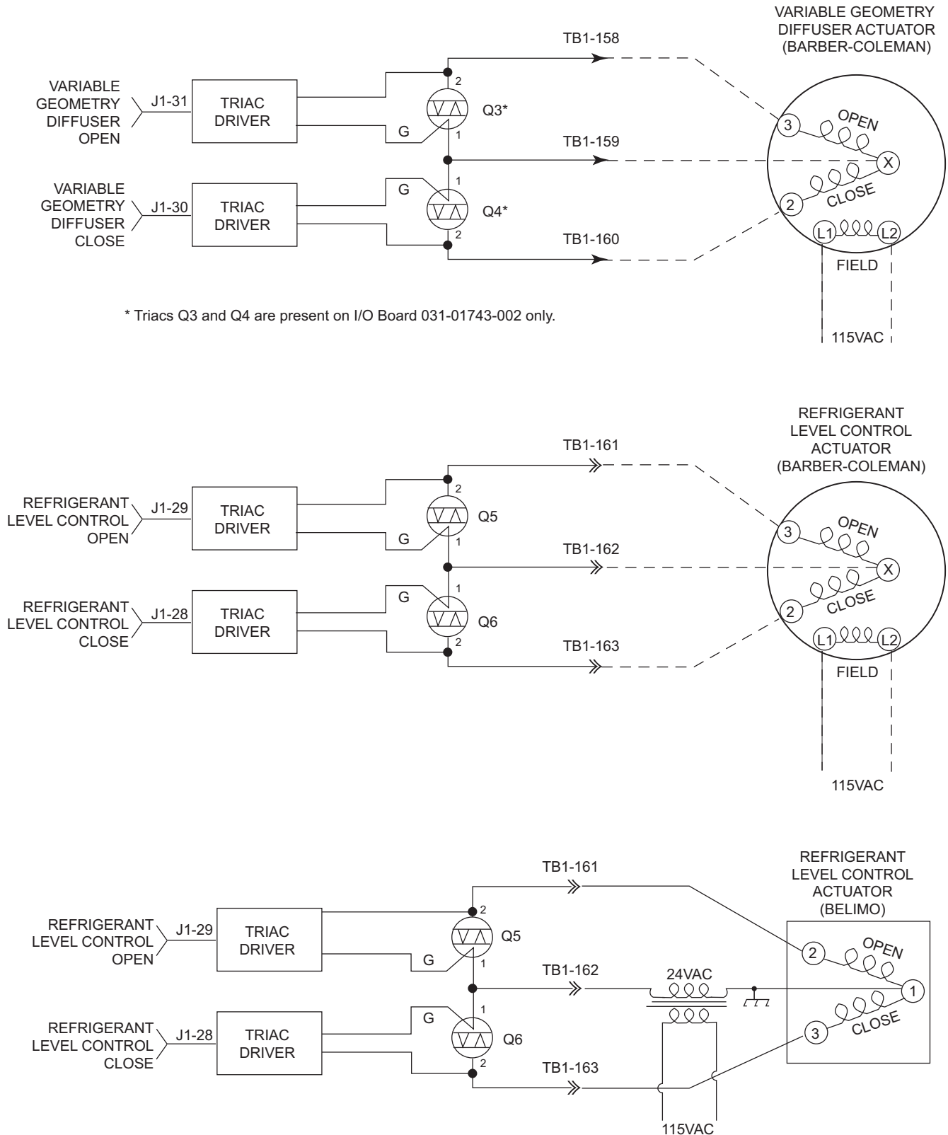
FIGURE 29 - J1 I/O BOARD DIGITAL OUTPUTS (CONT'D)
