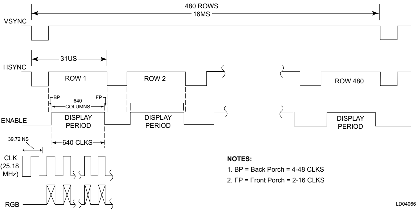
FIGURE 34 - LIQUID CRYSTAL DISPLAY TYPICAL CONTROL SIGNAL TIMING
