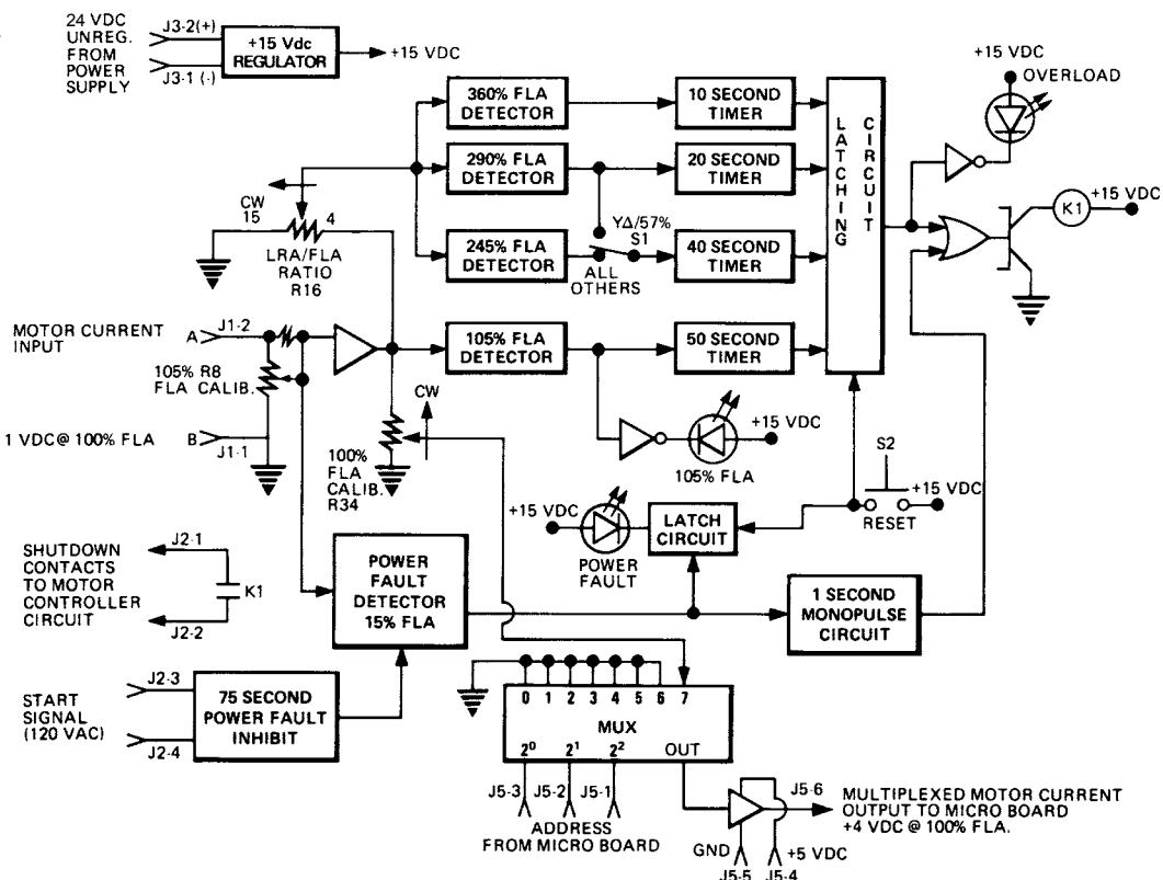
FIGURE 46 - CM-2 CURRENT MODULE (ELECTRO-MECHANICAL STARTER APPLICATIONS)
