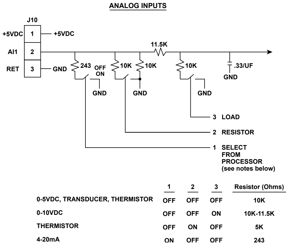
FIGURE 81 - ANALOG INPUTS
