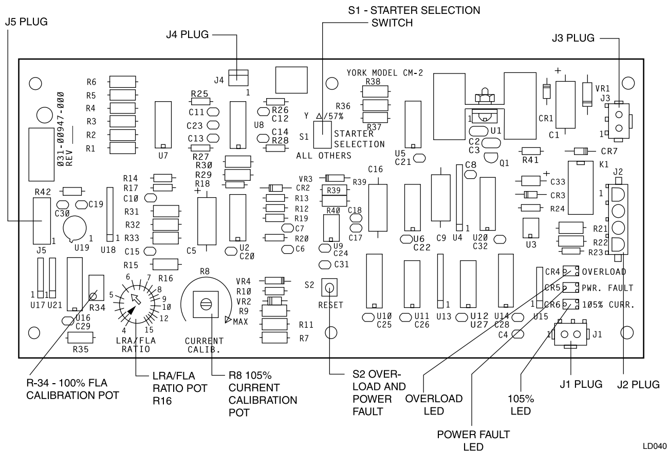
FIGURE 45 - CM-2 CURRENT MODULE (ELECTRO-MECHANICAL STARTER APPLICATION)
