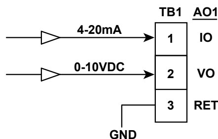
FIGURE 82 - ANALOG OUTPUTS
