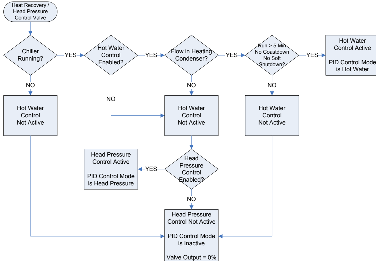
FIGURE 86 - HEAT RECOVERY FLOW DIAGRAM
