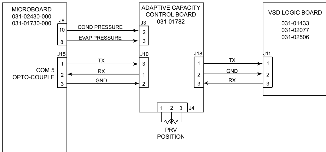
FIGURE 54 - SERIAL COMMUNICATIONS INTERFACE – YORK PROTOCOL
