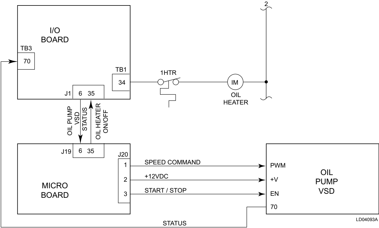
FIGURE 67 - OIL PUMP VSD / OIL HEATER CONTROL – INTERFACE
