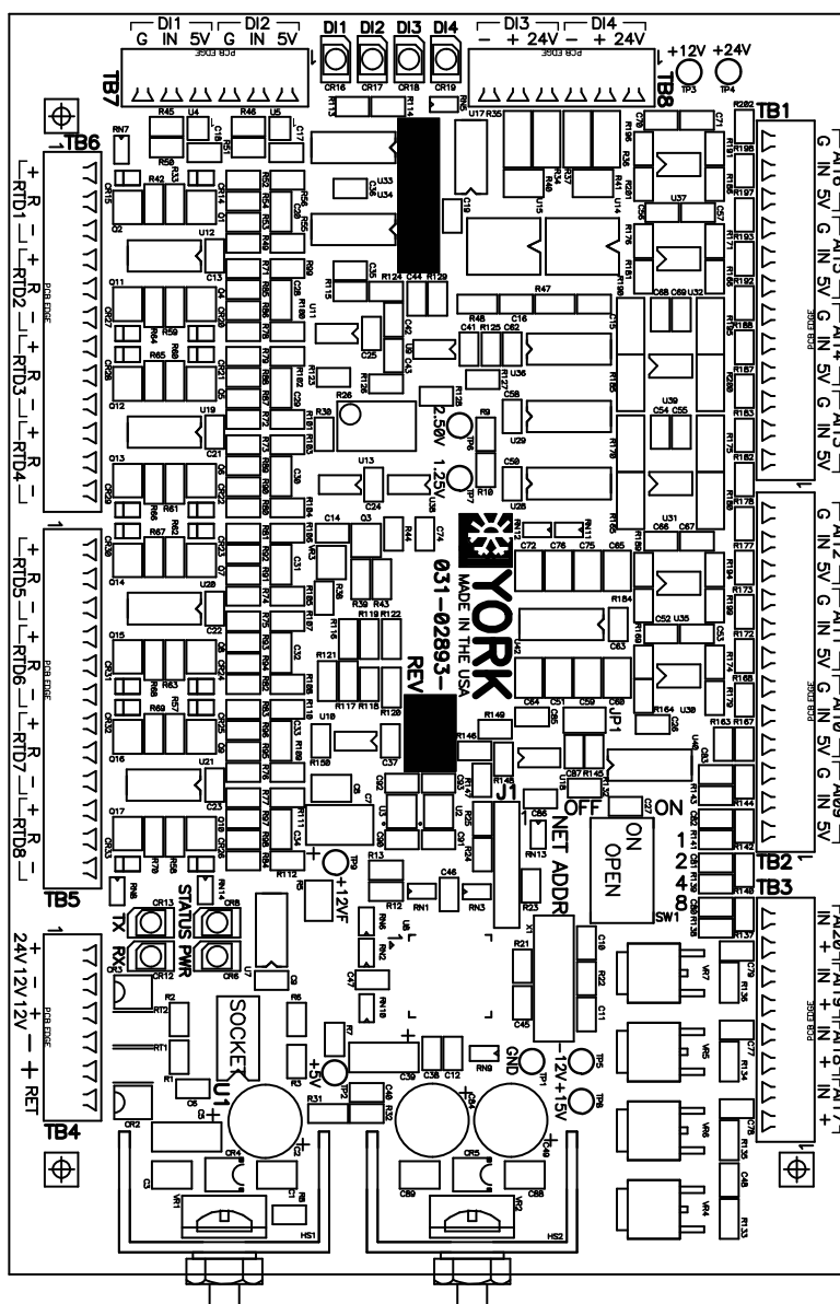
FIGURE 90 - MOTOR MONITORING BOARD (031-02893-000/001)
