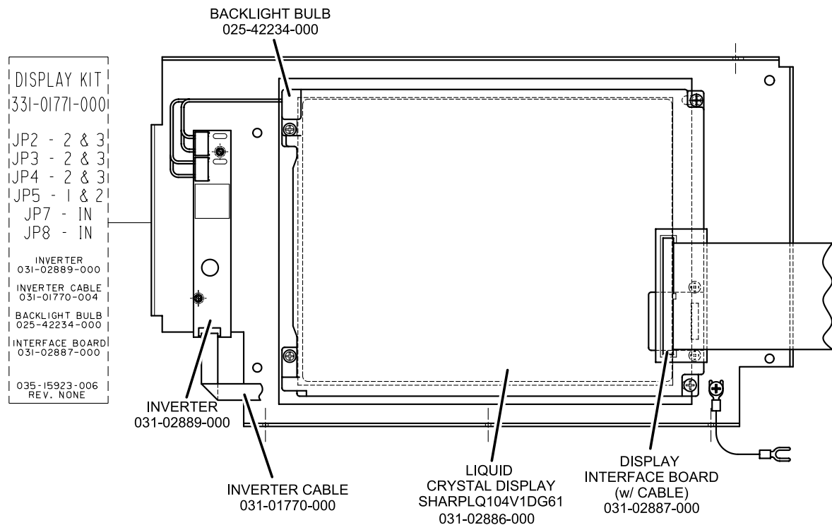
FIGURE 31 - LIQUID CRYSTAL DISPLAY ASSEMBLY – SHARP LQ10D367/368 (031-01774-000) DISPLAY
