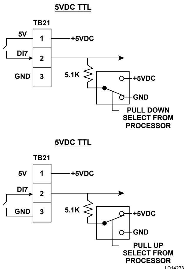
FIGURE 77 - +5VDC DIGITAL INPUT
