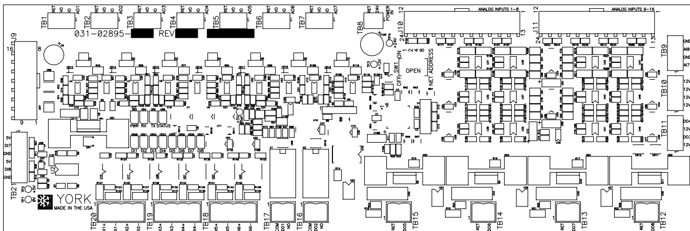
FIGURE 83 - I/O BOARD (031-02895-XXX)
