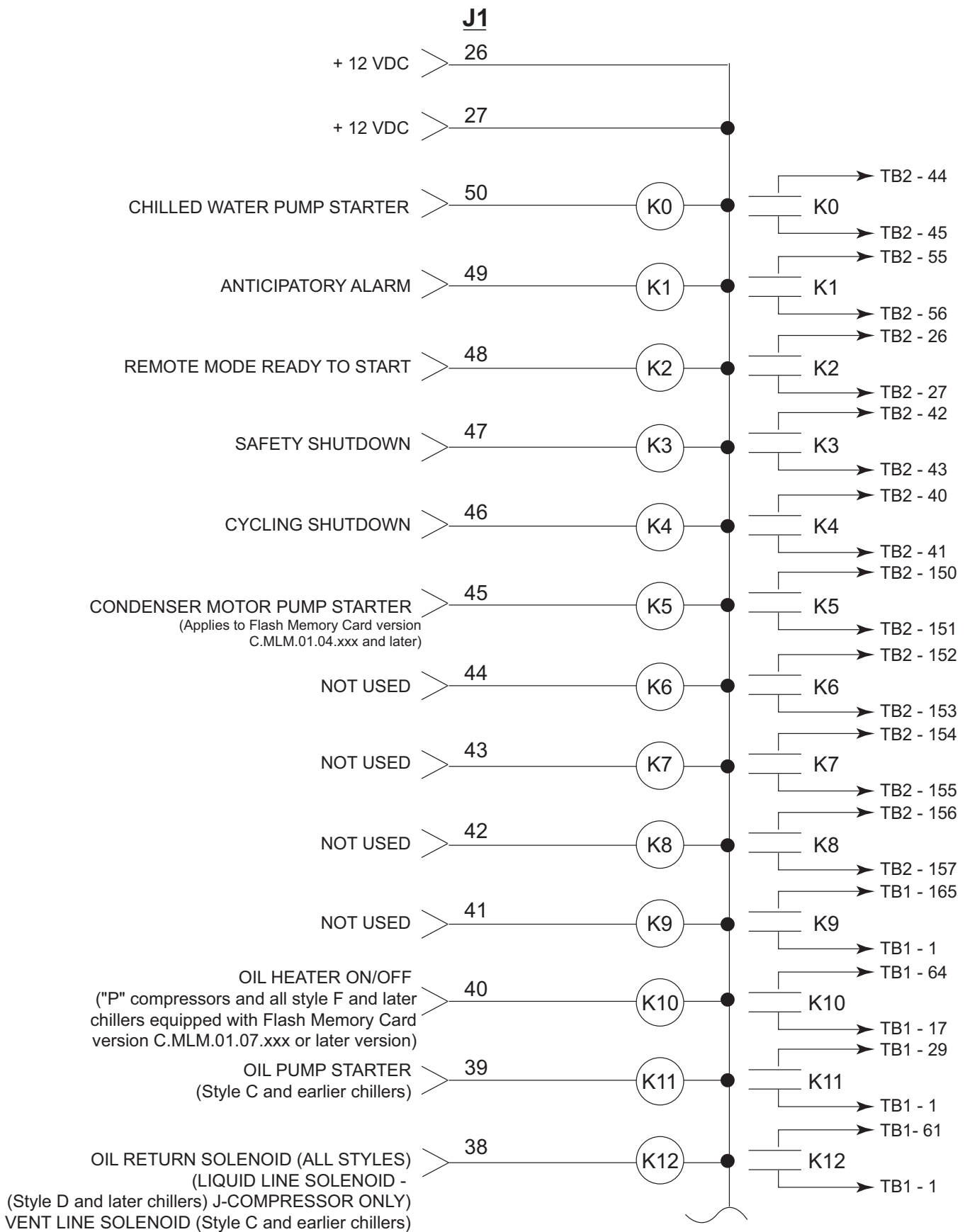
FIGURE 29 - J1 I/O BOARD DIGITAL OUTPUTS
