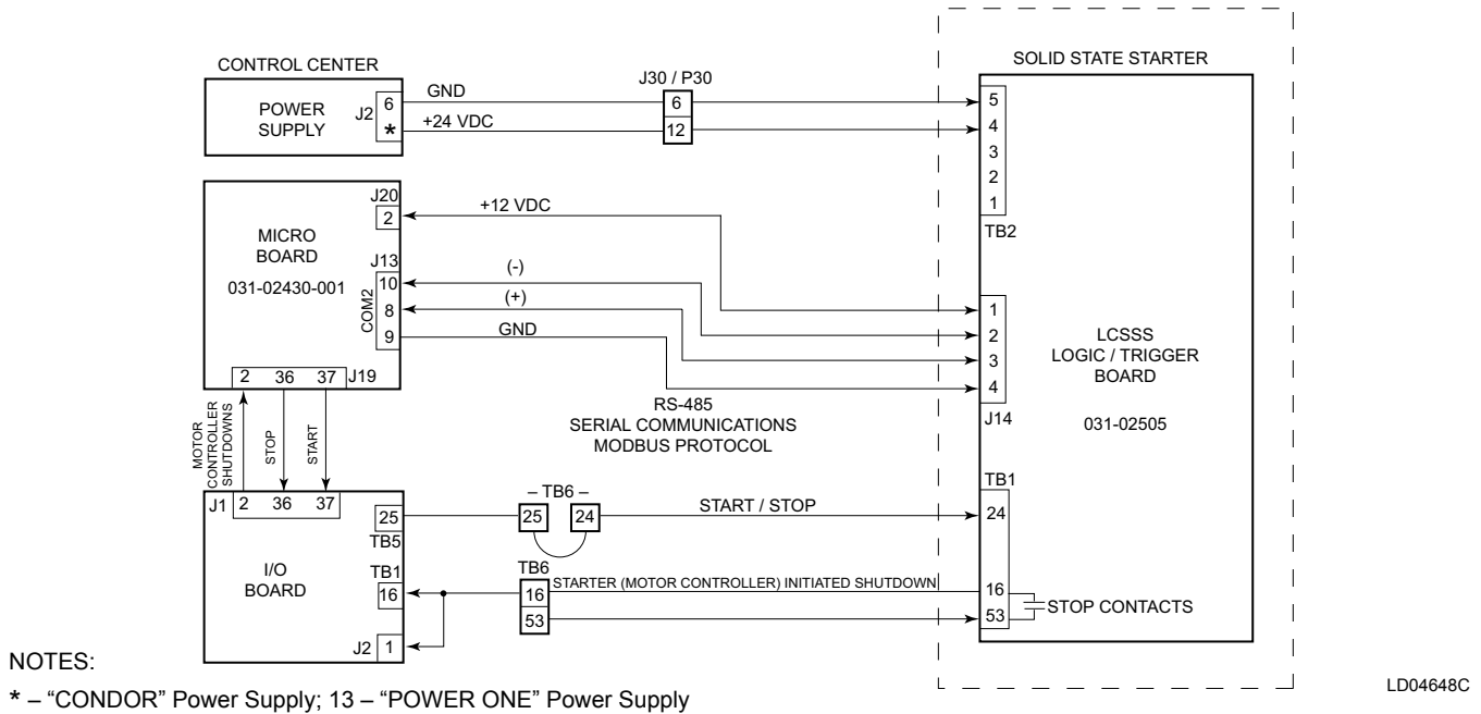
FIGURE 50 - STYLE B LIQUID COOLED SOLID STATE STARTER (LCSSS) – INTERFACE (MODBUS PROTOCOL)
