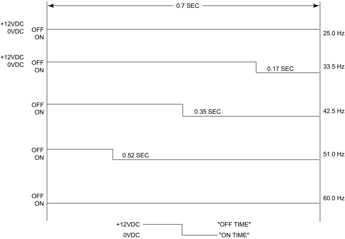
FIGURE 68 - OIL PUMP VSD SPEED CONTROL SIGNAL
