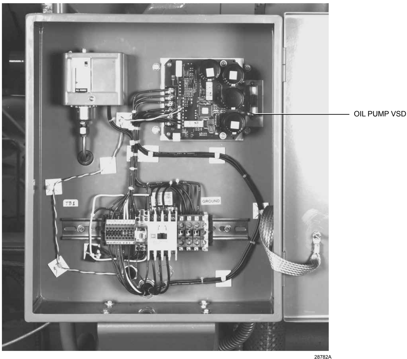
FIGURE 66 - OIL PUMP VARIABLE SPEED DRIVE (VSD)
