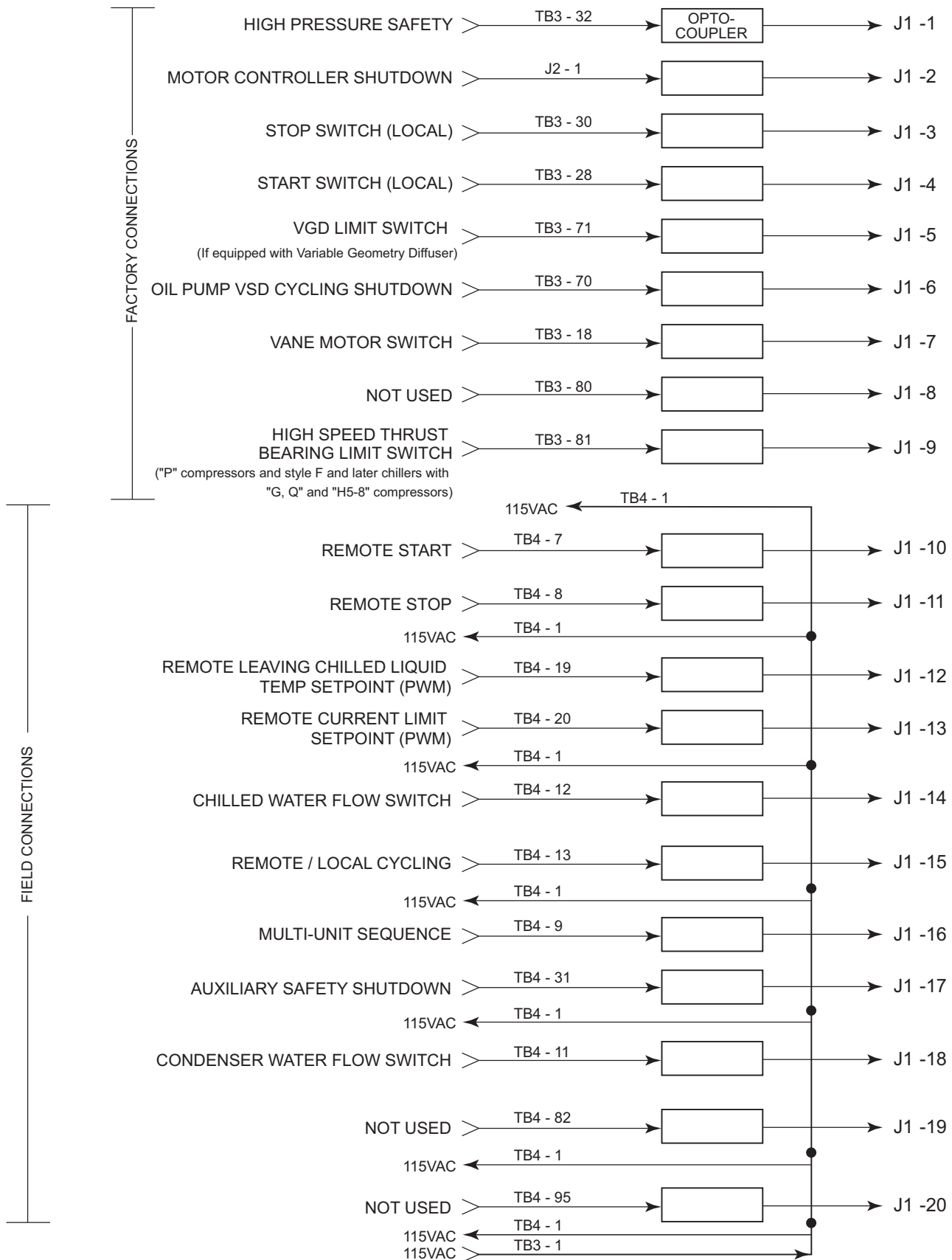
FIGURE 26 - I/O BOARD DIGITAL INPUTS
