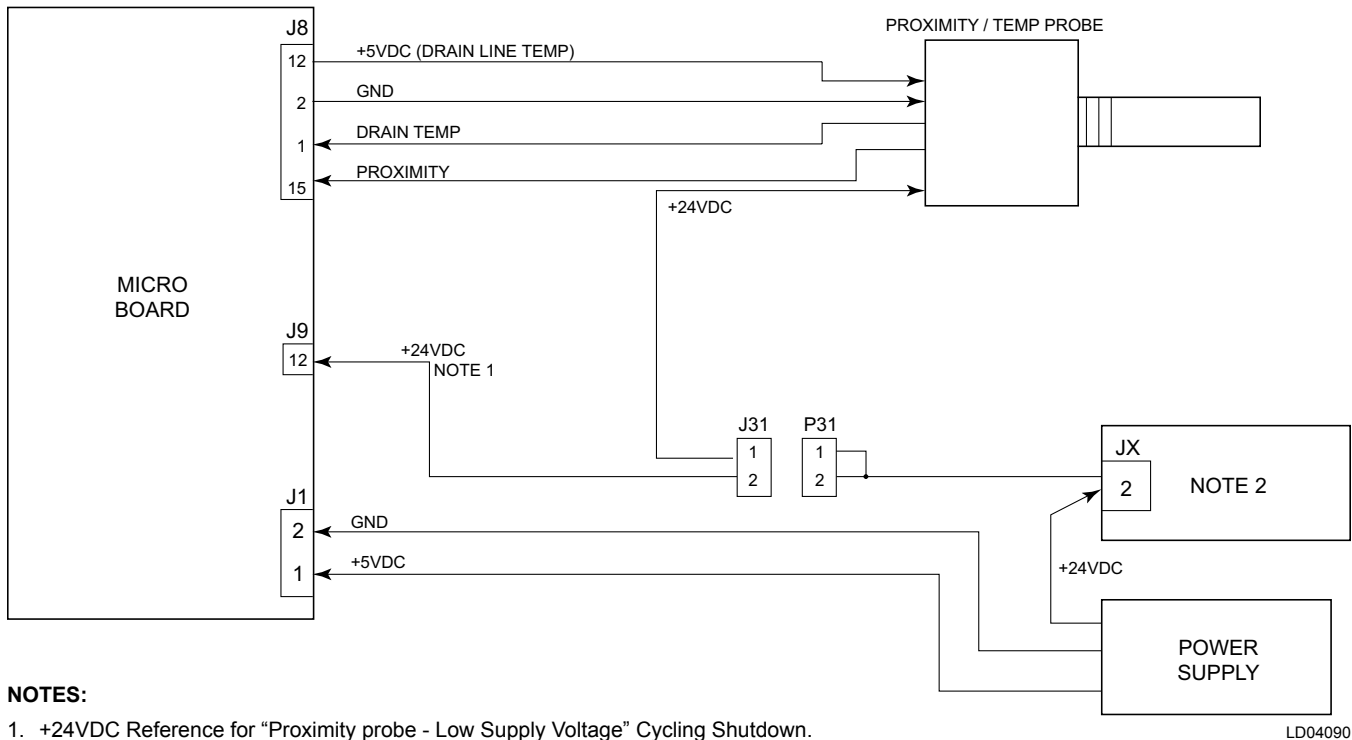
FIGURE 58 - PROXIMITY PROBE INTERFACE – PROBE PART NUMBER 025-30961-000
