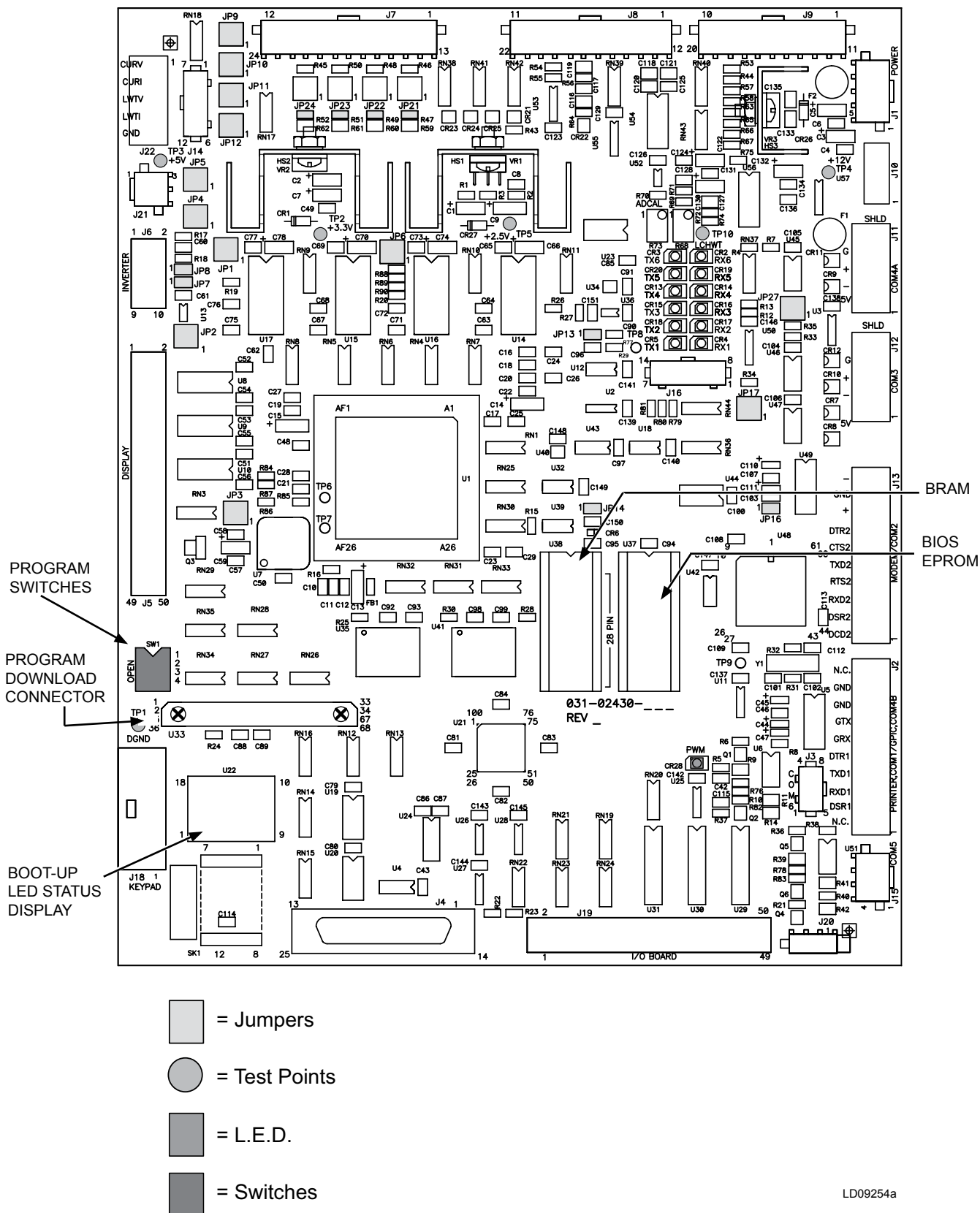
FIGURE 17 - MICROBOARD 031-02430-000 AND 031-02430-001
