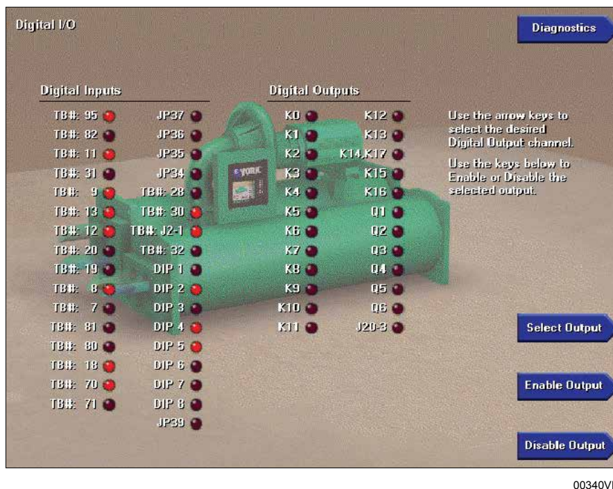
FIGURE 107 - DIGITAL INPUTS / OUTPUTS TEST SCREEN
