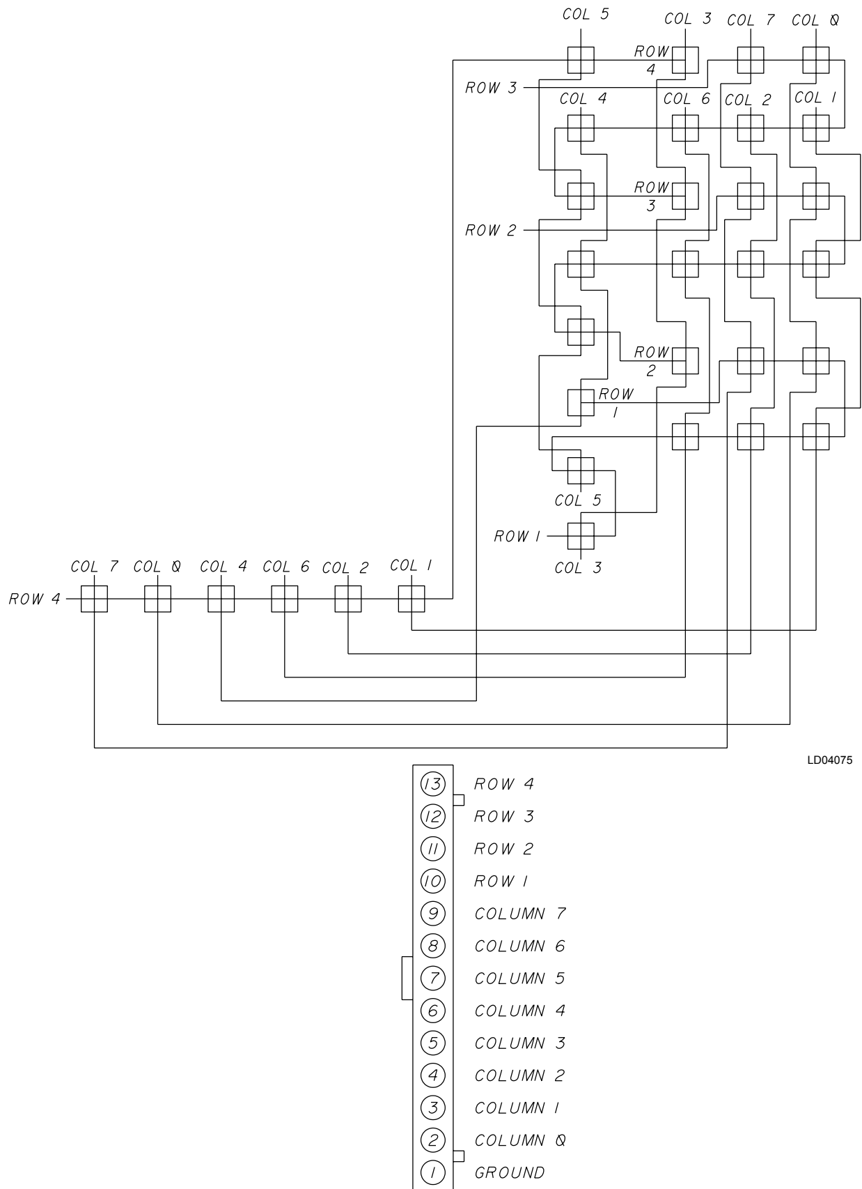
FIGURE 42 - KEYPAD
