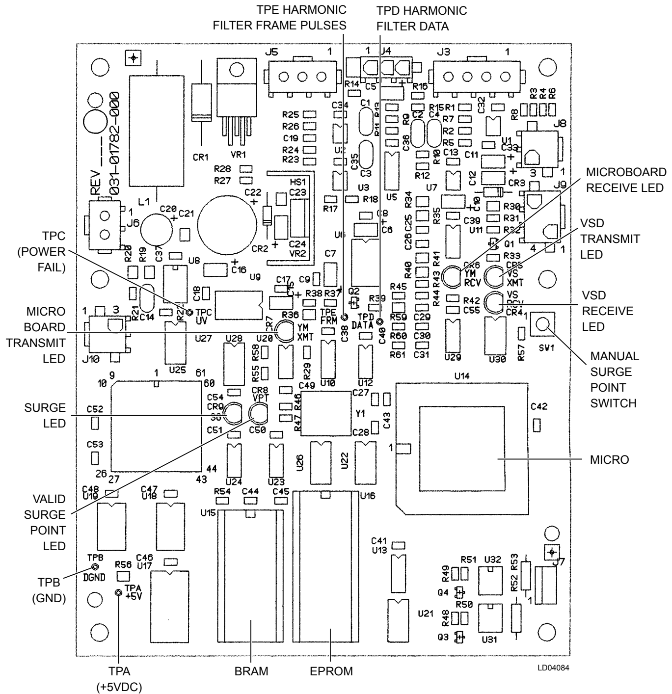
FIGURE 53 - COMPRESSOR MOTOR VARIABLE SPEED DRIVE (VSD) ADAPTIVE CAPACITY CONTROL (ACC) BOARD
