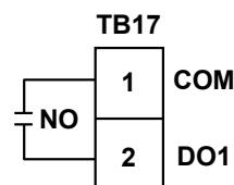
FIGURE 78 - RELAY OUTPUTS
