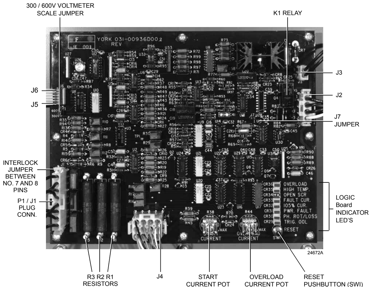
FIGURE 51 - SOLID STATE STARTER LOGIC BOARD
