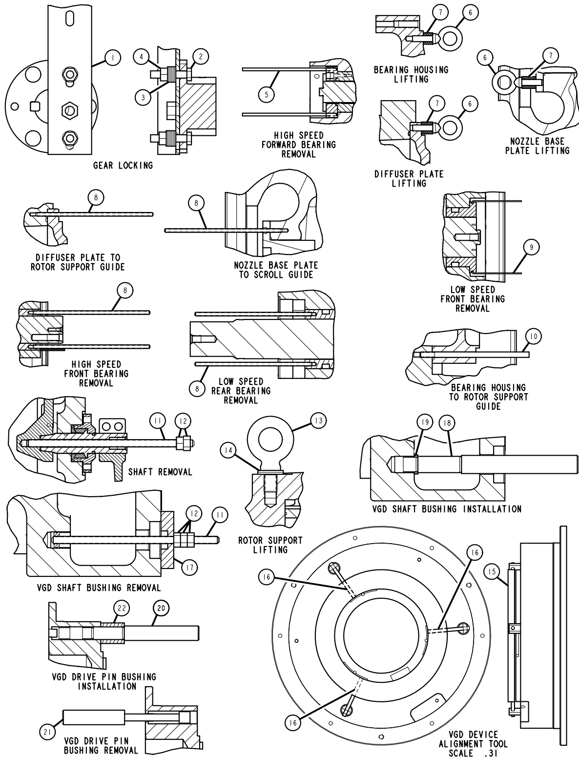
FIG. 1 – COMPRESSOR TOOL KIT (P7 W/ VGD)
