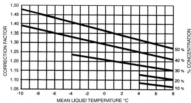
FIGURE 8 - PRESSURE DROP CORRECTION FACTORS FOR ETHYLENE GLYCOL SOLUTIONS
