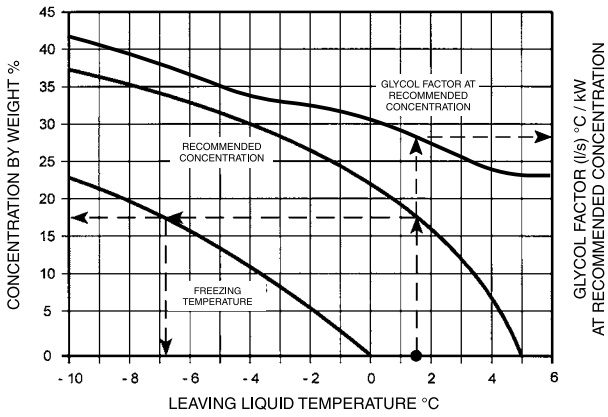
FIGURE 4 - RECOMMENDED CONCENTRATIONS FOR ETHYLENE GLYCOL SOLUTIONS
