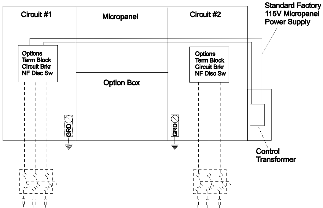
FIGURE 10 - MULTIPOINT POWER SUPPLY CONNECTION - STANDARD UNIT
