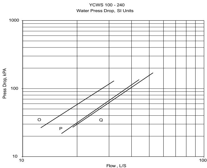
FIGURE 2 - COOLER WATER PRESSURE DROP CURVES (SI)
