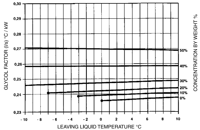
FIGURE 7 - FACTORS AT OTHER CONCENTRATIONS FOR PROPYLENE GLYCOL SOLUTIONS
