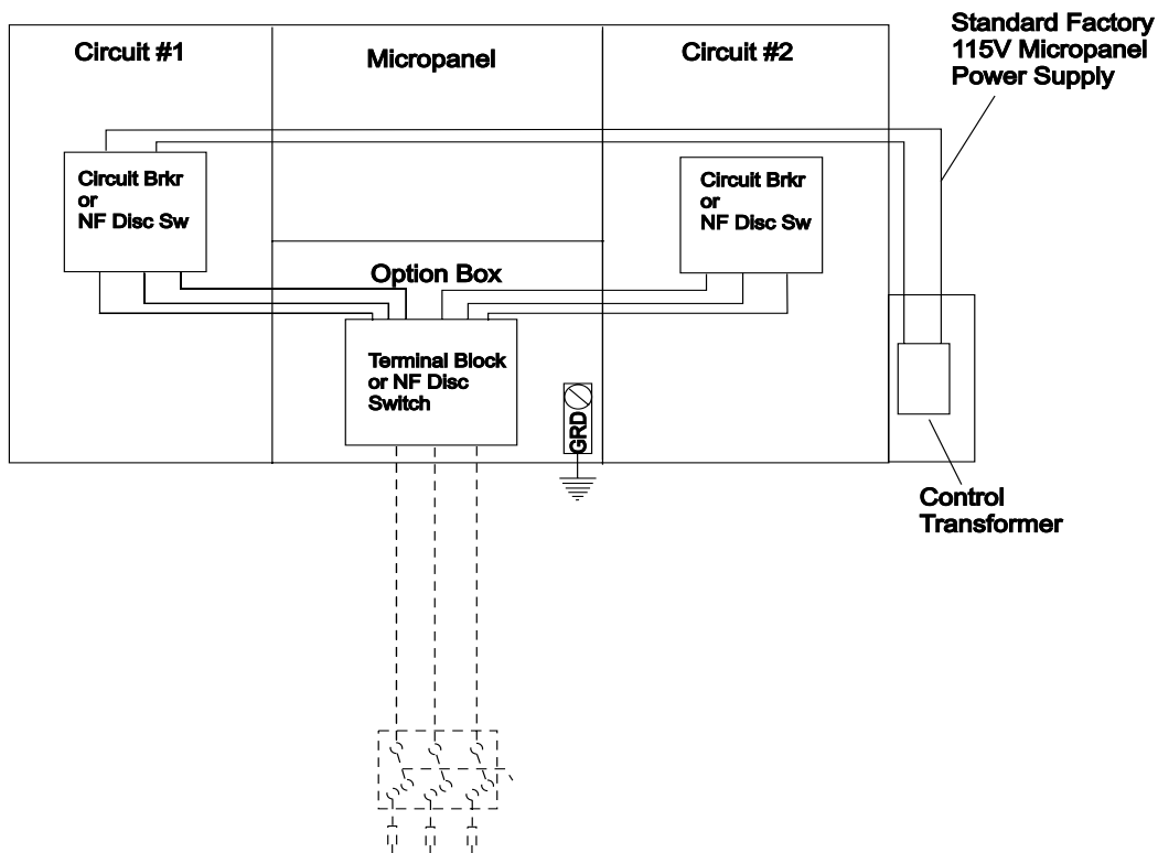
FIGURE 11 - SINGLE POINT POWER SUPPLY WITH INTERNAL CIRCUIT BREAKER OR NON-FUSED DISCONNECT SWITCH
