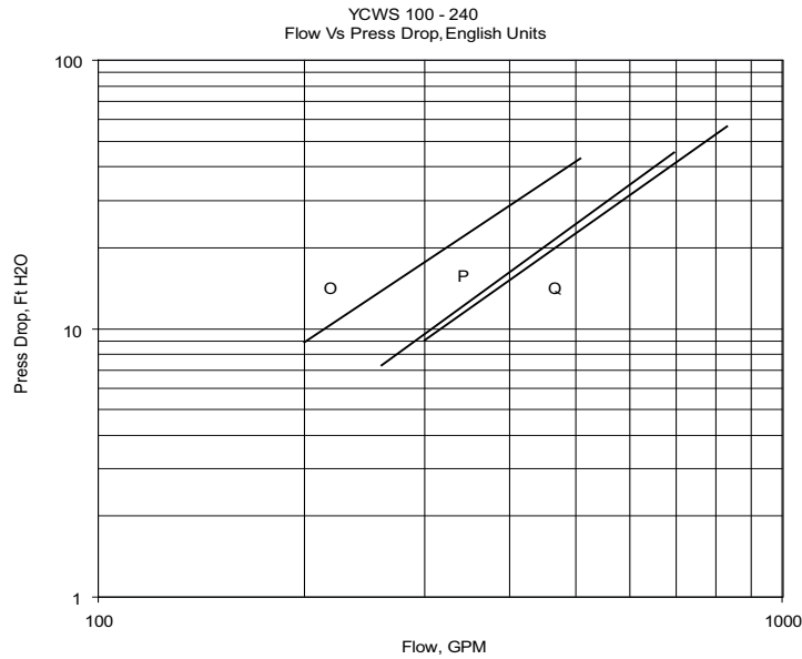
FIGURE 1 - COOLER WATER PRESSURE DROP CURVES (ENGLISH)
