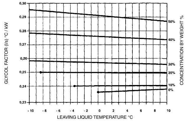
FIGURE 5 - FACTORS AT OTHER CONCENTRATIONS FOR ETHYLENE GLYCOL SOLUTIONS
