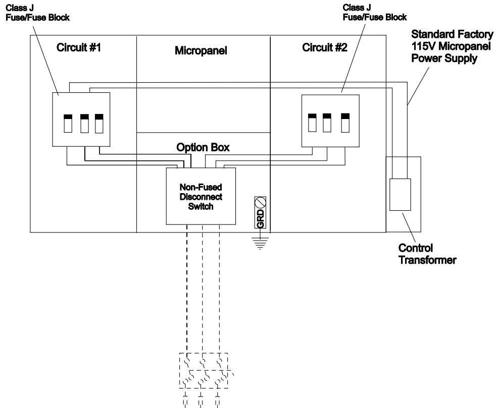
FIGURE 12 - OPTIONAL SINGLE POINT POWER SUPPLY WITH INTERNAL CLASS J FUSES/BLOCK
