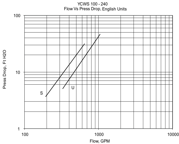
FIGURE 2 - CONDENSER WATER PRESSURE DROP CURVES (ENGLISH)
