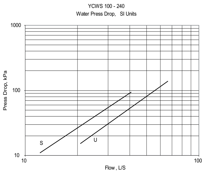
FIGURE 3 - CONDENSER WATER PRESSURE DROP CURVES (SI)
