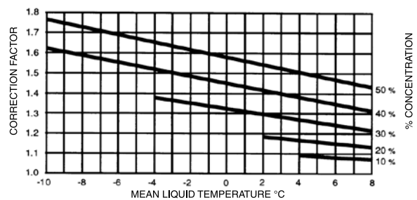
FIGURE 9 - PRESSURE DROP CORRECTION FACTORS FOR PROPYLENE GLYCOL SOLUTIONS
