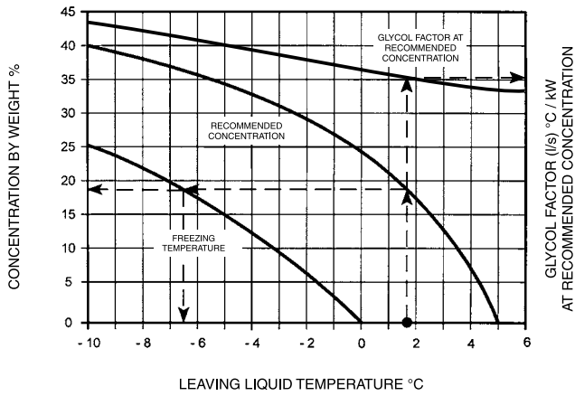
FIGURE 6 - RECOMMENDED CONCENTRATIONS FOR PROPYLENE GLYCOL SOLUTIONS
