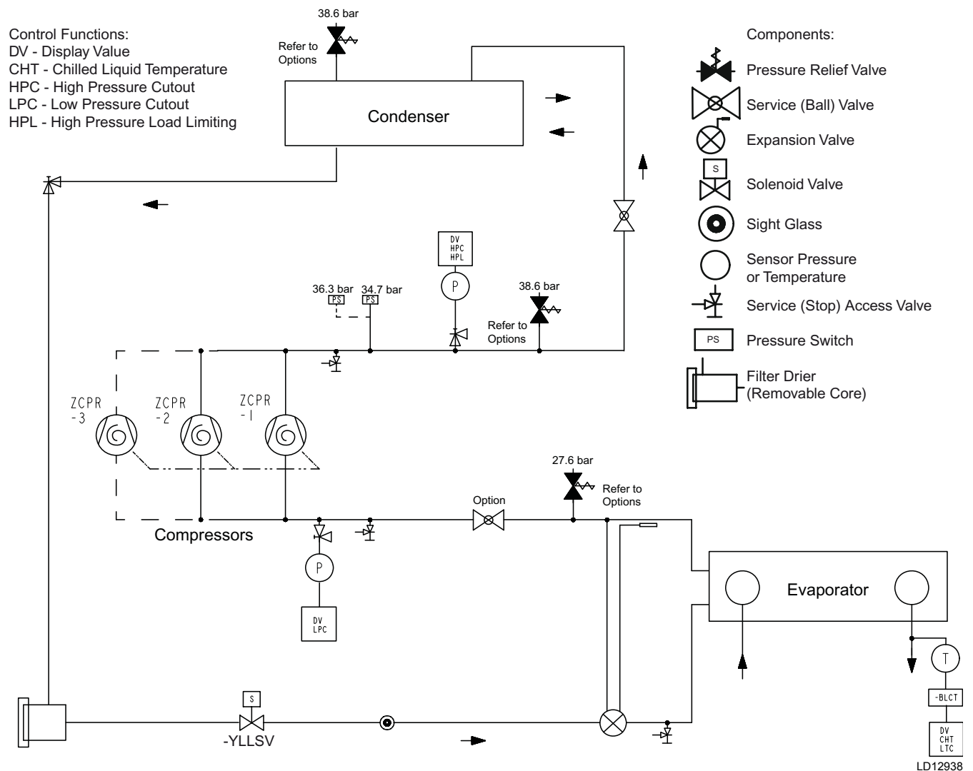
FIGURE 7 - PROCESS AND INSTRUMENTATION DIAGRAM
