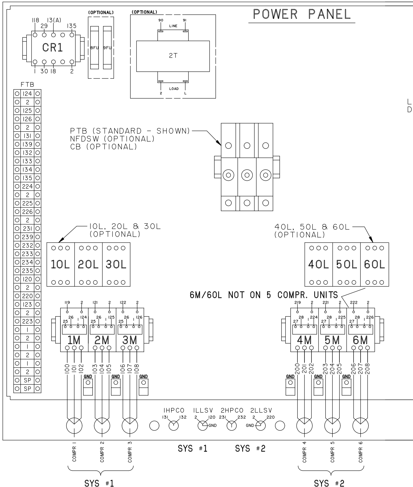
FIGURE 31 - CONNECTION WIRING DIAGRAM, 6 COMPRESSOR
