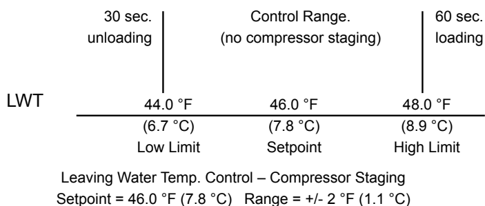
FIGURE 36 - LEAVING WATER TEMPERATURE CONTROL EXAMPLE
