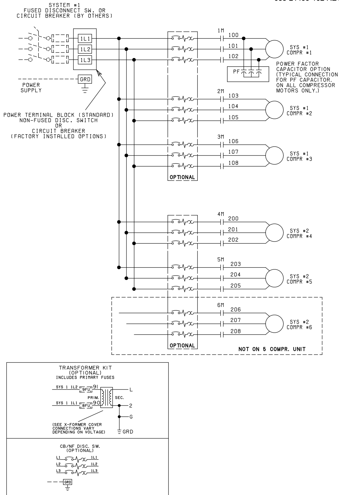
FIGURE 26 - POWER CIRCUIT, 5 AND 6 COMPRESSOR
