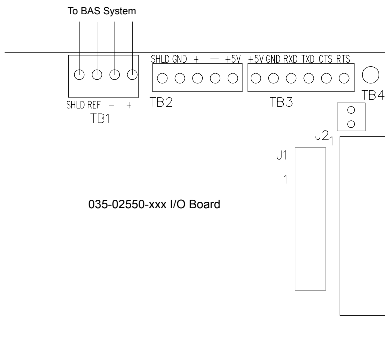
FIGURE 40 - MICRO PANEL CONNECTIONS
