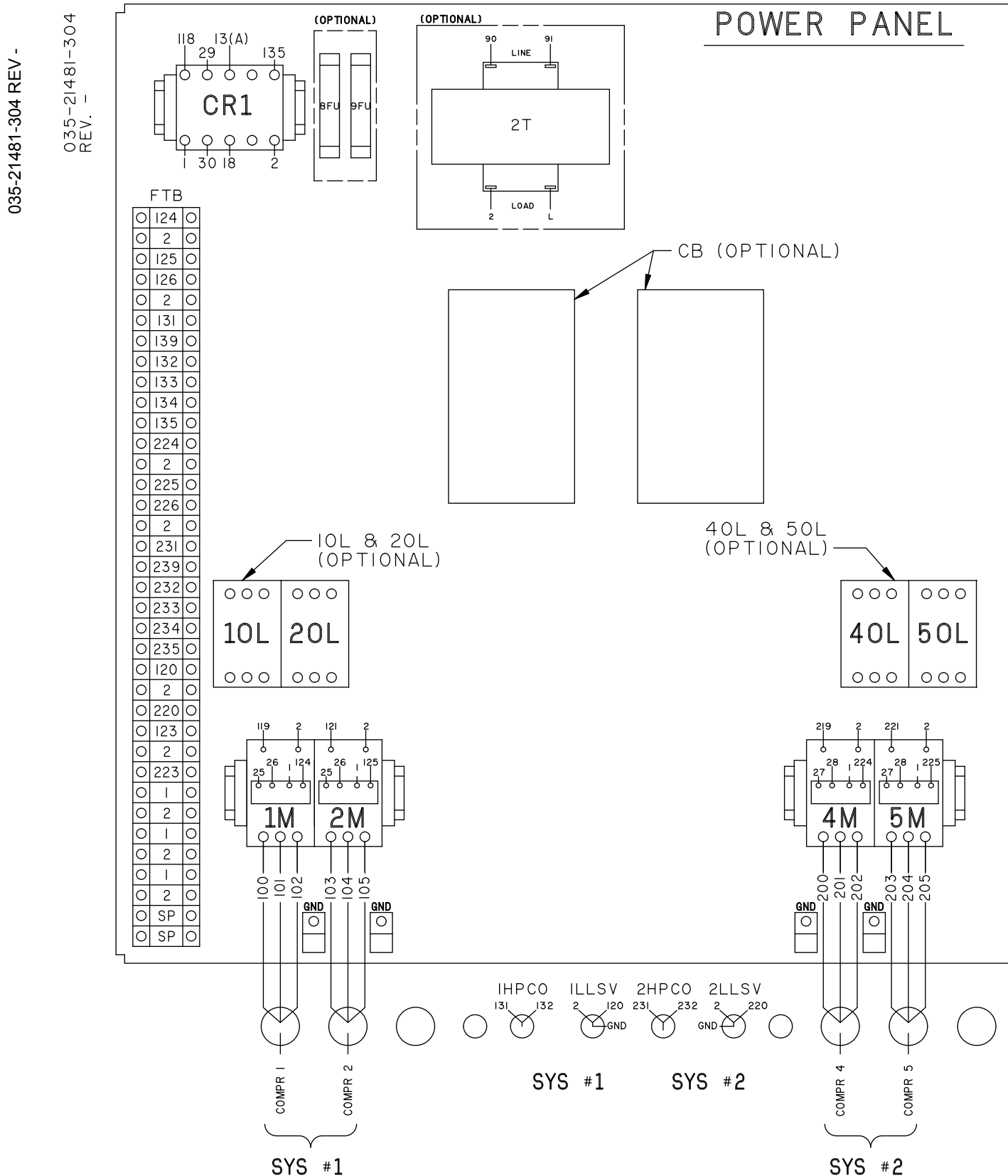
FIGURE 29 - CONNECTION WIRING DIAGRAM, 4 COMPRESSOR
