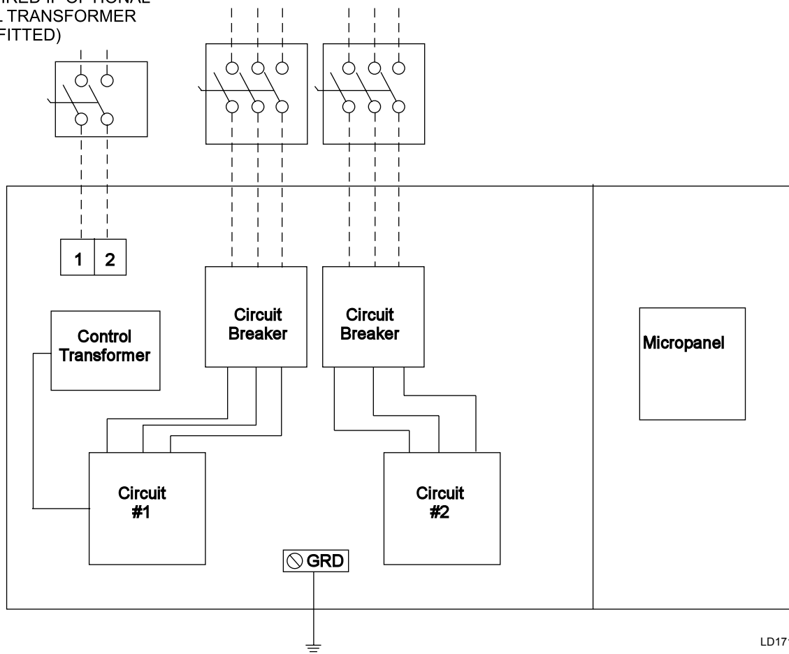
FIGURE 21 - DUAL POINT POWER SUPPLY CONNECTION – STANDARD UNIT
