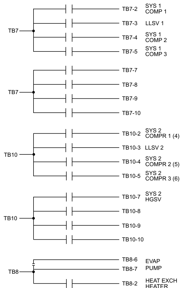
FIGURE 39 - I/O BOARD RELAY CONTACT ARCHITECTURE
