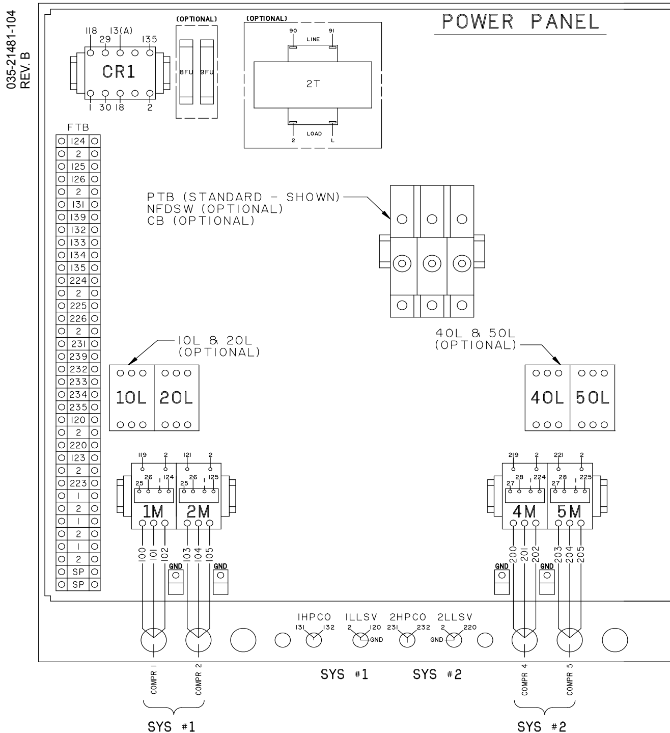
FIGURE 28 - CONNECTION WIRING DIAGRAM, 4 COMPRESSOR
