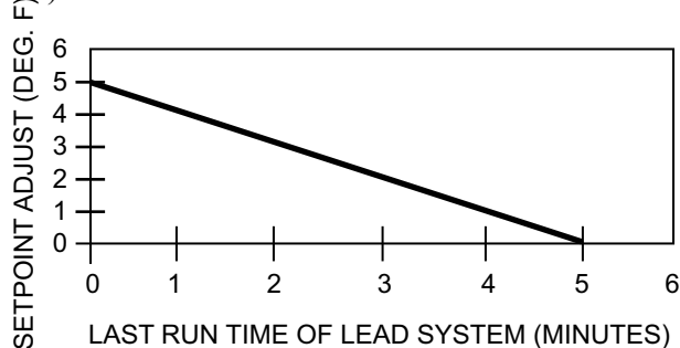
FIGURE 37 - SETPOINT ADJUST
