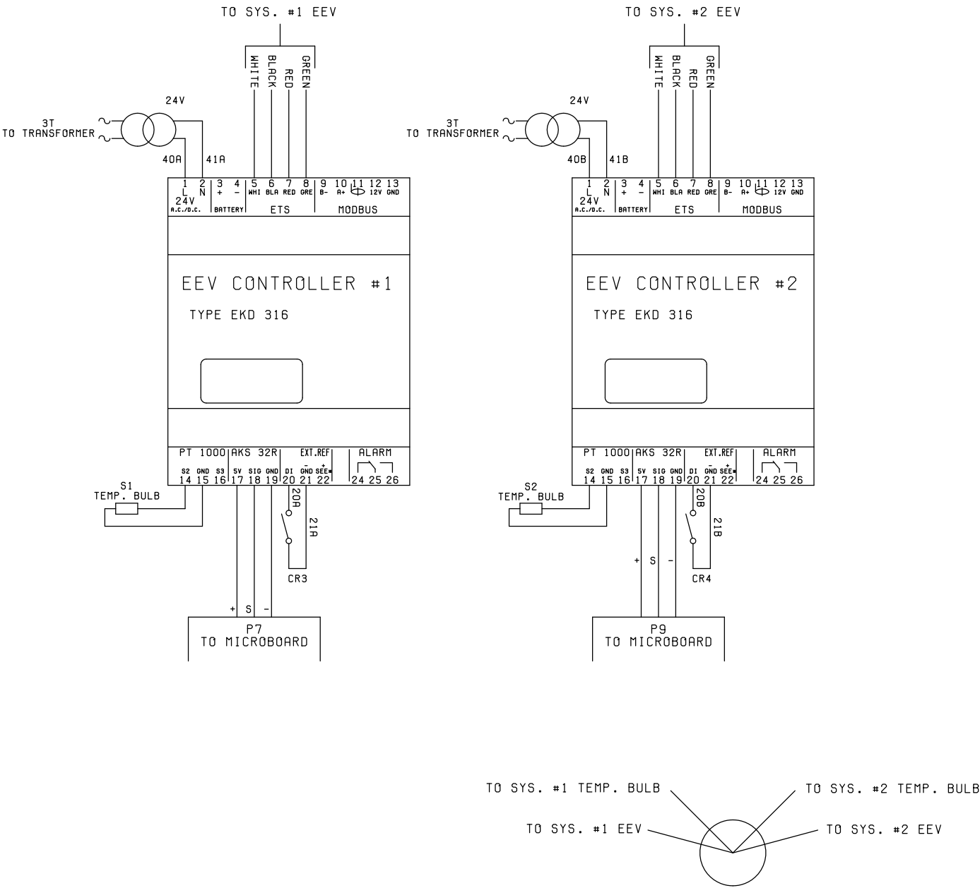
FIGURE 34 - ELEMENTARY WIRING DIAGRAM, EEV CONTROLLER, 4 AND 6 COMPRESSOR
