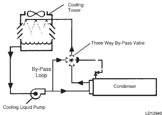
FIGURE 10 - DIRECT PRESSURE CONTROL DIAGRAM
