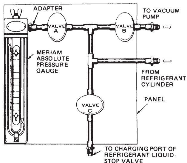
FIG. 7 – TYPICAL ABSOLUTE PRESSURE GAUGE AND CHARGING PANEL
