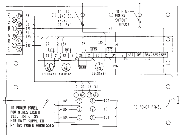
8 CYL. "J" COMPRESSOR TERMINAL BOX SYSTEM NO. 1 (UNIT WITH STANDARD UNLOADING)
