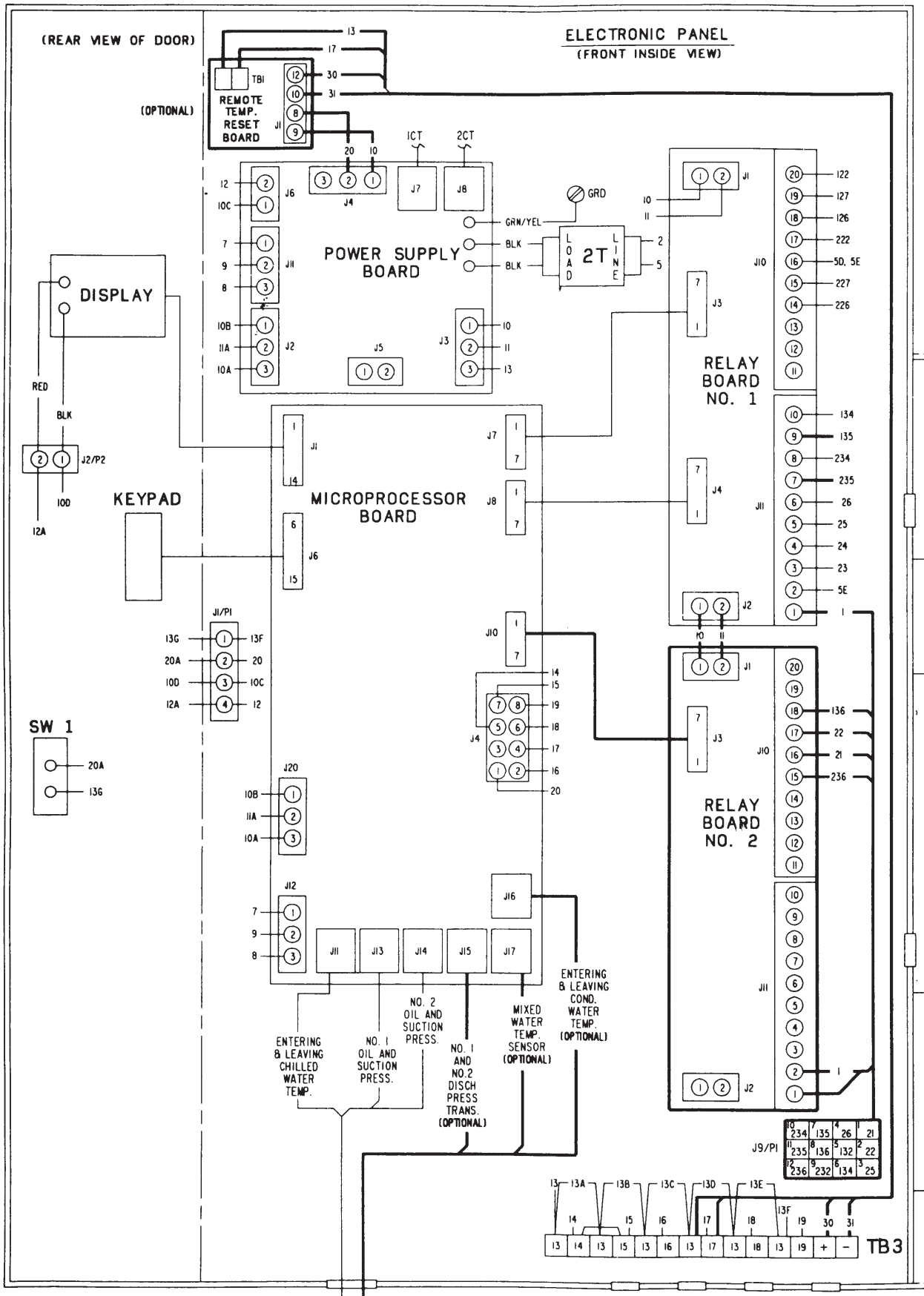
FIG. 10 – CONNECTION DIAGRAM
