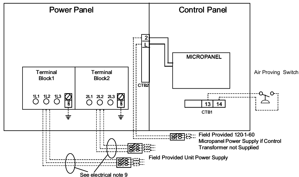
Figure 2: Multiple Point Power Supply Connection – Terminal Block (YCUL0046-0090)
