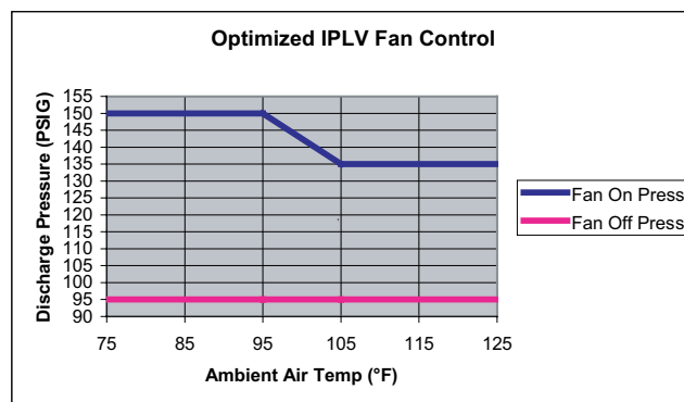
FIGURE 59 - HIGH IPLV FAN CONTROL
