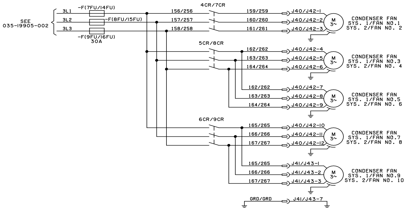
5 CONDENSER FAN ARRANGEMENT
