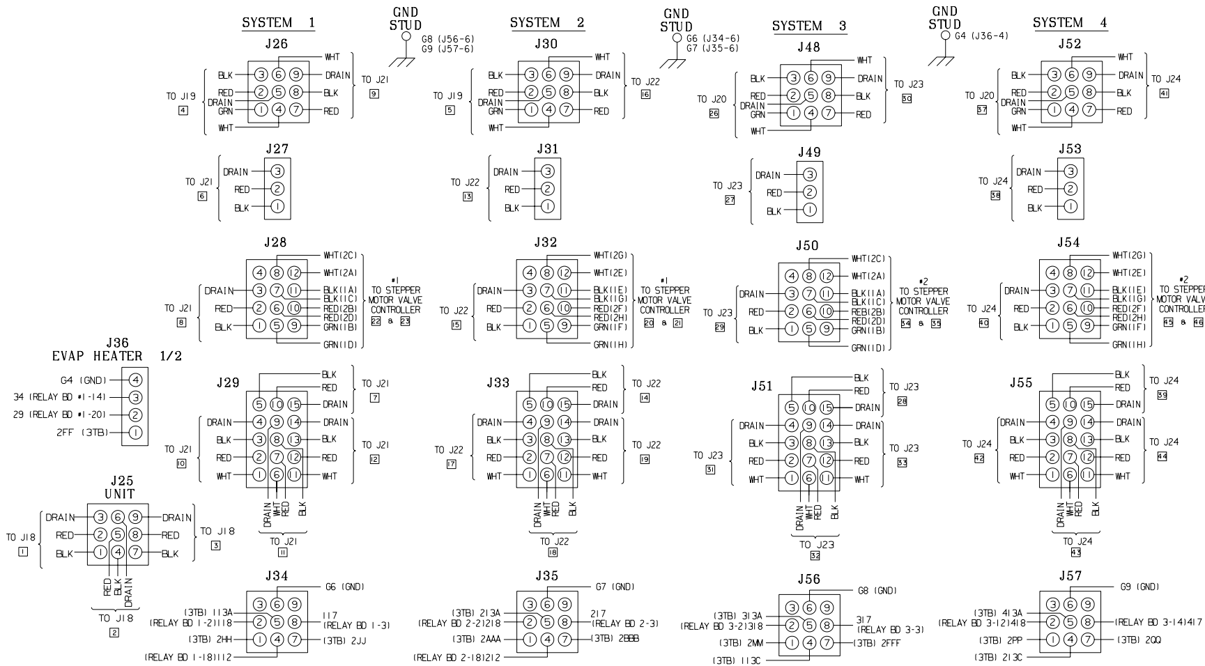
CONTROL WIRING - CONNECTION DIAGRAM 4 COMPRESSOR YCAV CHILLER 035-20890-005 REV. B
