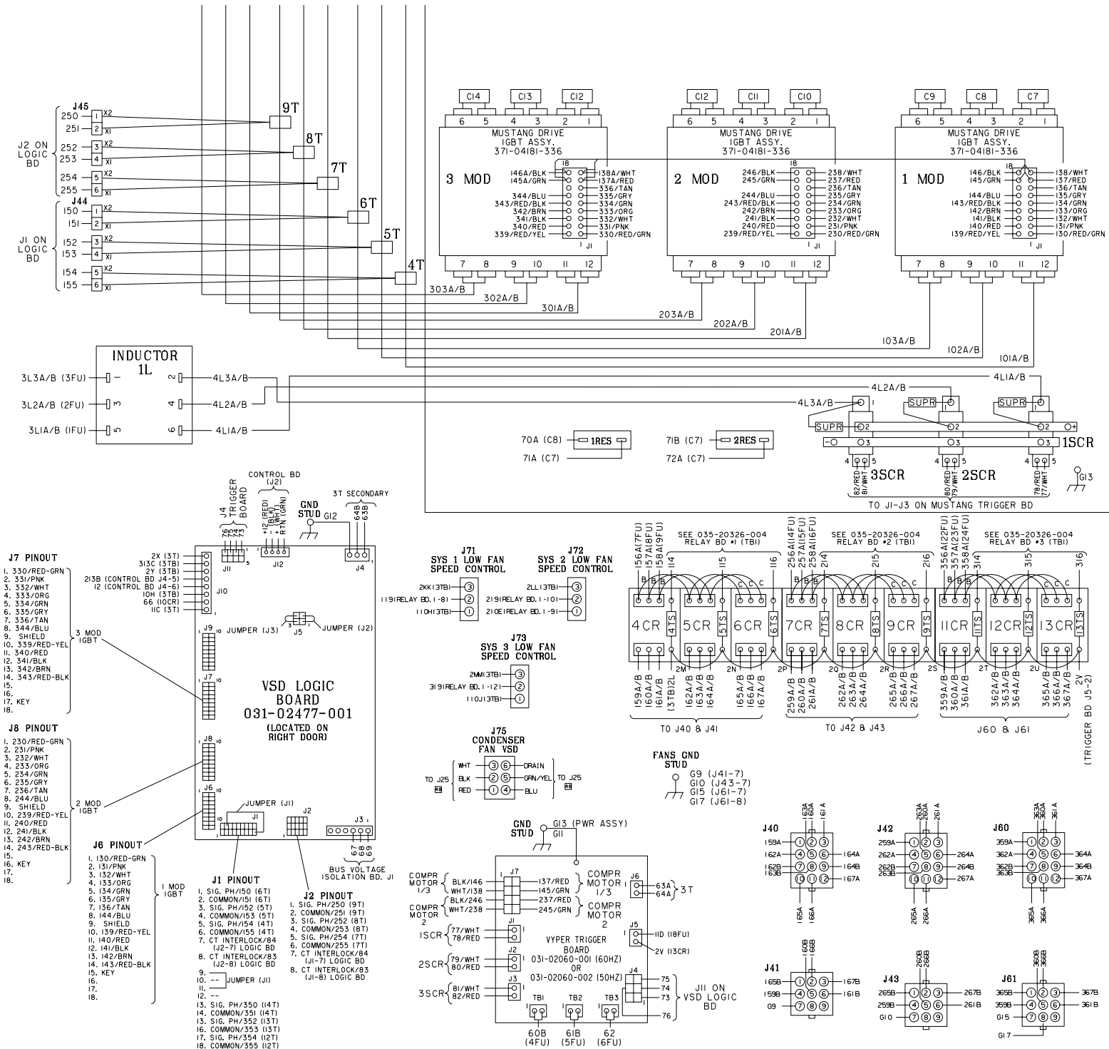
POWER WIRING - CONNECTION DIAGRAM 3 COMPRESSOR YCAV CHILLER 035-20326-005 REV. D
