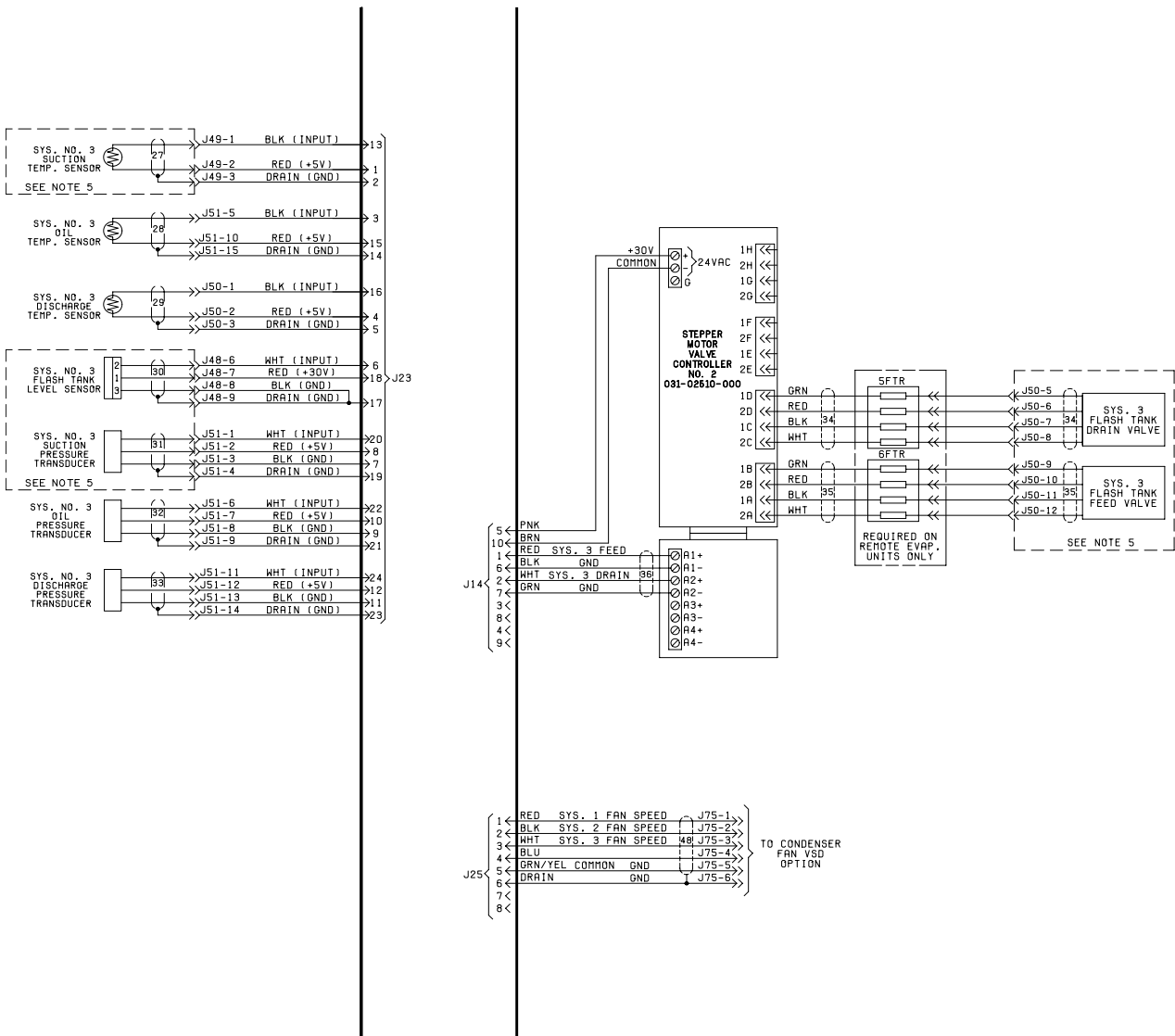
CONTROL ELEMENTARY DIAGRAM 3 COMPRESSOR YCAV CHILLER 035-20326-002 REV. D
