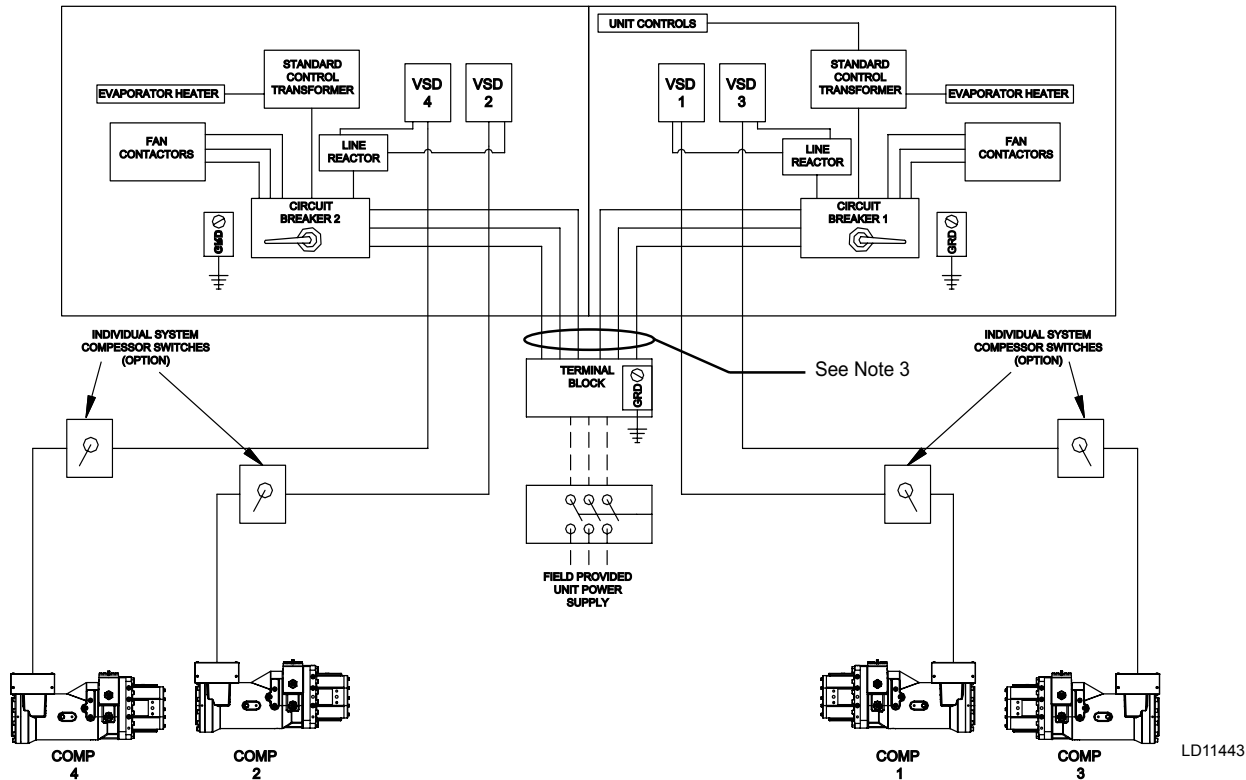
FIG. 3 - SINGLE-POINT POWER SUPPLY CONNECTION WITH CIRCUIT BREAKER PROTECTION
