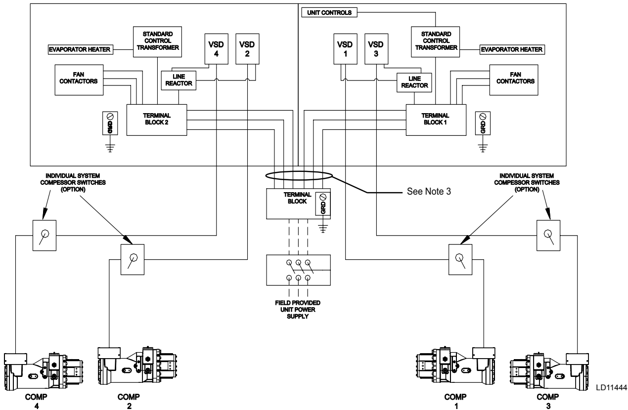
FIG. 4 - SINGLE-POINT POWER SUPPLY CONNECTION WITH TERMINAL BLOCK
