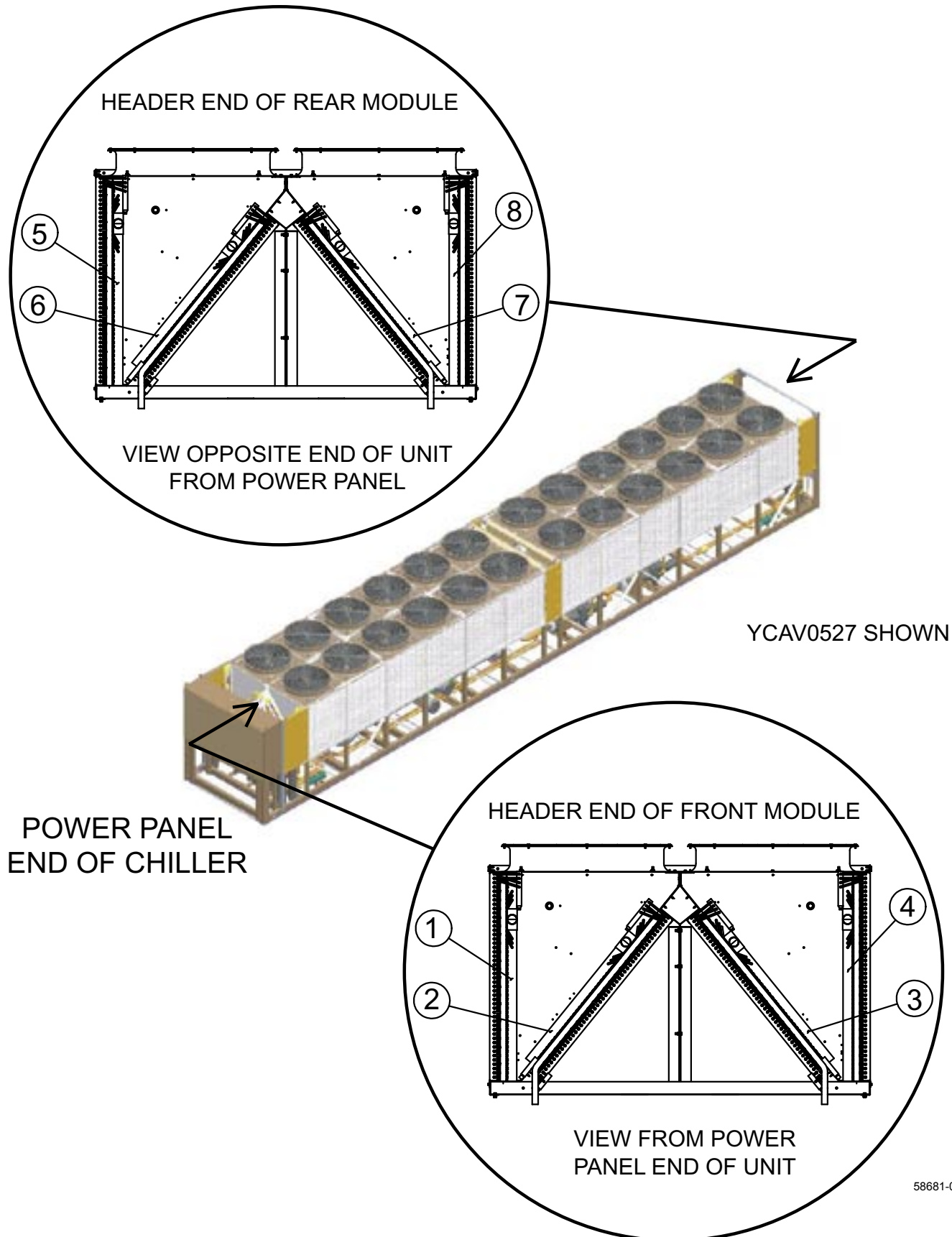
FIG. 2 – CONDENSER COIL COMPONENTS (REF. TABLES 2 AND 2A, PAGES 10 THRU 14)
