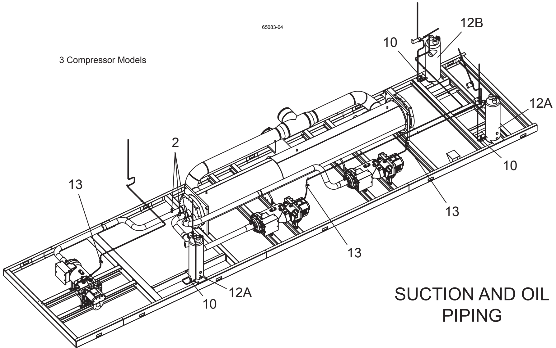
FIG. 4B – SUCTION AND OIL PIPING COMPONENTS - 3 COMPRESSOR MODELS (REF. TABLE 4, PAGES 20 AND 21)
