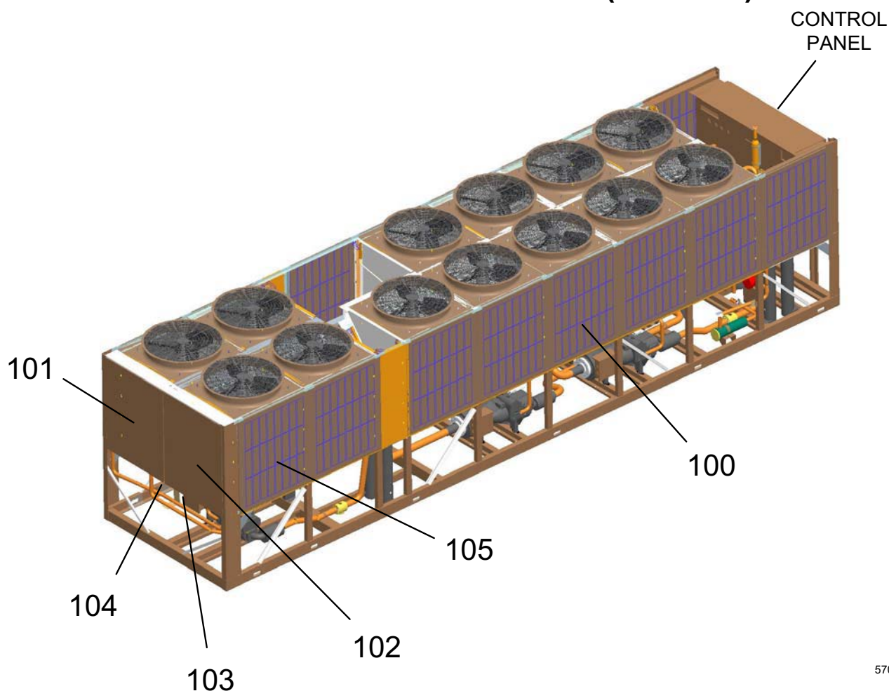
FIG. 17 – LOUVERED ENCLOSURE (TOP SECTIONS) - 375-57097-130 SHOWN (REF. TABLE 20)
