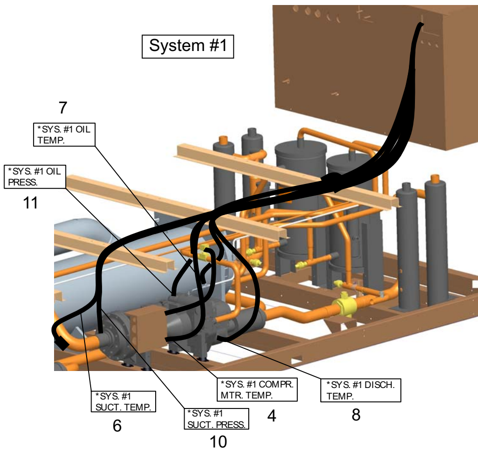
FIG. 12A – HARNESS LAYOUT (REF. TABLE 12, PAGES 61 - 65)
