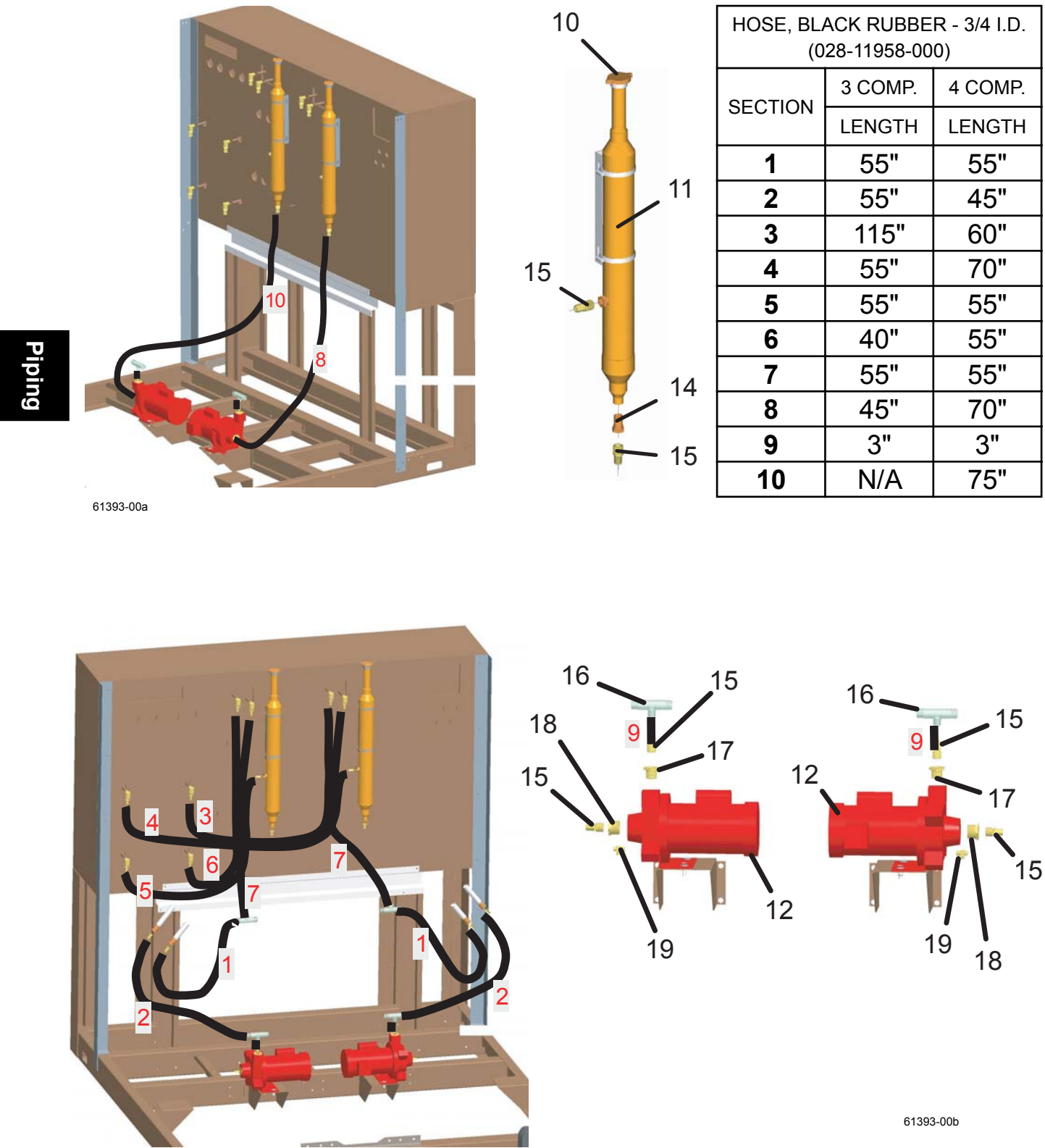
FIG. 4J – GLYCOL LOOP COMPONENTS (REF. TABLE 4C, PAGE 31)
