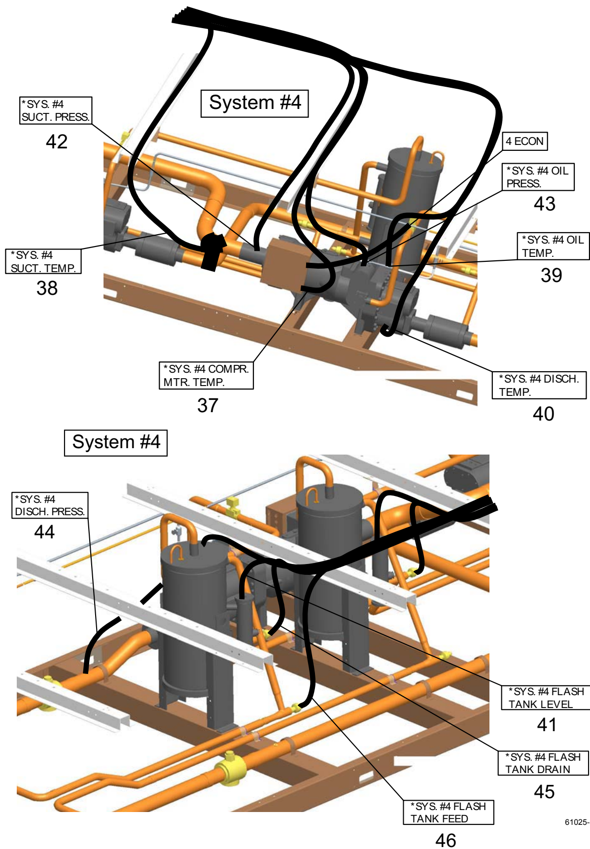
FIG. 12D – HARNESS LAYOUT (REF. TABLE 12, PAGES 61 - 65)
