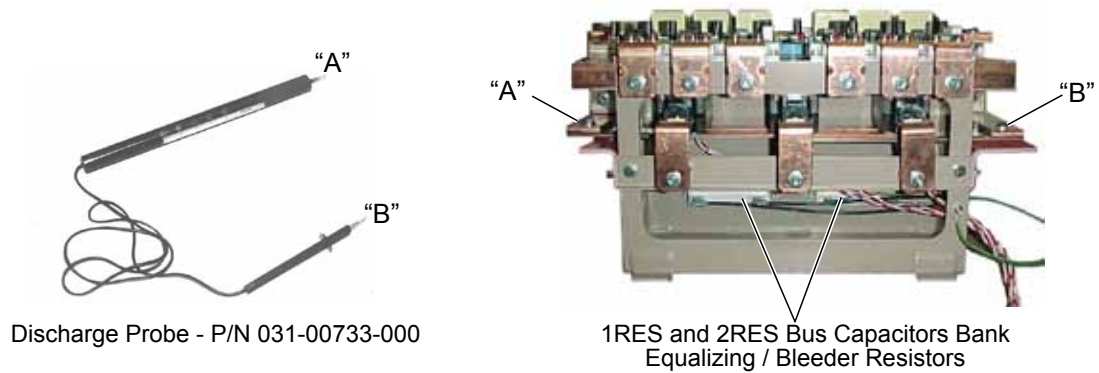
FIGURE 3 - DISCHARGE PROBE
