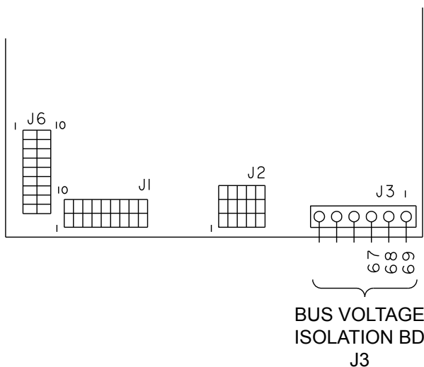
FIGURE 4 - VOLTAGE ISOLATION
